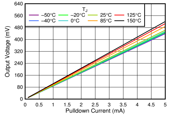
5-14. V_{OUT} vs I_{OUT} Pulldown Resistor
