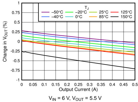
5-13. 5.5-V Load Regulation vs I_{OUT}
