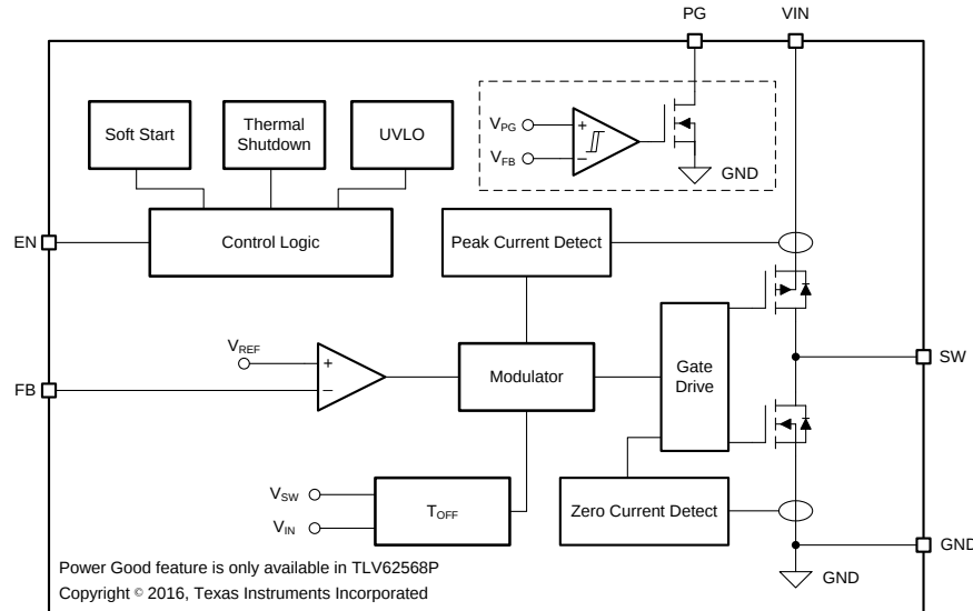
FIG 4. TLV62568 Functional Block Diagram
