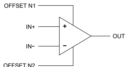
TL071 for PS Package (SO, 8) Only
