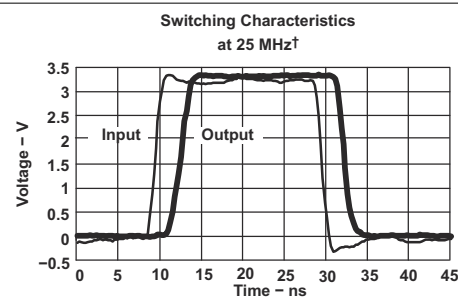
Figure 9-3. Excellent Signal Integrity
