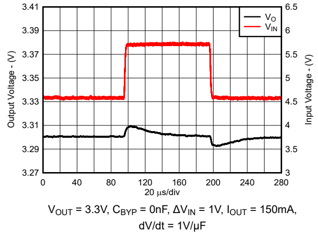
7-17. Line Transient Response (New Chip)
