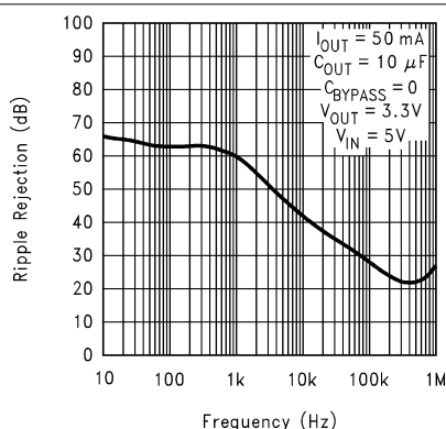
図 5-7. Ripple Rejection vs Frequency (Legacy Chip)
