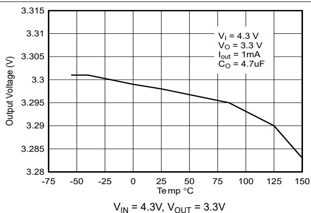
Figure 5-2. V_{OUT} vs Temperature (New Chip)
