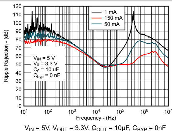
図 5-9. Ripple Rejection vs Frequency (New Chip)
