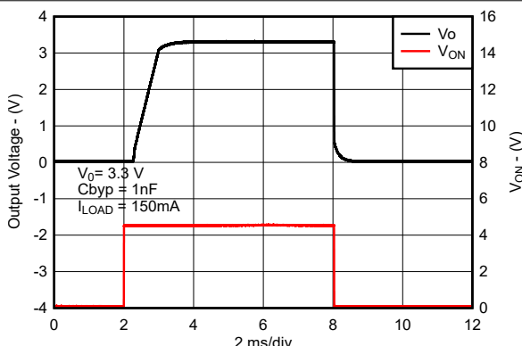
7-25. Turn-On Time (New Chip)
