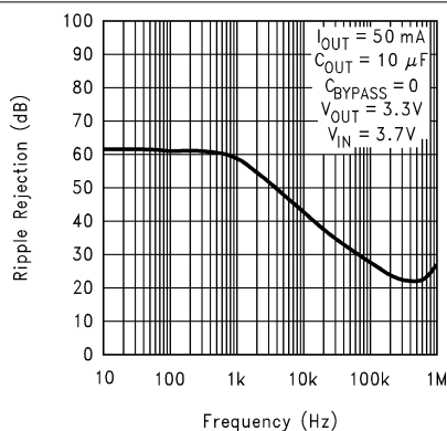
図 5-9. Ripple Rejection vs Frequency (New Chip)
