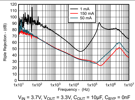
図 5-14. Ripple Rejection vs Frequency (New Chip)
