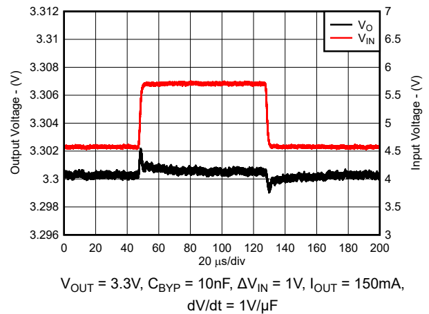
7-21. Line Transient Response (New Chip)
