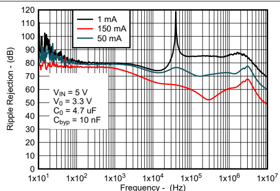
図 5-14. Ripple Rejection vs Frequency (New Chip)
