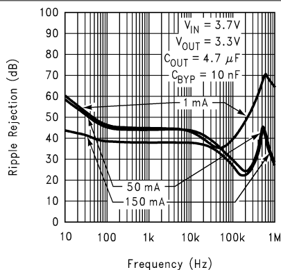
図 5-13. Ripple Rejection vs Frequency (Legacy Chip)
