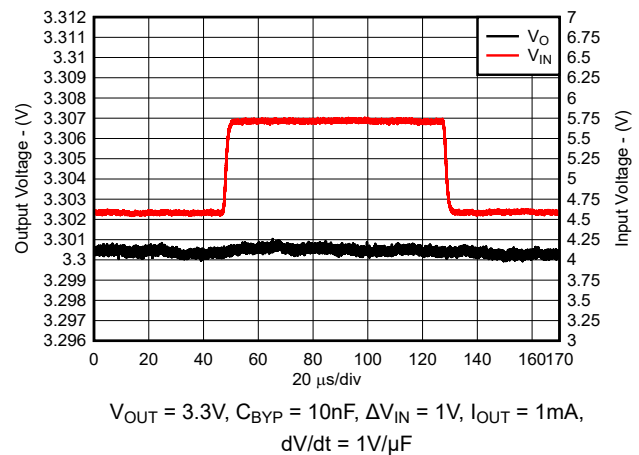
7-19. Line Transient Response (New Chip)
