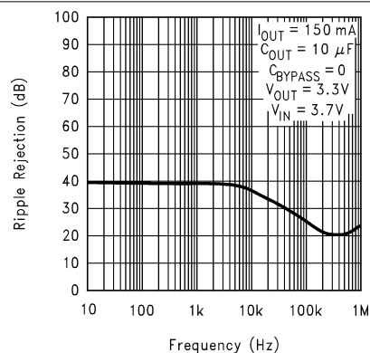
図 5-10. Ripple Rejection vs Frequency (Legacy Chip)
