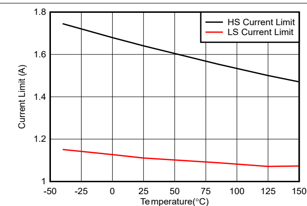
図 6-12. HS and LS Current Limit Versus Temperature
