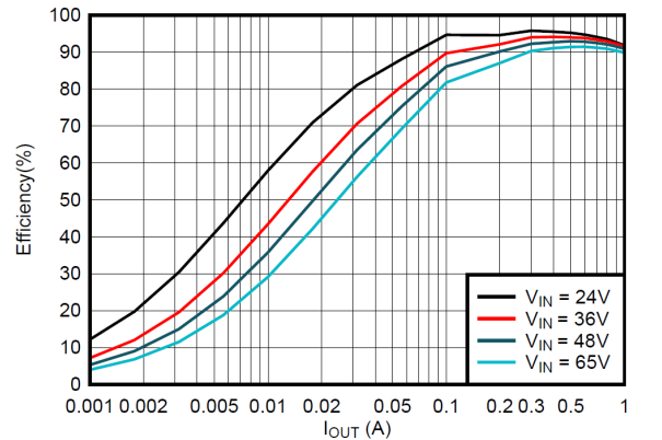
図 6-4. 5V FPWM Efficiency Versus Load Current
