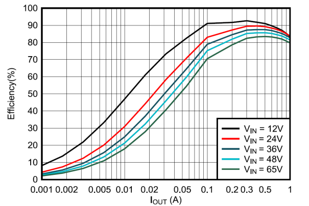
図 6-2. 3.3V FPWM Efficiency Versus Load Current
