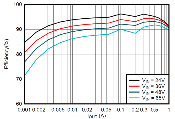
図 6-3. 5V PFM Efficiency Versus Load Current
