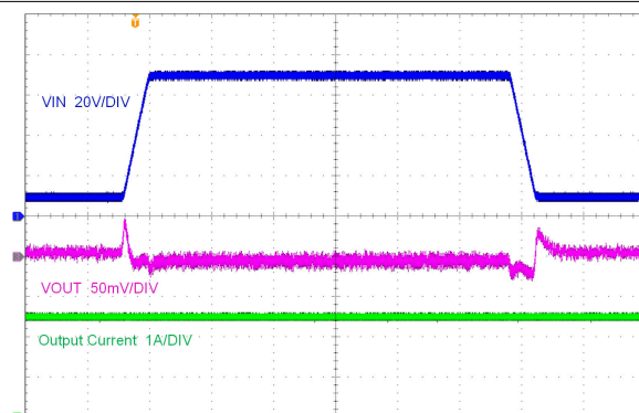
LMR38025(PFM) V_{OUT} = 5V 400kHz (AC 結合)
