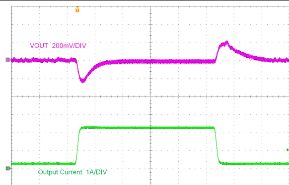
LMR38025(PFM) V_{OUT} = 5V 400kHz, 100 \mu s/DIV (AC 結合)
