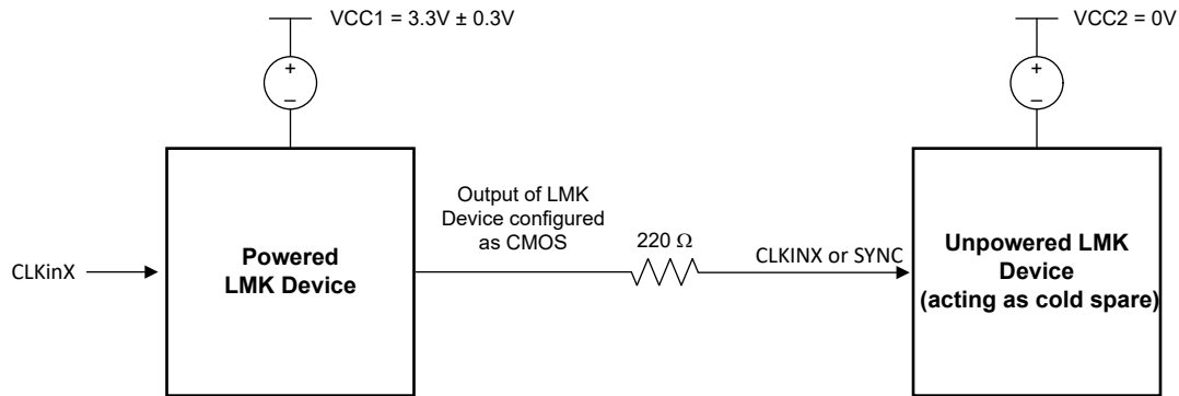
☒ 9-8. Cold Sparring Devices Setup
