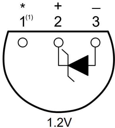
図 5-3. LP Package 3-Pin TO-92 Bottom View
