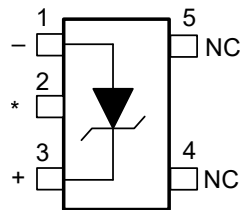
図 5-2. DCK Package 5-Pin SC70 Top View
