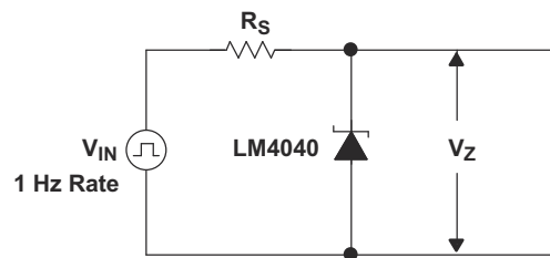
8-3. Test Circuit
