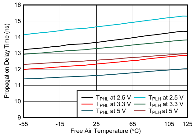
FIG 5-16. Propagation Delay Time vs Free-Air Temperature
