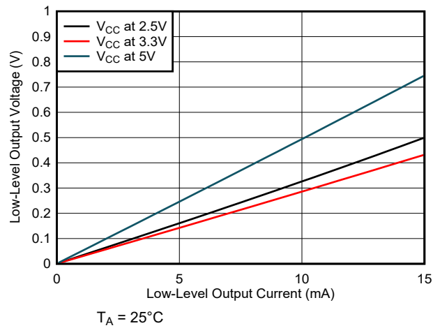
FIG 5-14. Low-Level Output Voltage vs Low-Level Output Current
