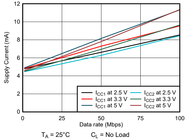
FIG 5-12. ISO7763 Supply Current vs Data Rate (With No Load)
