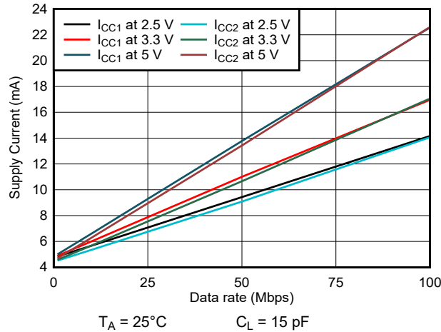
FIG 5-11. ISO7763 Supply Current vs Data Rate (With 15-pF Load)
