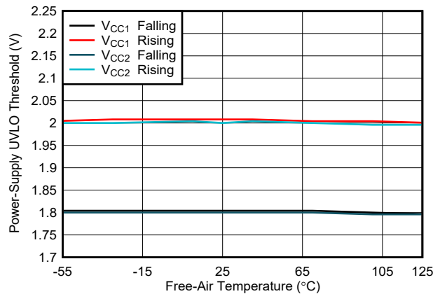
FIG 5-15. Power Supply Undervoltage Threshold vs Free-Air Temperature
