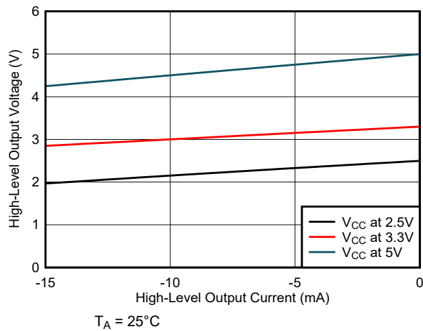
FIG 5-13. High-Level Output Voltage vs High-Level Output Current
