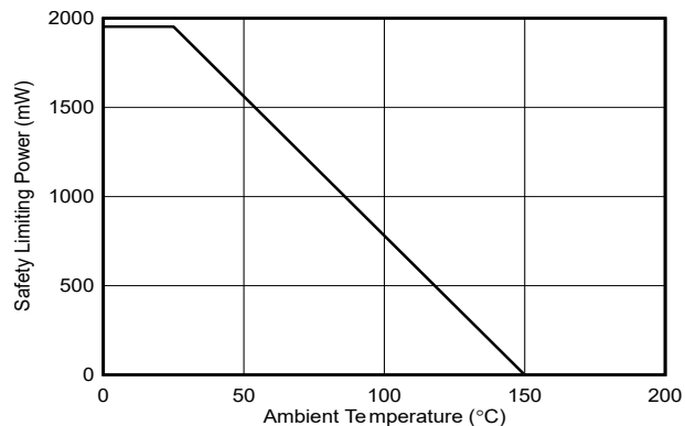
図 5-2. Thermal Derating Curve for Safety Limiting Power for DW-16 Package
