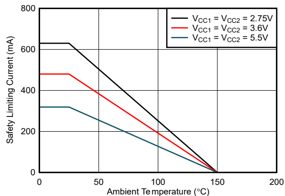
図 5-1. Thermal Derating Curve for Safety Limiting Current for DW-16 Package
