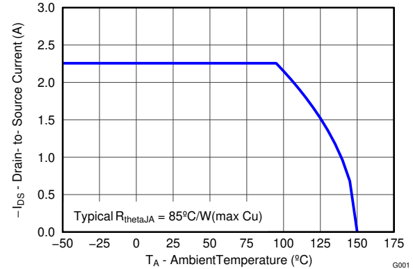
5-11. Maximum Drain Current vs Temperature
