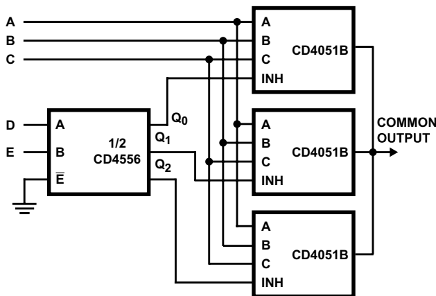
❏ 6-17. 24-to-1MUX Addressing
