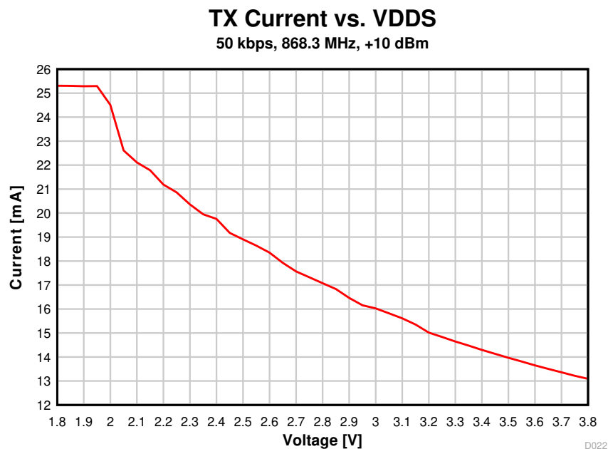
8-11. TX Current vs. Supply Voltage (VDD S ) (50 kbps, 868.3 MHz)
