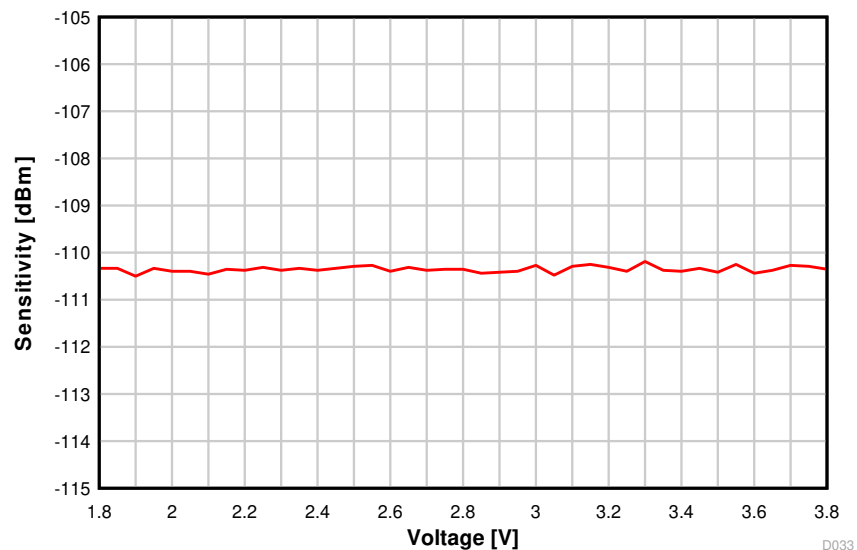
8-15. Sensitivity vs. Supply Voltage (VDD5) (50 kbps, 868.3 MHz)
