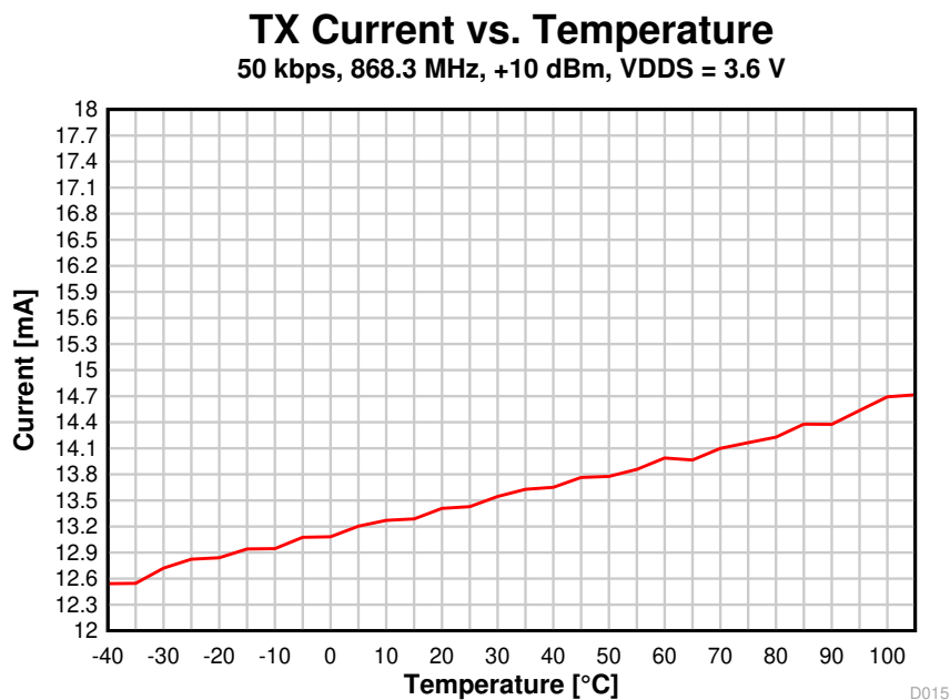
8-10. TX Current vs. Temperature (50 kbps, 868.3 MHz, VDD S = 3.6 V)
