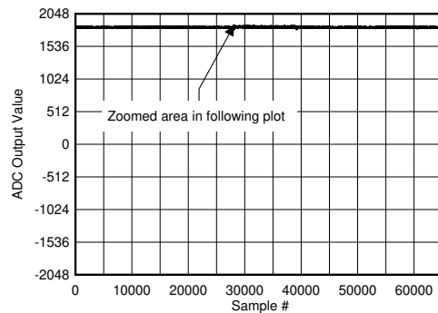
5-144. Background Calibration Core Transition (DC Signal)
