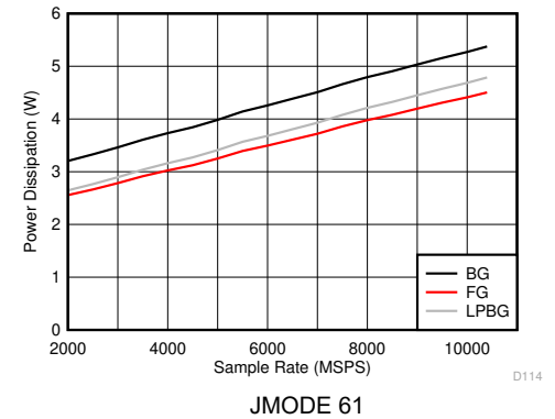
FIG 5-130. DES Mode: Power Dissipation vs Sample Rate
