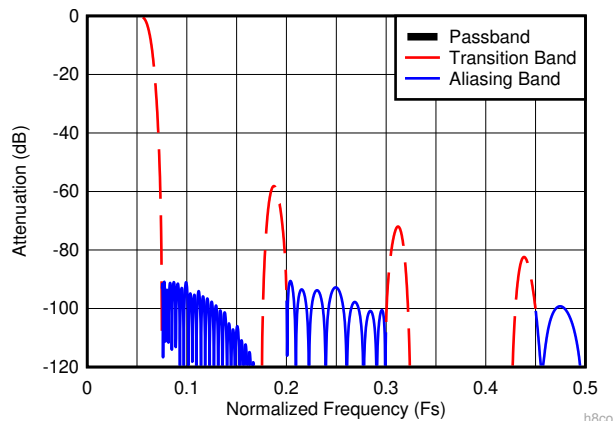
6-13. Decimate-by-8 Composite Response
