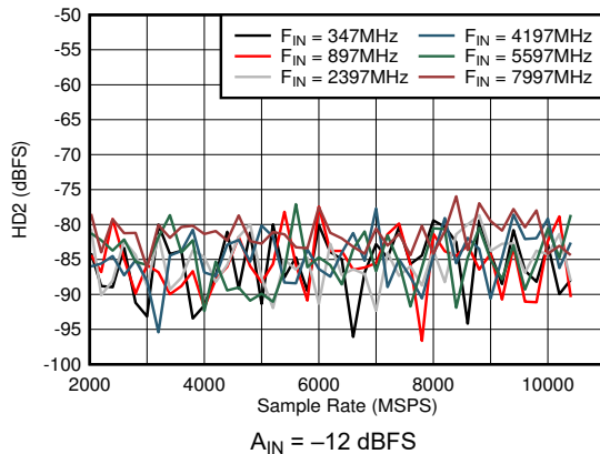
図 5-37. DES Mode: HD2 vs Sample Rate and Input Frequency
