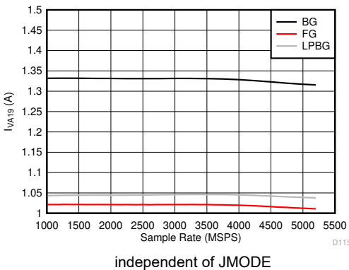
FIG 5-131. Dual Channel Mode: I_{VA19} vs Sample Rate
