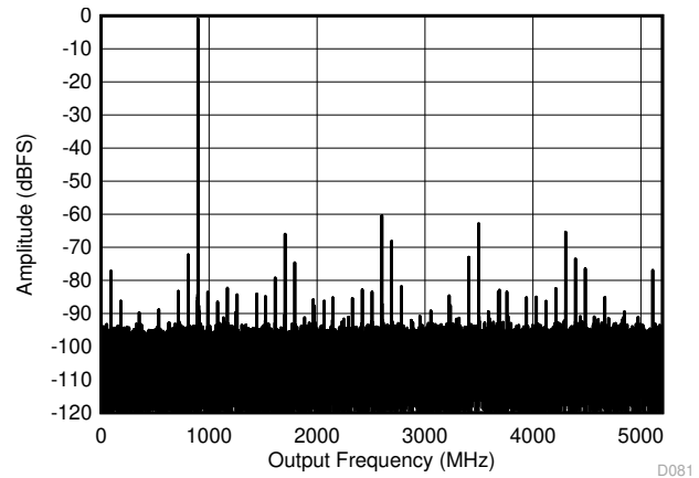
5-6. DES Mode: Single Tone FFT at 897 MHz
