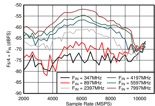
図 5-42. DES Mode: \text{Fs}/4 + F_{\text{IN}} vs Sample Rate and Input Frequency
