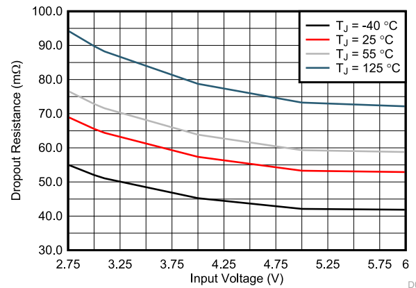
Figure 6-4. Dropout Resistance
