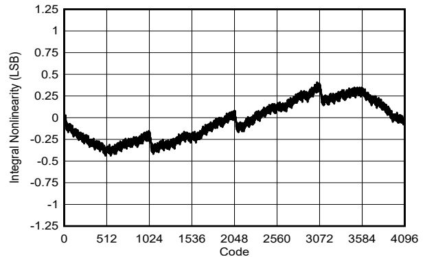
Figure 6-7. Integral Linearity Error vs Code
