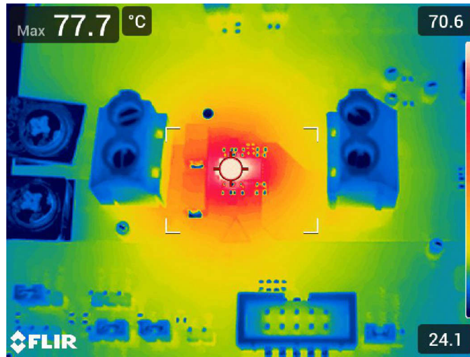
图 4-1. 热性能 (TPSM8287B30LAPEVM, V_{IN} = 5V , V_{OUT} = 0.6V , I_{OUT} = 30A )
