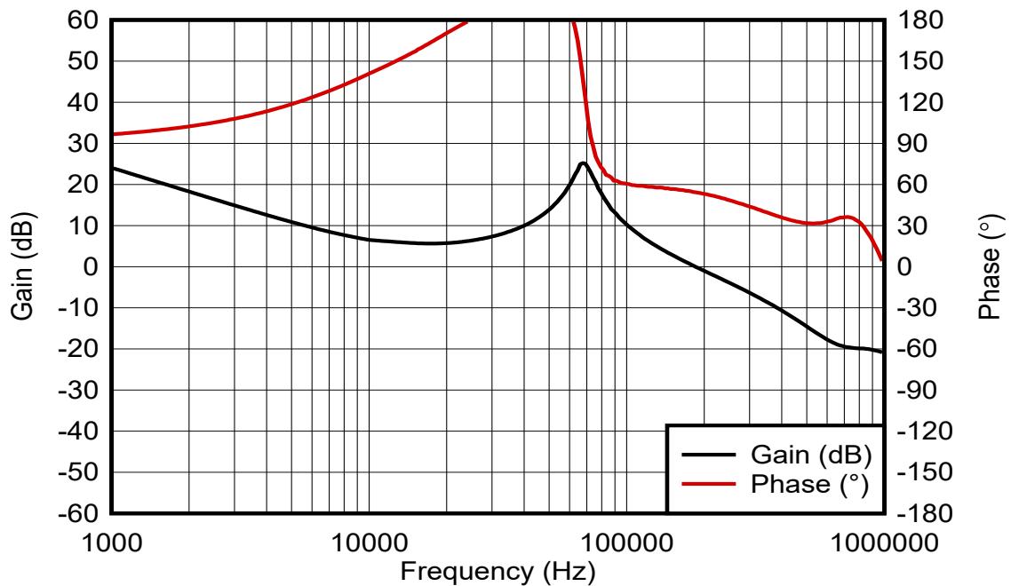
图 4-2. 环路响应测量 (TPSM8287B30LAPEVM, V_{IN} = 5V , V_{OUT} = 0.6V , I_{OUT} = 30A )
