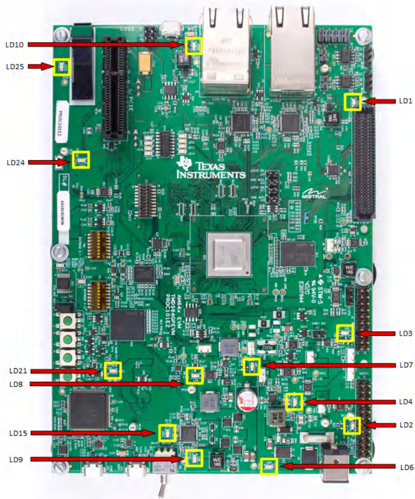
图 2-4. 电源正常 LED
