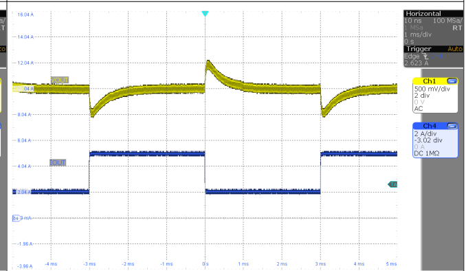
图 3-22. 负载阶跃 ( V_{IN} = 36V , I_{OUT} = 2A 至 5A )
