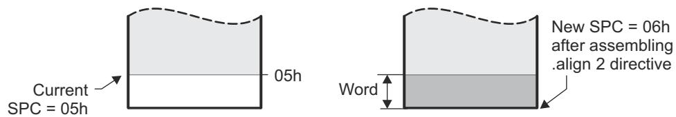
(b) Result of .align without an argument
