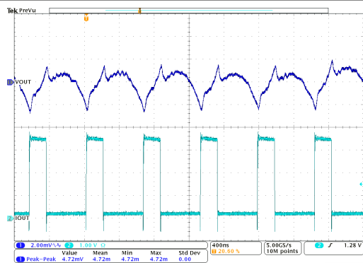
图 9-20. 负载瞬态 TPSM8287B30HAPx
