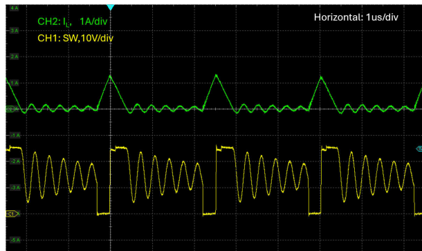
图 7-10. V_{in} = 14.4V , V_{out} = 24V , DEM, I_{load} = 0.1A
