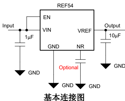
Basic Connection Diagram
