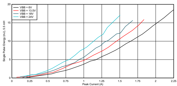
图 6-19. 单脉冲电感能量, L = 5.5\text{mH} , T_J = 125^\circ\text{C} , V_{BB} = 24\text{V} , I_{OUT} = 1.5\text{A}
