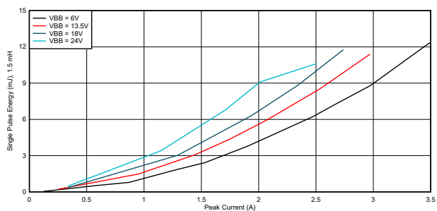
图 6-20. 单脉冲电感能量, L = 1.5\text{mH} , T_J = 125^\circ\text{C} , V_{BB} = 24\text{V} , I_{OUT} = 1.5\text{A}
