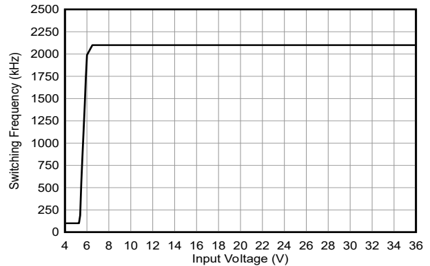
器件类型 = 1A 5V 输出 模式 = AUTO V IN = 12V F sw = 2MHz I OUT = 1A
