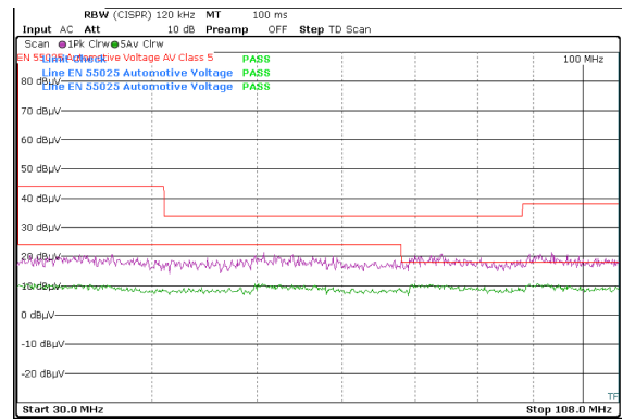
V_{OUT} = 3.3V F_{SW} = 2MHz I_{OUT} = 1A 频率跨度：30MHz 至 108MHz
