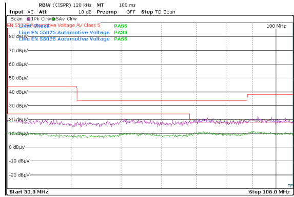
V_{OUT} = 5V F_{SW} = 2MHz I_{OUT} = 1A 频率跨度：30MHz 至 108MHz
