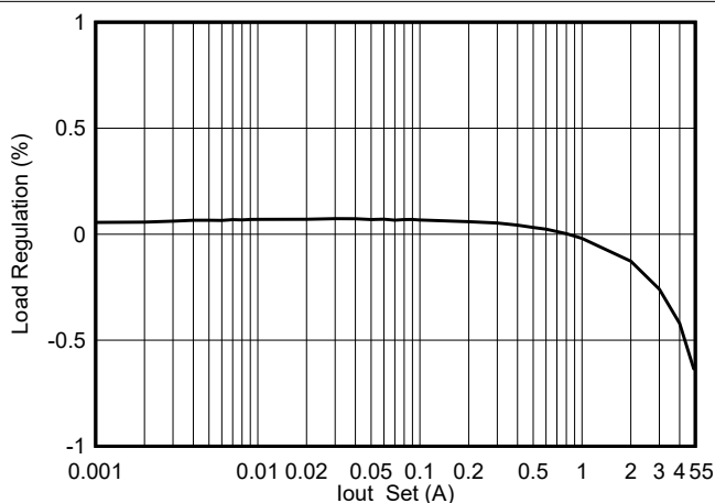
图 5-19. TPS54538 负载调节 (FCCM), V_{IN} = 24\text{V} , V_{OUT} = 12\text{V} , f_{SW} = 500\text{kHz}
