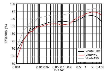
TPS54538 效率 ( V_{IN} = 24V , f_{SW} = 500kHz )
