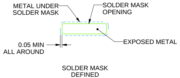
SOLDER MASK DETAILS
