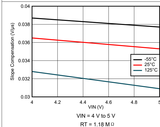
图 7-65. Slope Compensation Variation
