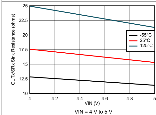
图 7-63. Output Sink Resistance Variation
