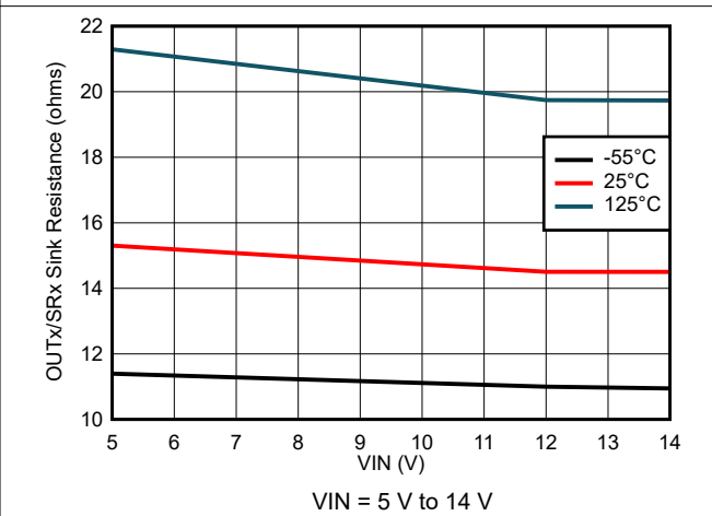
图 7-64. Output Sink Resistance Variation
