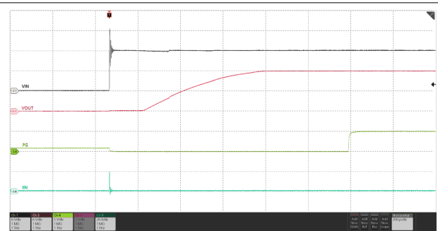
C_{OUT} = 22\ \mu\text{F} , C_{dVdt} = \text{Open} , EN/UVLO connected to IN through resistor ladder, 12\text{ V} hot-plugged to IN
