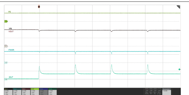
图 8-5. Transient Overload
