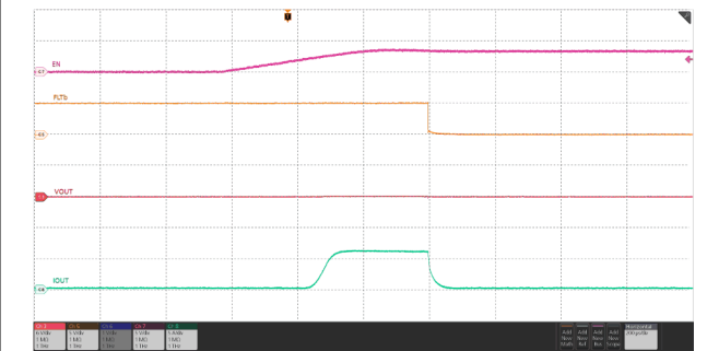
图 6-44. Output Short-Circuit During Steady State
