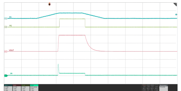
V_{IN} = 12\text{ V} , C_{OUT} = 22\ \mu\text{F} , C_{dVdt} = \text{Open} , V_{EN/UVLO} ramped from 0\text{ V} \rightarrow 1.4\text{ V} \rightarrow 0\text{ V}
