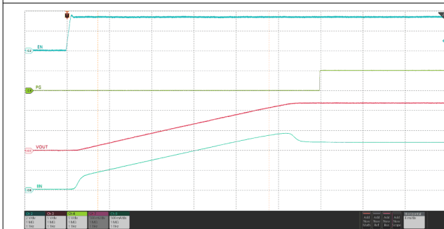
V_{IN} = 12\text{ V} , C_{OUT} = 470\ \mu\text{F} , R_{OUT} = 10\ \Omega , C_{dVdt} = 5100\text{ pF} , V_{EN/UVLO} stepped up to 3.3\text{ V}
