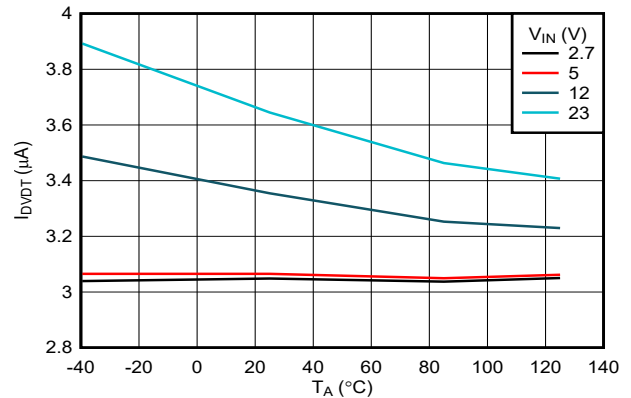
图 6-24. DVDT Charging Current vs Temperature
