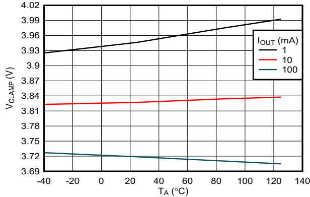
图 6-19. OVC Clamping Voltage (OVCSEL = GND) vs Load Current (TPS25972x Variant)
