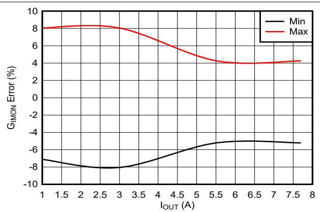
图 6-14. Analog Current Monitor Gain Accuracy
