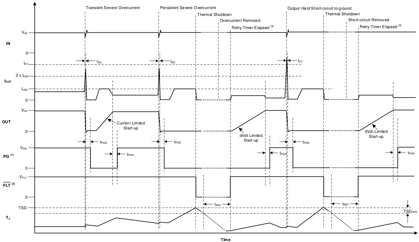
图 7-11. TPS2597xx Short-Circuit Response
