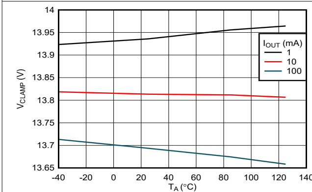
图 6-17. OVC Clamping Voltage (OVCSEL = 390 kΩ to GND) vs Load Current (TPS25972x Variant)
