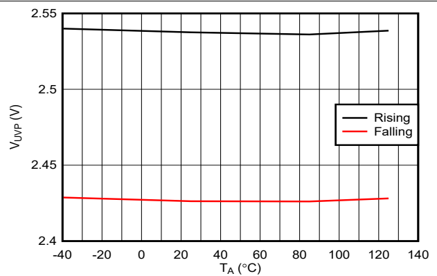
图 6-6. IN Undervoltage Threshold vs Temperature
