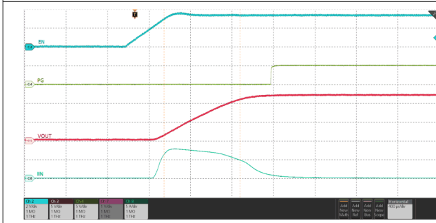
V_{IN} = 12\text{ V} , C_{OUT} = 470\ \mu\text{F} , C_{dVdt} = \text{Open} , V_{EN/UVLO} stepped up to 3.3\text{ V}
