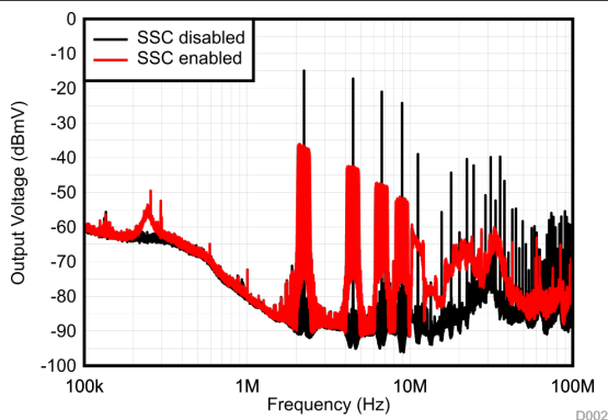
V_{OUT} = 0.75V PWM T_A = 25^\circ C V_{IN} = 5V I_{OUT} = 11.3A
