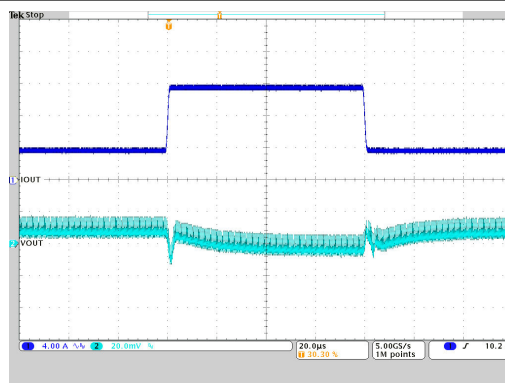
V_{OUT} = 0.75V PWM , TPS62874 T_A = 25^\circ C 压降启用 I_{OUT} = 3.8A 至 11.3A 至 3.8A V_{IN} = 5V
