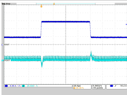
V_{OUT} = 0.75V PWM ; TPS62874 T_A = 25^\circ C 压降禁用 I_{OUT} = 3.8A 至 11.3A 至 3.8A V_{IN} = 5V
