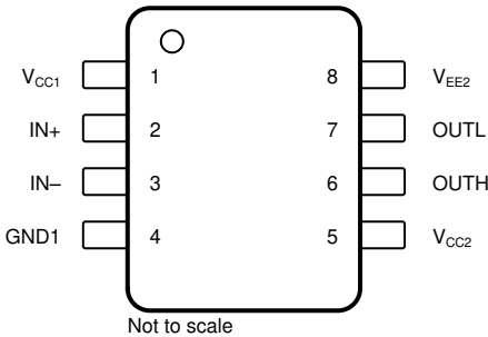
图 5-1. UCC5320S、UCC5350SB 和 UCC5390S 8 引脚 SOIC 顶视图
