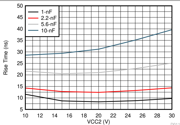
图 6-38. UCC5350SBD Rise Time vs C_L and V_{\text{CC2}}
