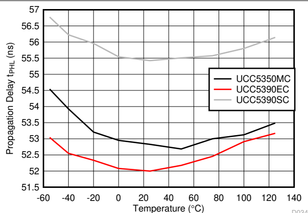
图 6-35. Propagation Delay t_{\text{PHL}} vs Temperature
