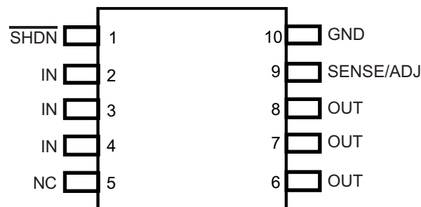
U PACKAGE (TOP VIEW)
