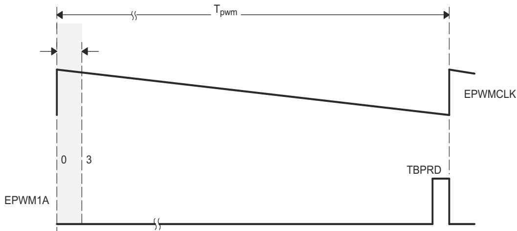
Figure 27-115. High % Duty Cycle Range Limitation Example (HRPCTL[HRPE] = 0)
