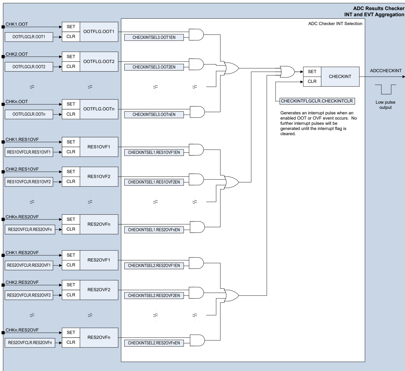
Figure 22-28. ADC Result Checker Interrupt Aggregation
