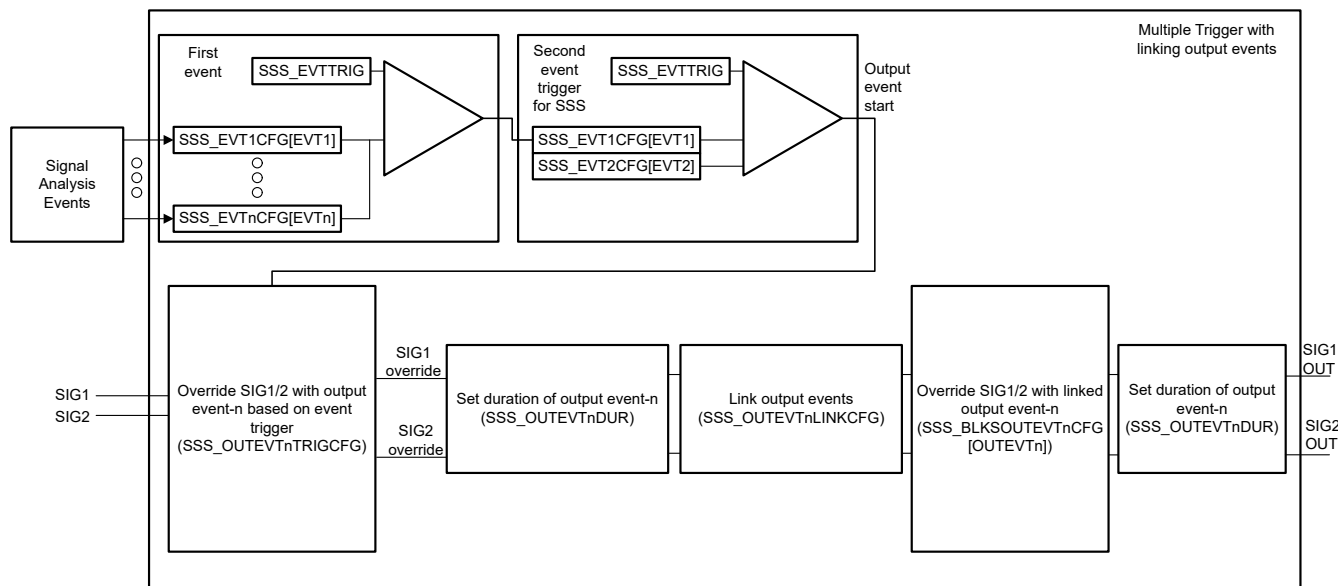
Figure 18-11. Linking Output Events for Generating Pattern Output Events
