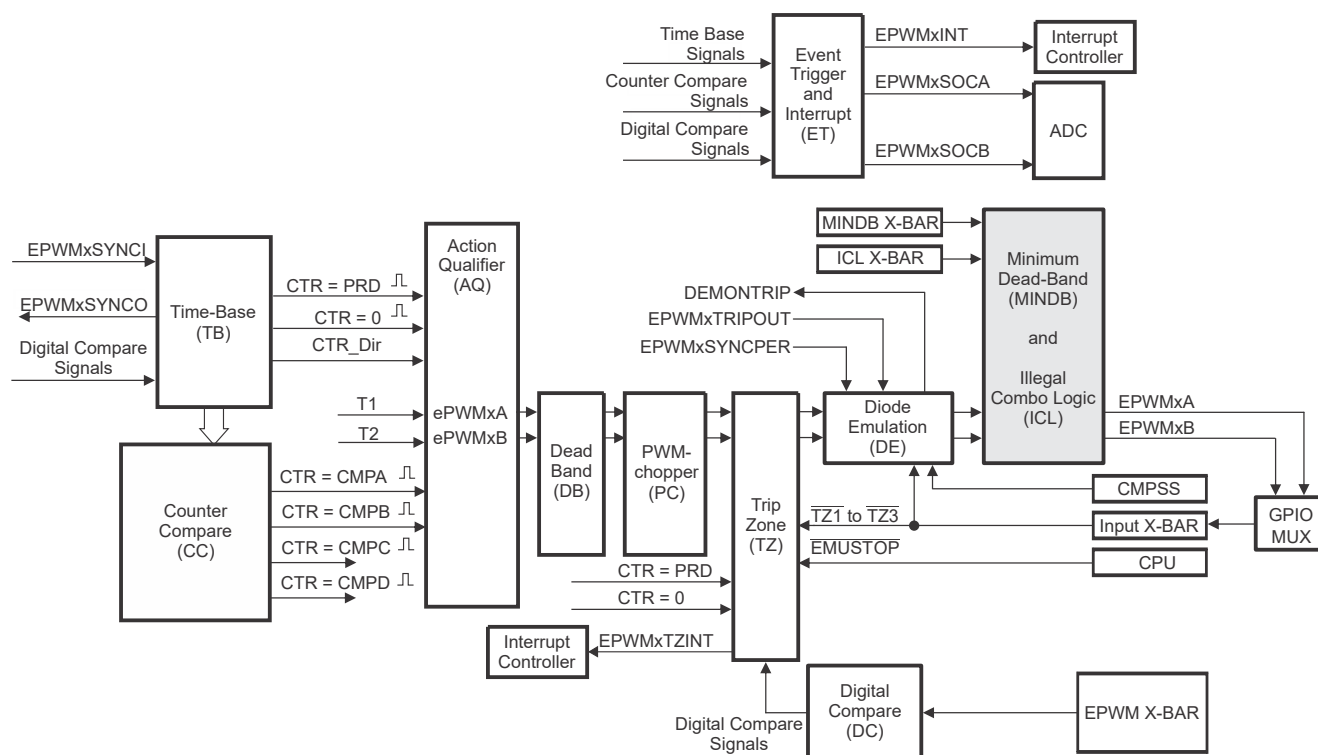
Figure 27-61. Minimum Dead-Band and Illegal Combo Logic Submodule
