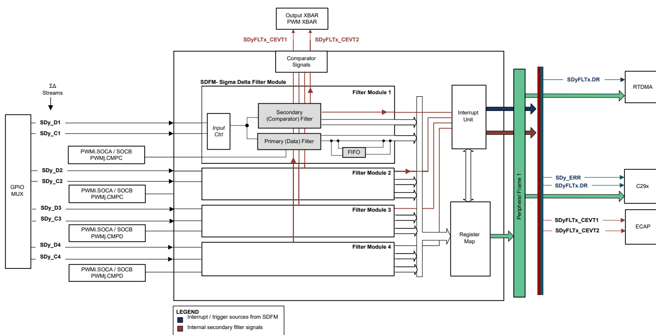
Figure 29-2. Sigma Delta Filter Module (SDFM) Block Diagram
