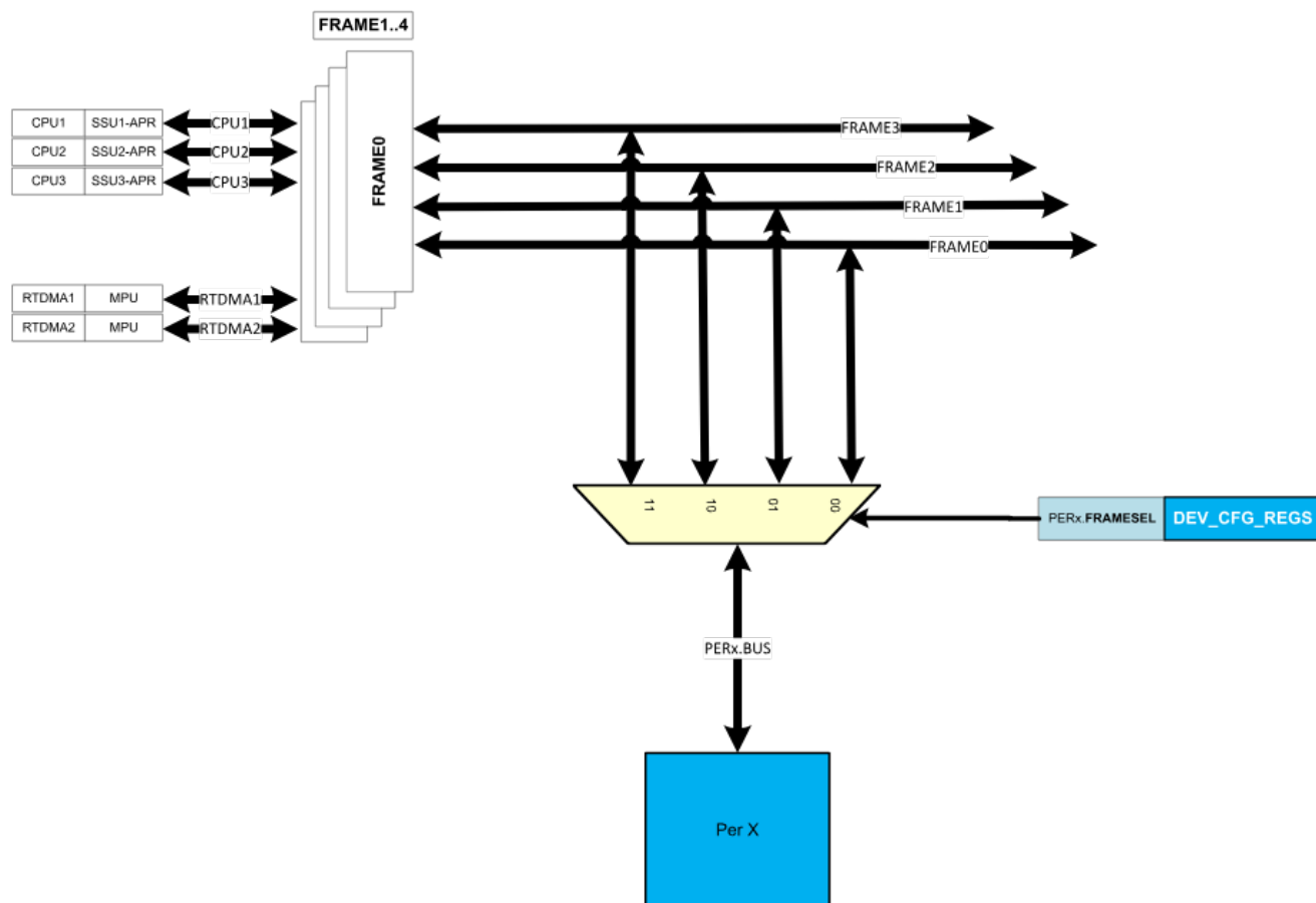
Figure 2-11. Peripheral Access Configuration
