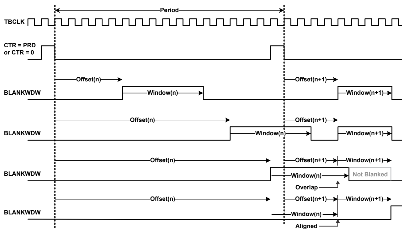
Figure 27-79. Blanking Window Timing Diagram
