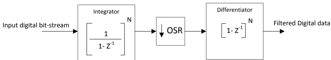
Figure 29-7. Simplified Sinc Filter Architecture
