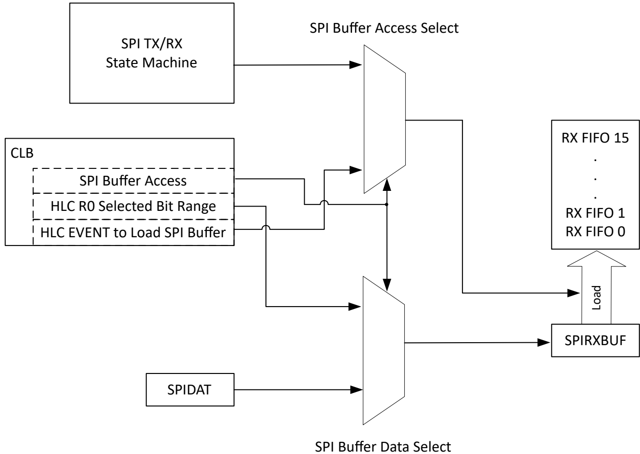
Figure 10-21. CLB Control of SPI RX Buffer
