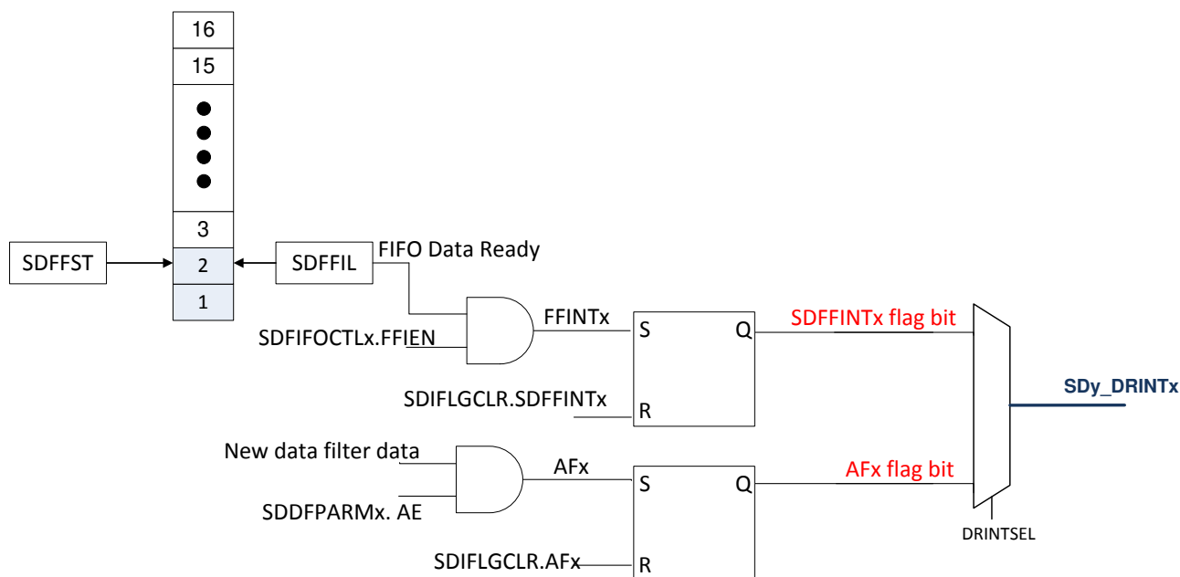
Figure 29-14. SDFM Data Ready (SDy_DRINTx) Interrupt
