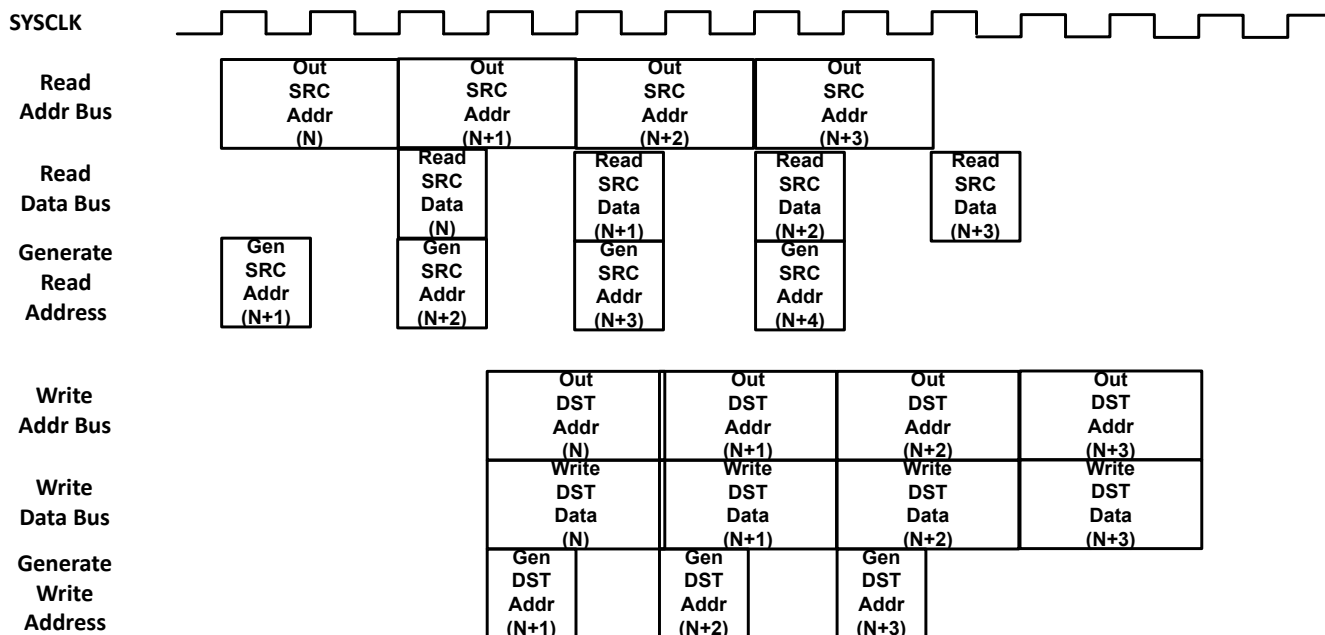
Figure 12-4. 3-stage Pipeline: With One Read Stall
