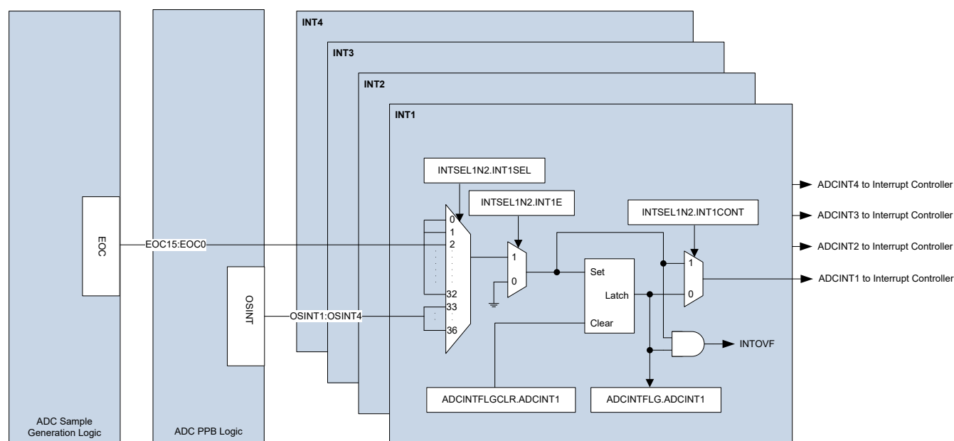
Figure 22-22. ADC End-of-Conversion (EOC) Signal Interrupts
