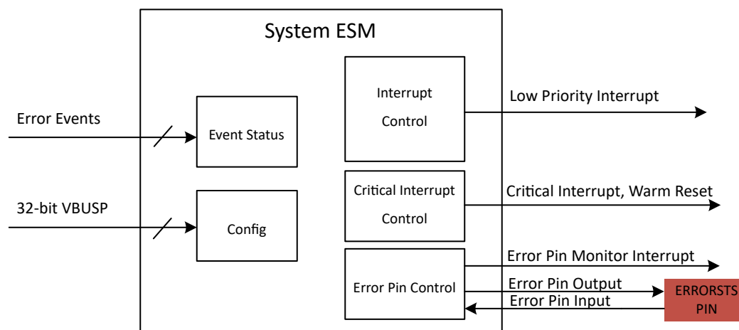
Figure 7-6. System ESM Block Diagram
