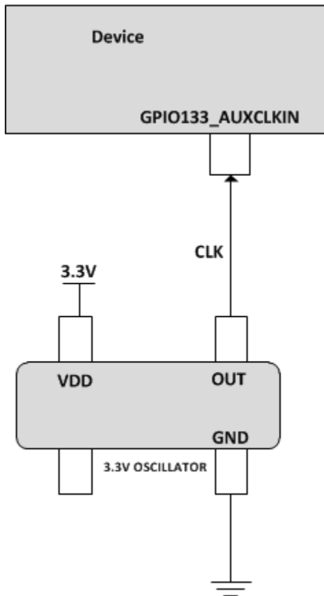
Figure 2-8. Auxiliary Clock Input (AUXCLKIN)
