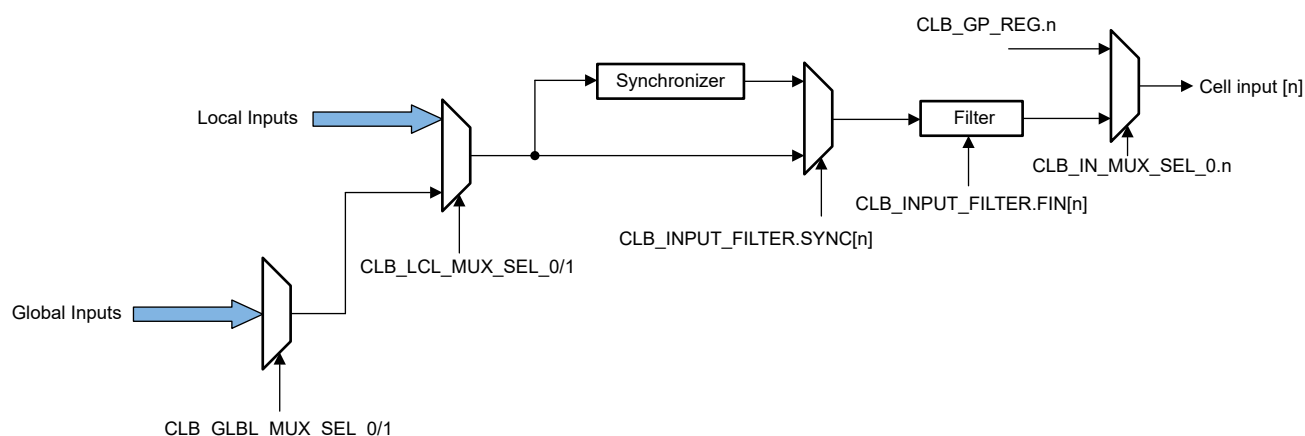
Figure 10-6. CLB Input Mux and Filter
