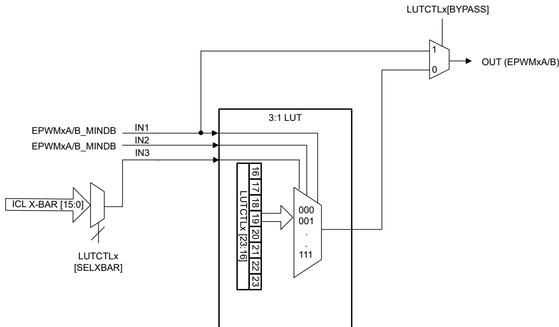
Figure 27-68. Illegal Combo Logic Block Diagram
