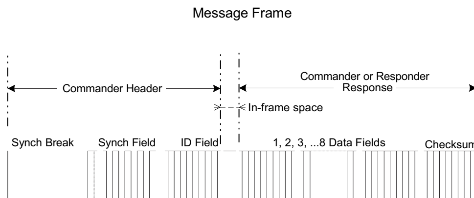
Figure 36-12. LIN Protocol Message Frame Format: Commander Header and Responder Peripheral Response
