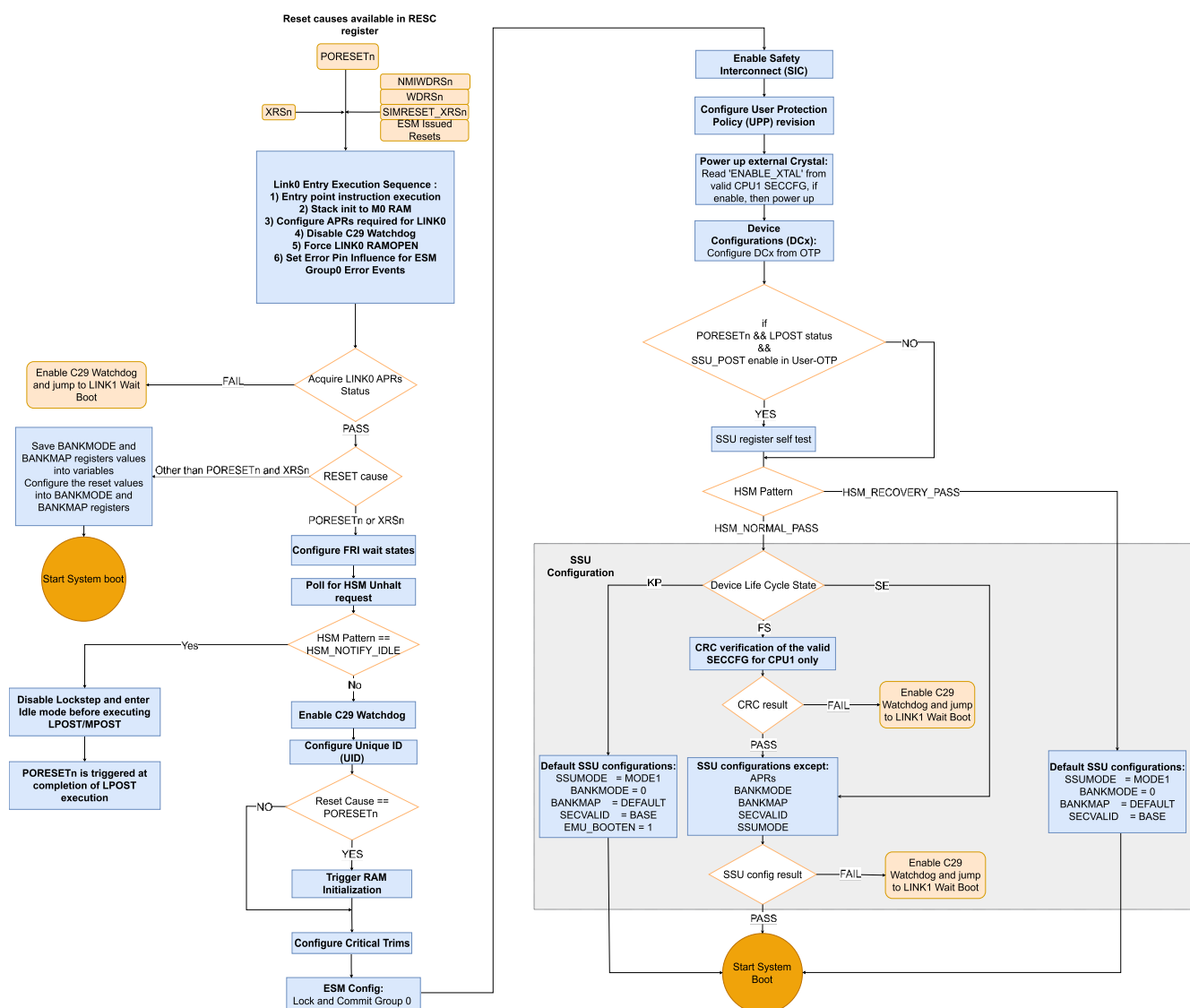
Figure 3-2. Device Boot Flow from Reset to System Boot
