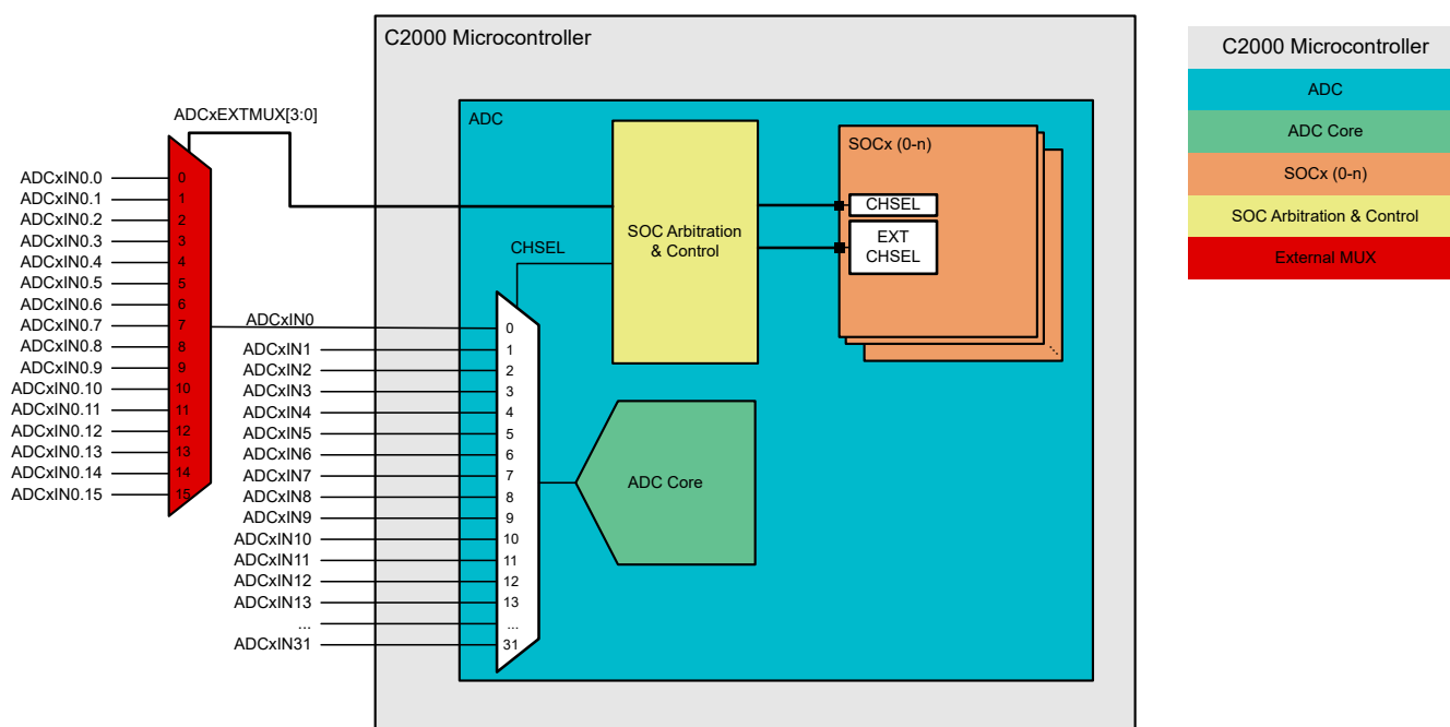
Figure 22-13. ADC with External Input Mux
