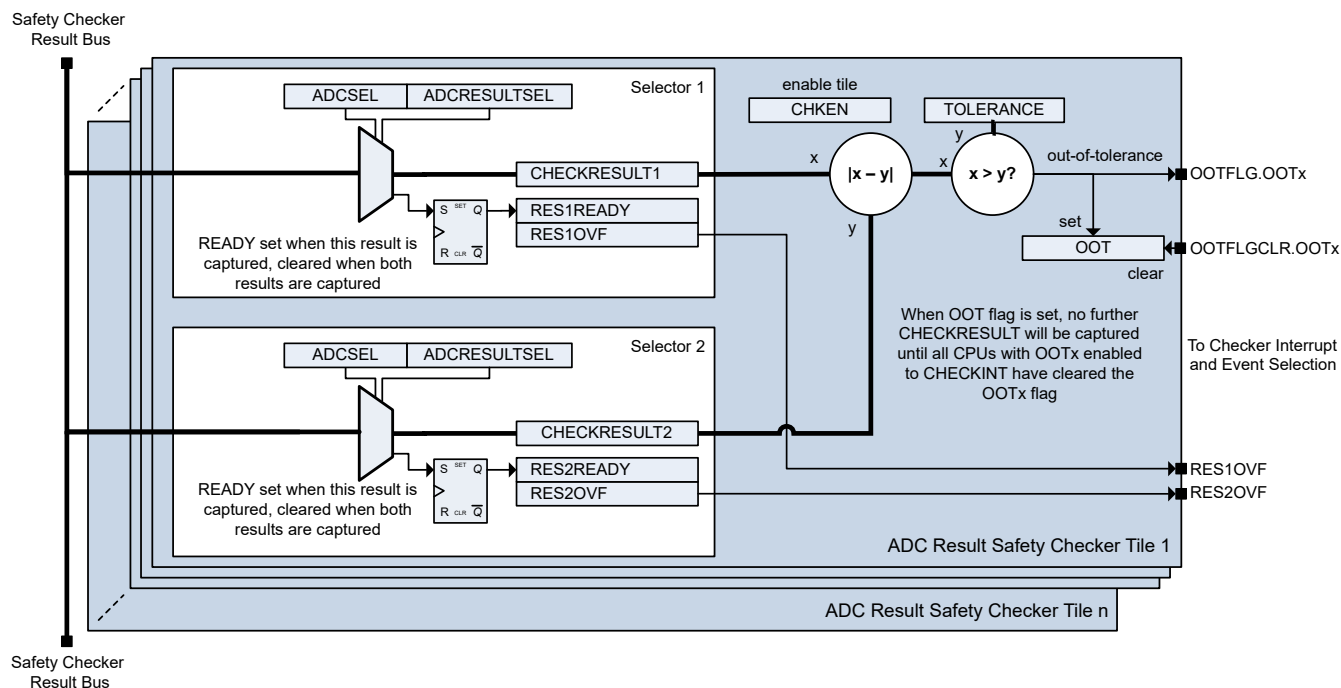
Figure 22-27. ADC Safety Checker Tile Diagram
