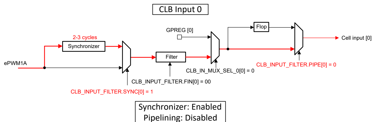
Figure 10-7. CLB Input Synchronization Example
