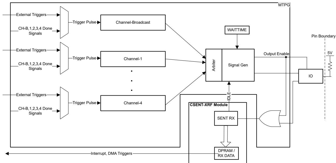
Figure 38-1. SENT Block Diagram
