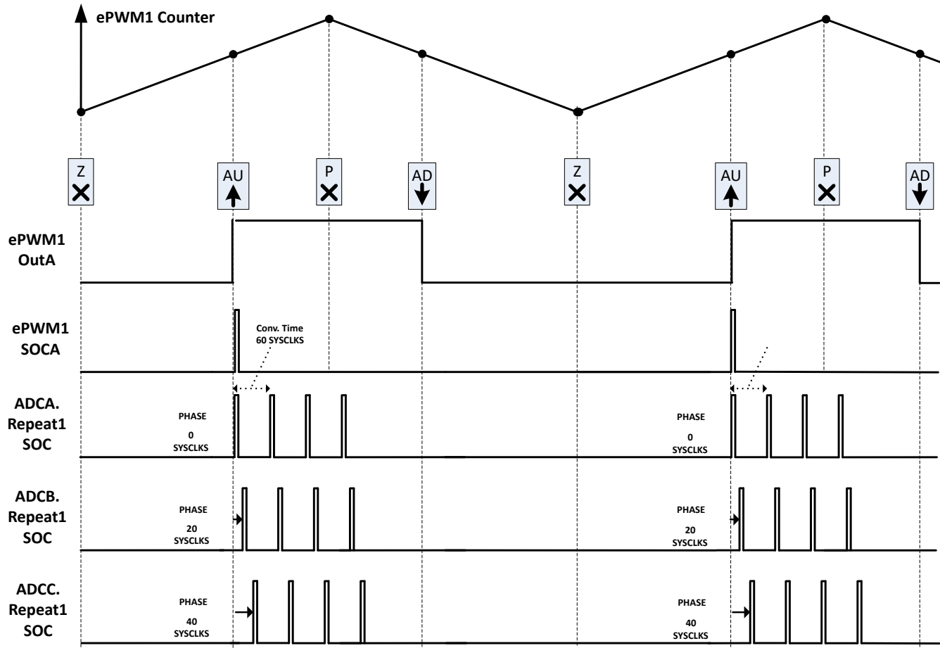
Figure 22-8. ADC Interleaved Trigger Example (12 Samples Across 3 ADCs)
