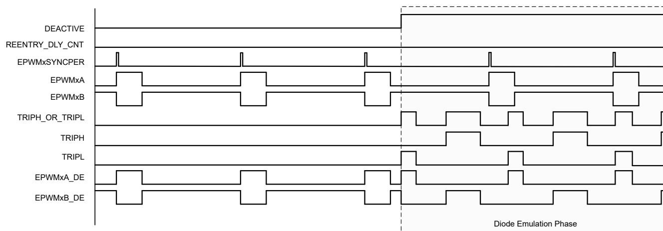
Figure 27-59. Diode Emulation Mode Timing Diagram
