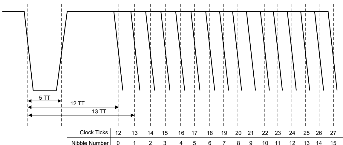
Figure 38-3. Nibble Pulse
