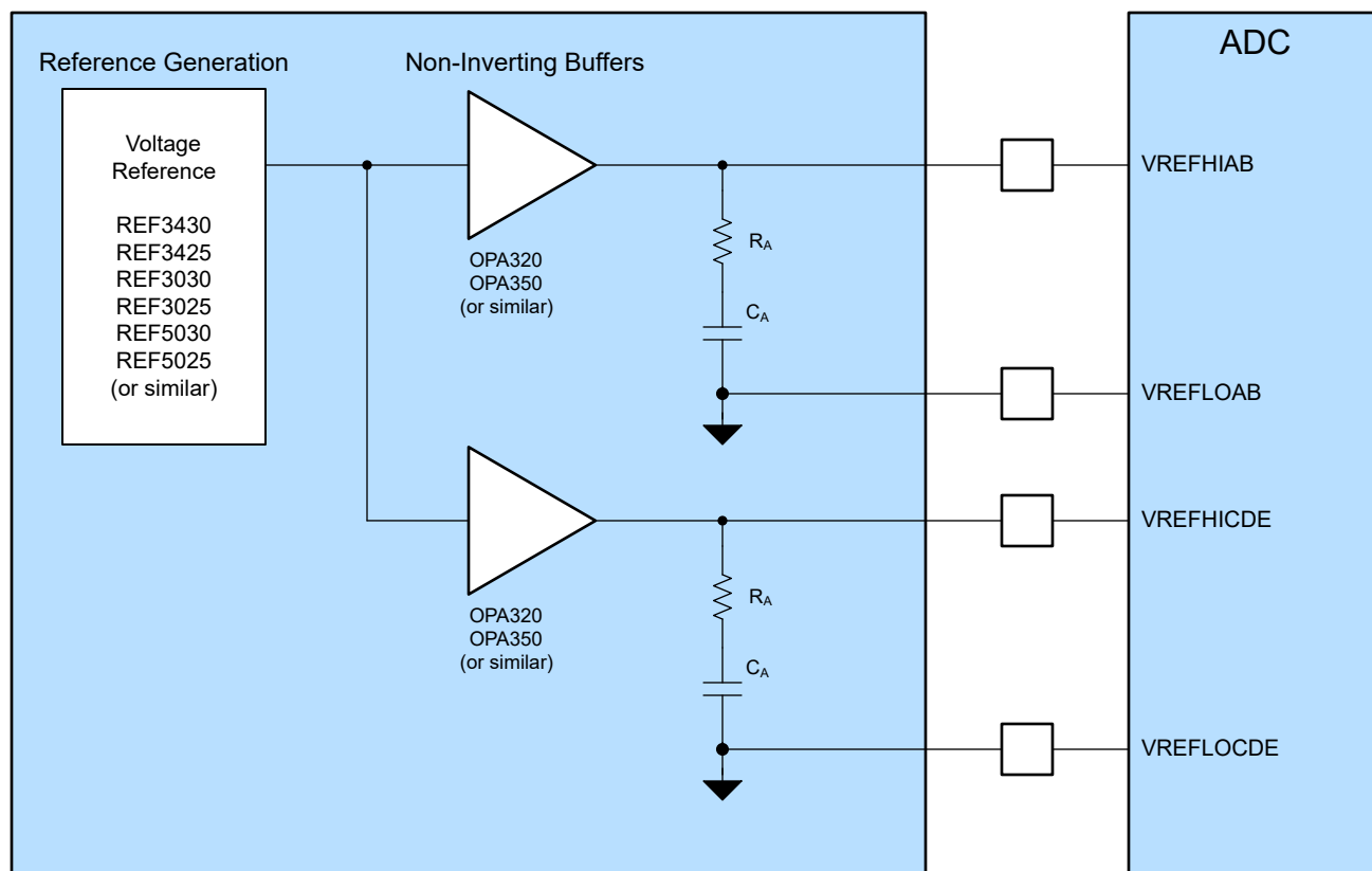
Figure 22-43. ADC Reference System
