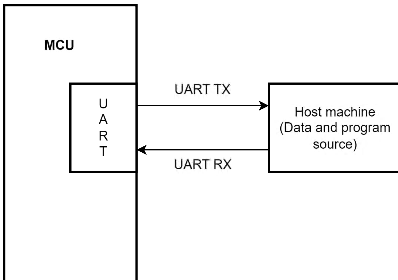
Figure 3-12. UART Boot Mode
