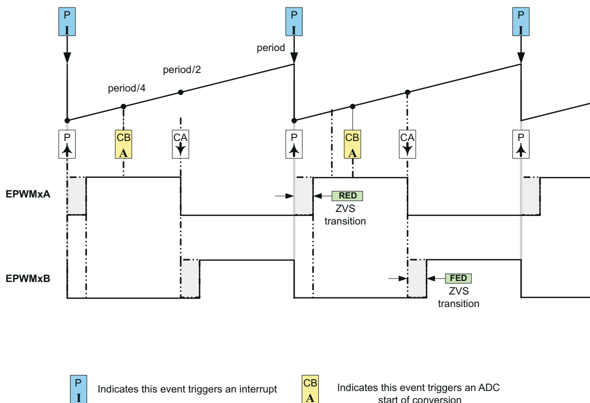
Figure 27-107. H-Bridge LLC Resonant Converter PWM Waveforms
