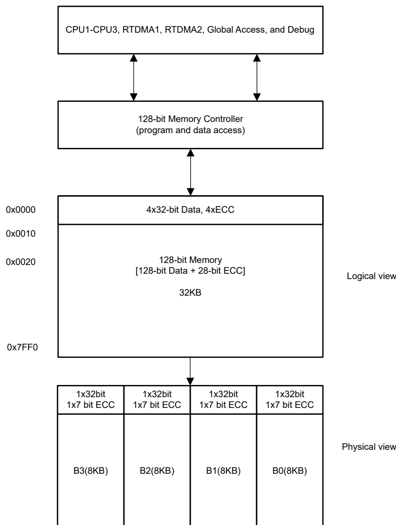
Figure 2-15. Generic view of 128-Bit Memory
