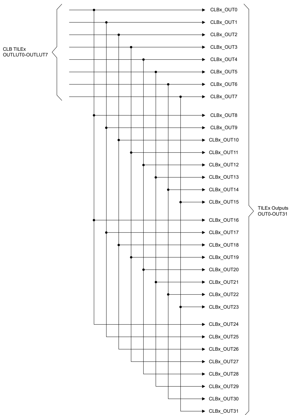
Figure 10-9. CLB Outputs
