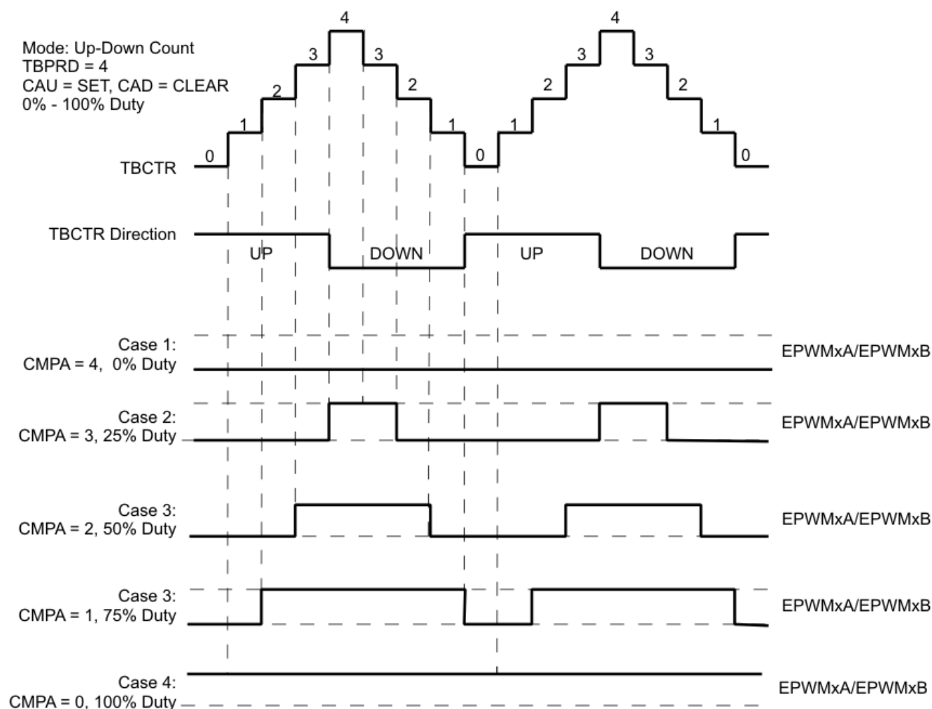
Figure 27-26. Up-Down Count Mode Symmetrical Waveform
