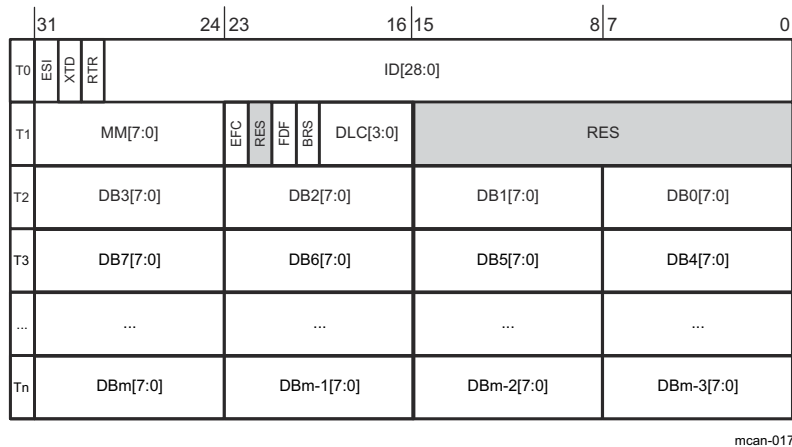
Figure 30-21. Tx Buffer Element Structure
