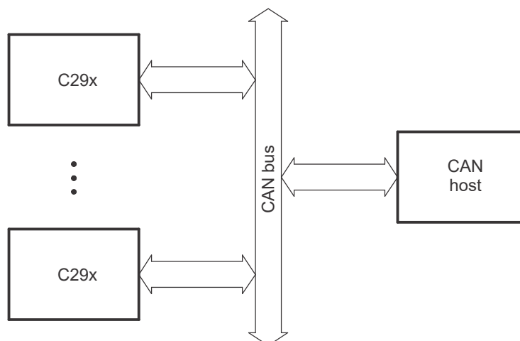
Figure 3-11. Overview of CAN-A Bootloader Operation
