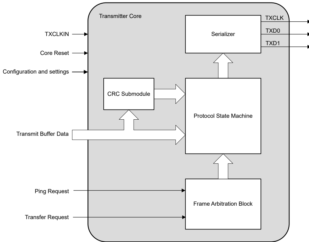
Figure 32-4. FSI Transmitter Core Block Diagram
