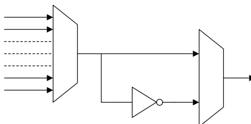
Figure 16-6. Trace Qualifier Input Conditioning Circuit
