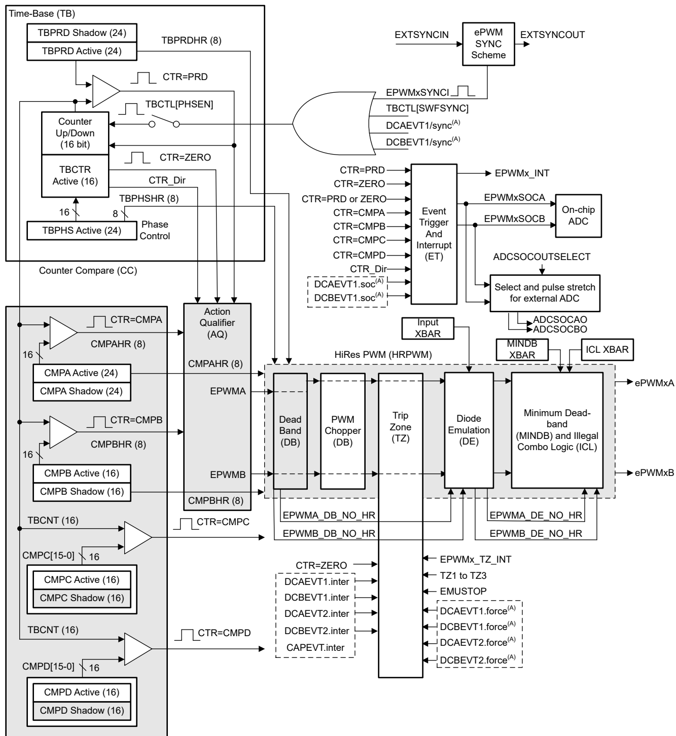
Figure 27-3. ePWM Modules and Critical Internal Signal Interconnects
