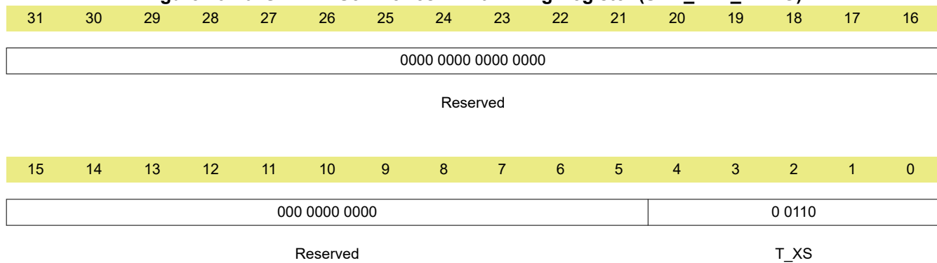
Figure 13-20. SDRAM Self Refresh Exit Timing Register (SDR_EXT_TMNG)
