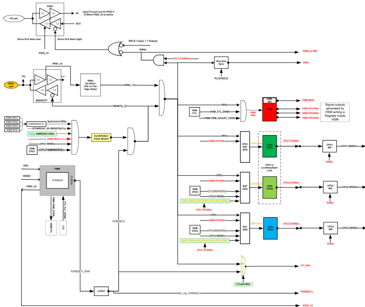
Figure 2-1. Device Reset Diagram
