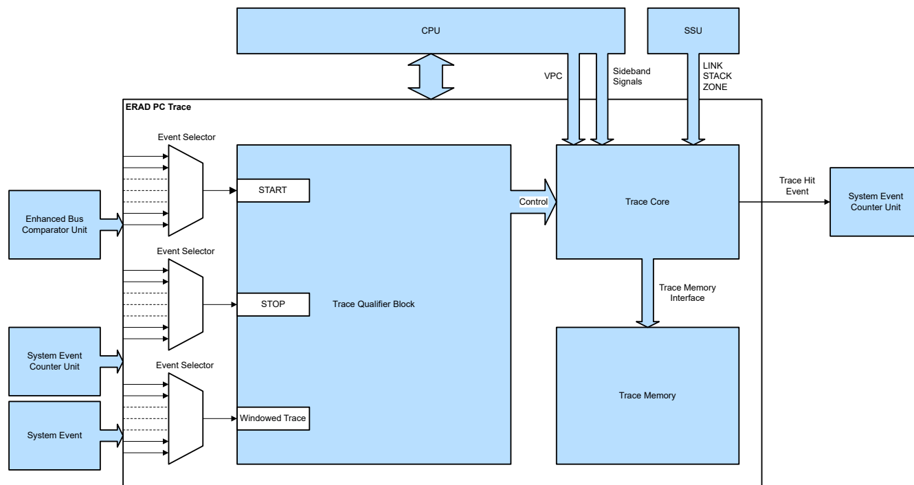
Figure 16-5. PC Trace Block Diagram
