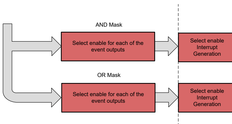
Figure 16-2. EBC Units Event Masking
