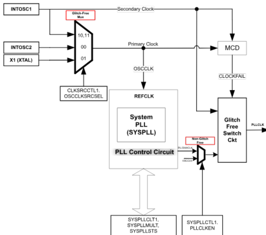
Figure 2-10. Missing Clock Detection Logic
