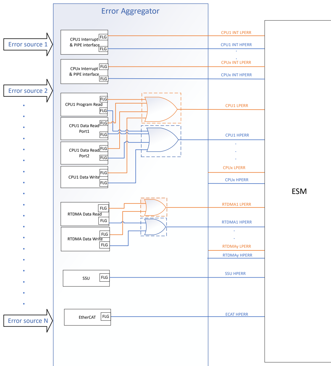
Figure 6-3. Error Aggregator Interface
