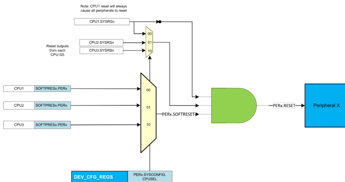
Figure 2-2. Software and SYSRSn Connectivity Diagram for Peripheral Reset
