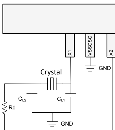
Figure 2-6. External Crystal
