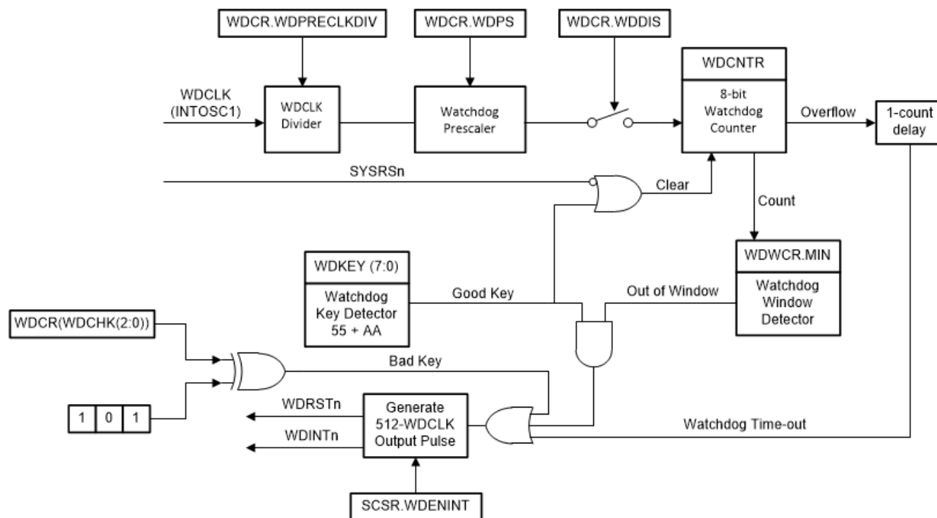
Figure 2-13. CPU Watchdog Timer Module
