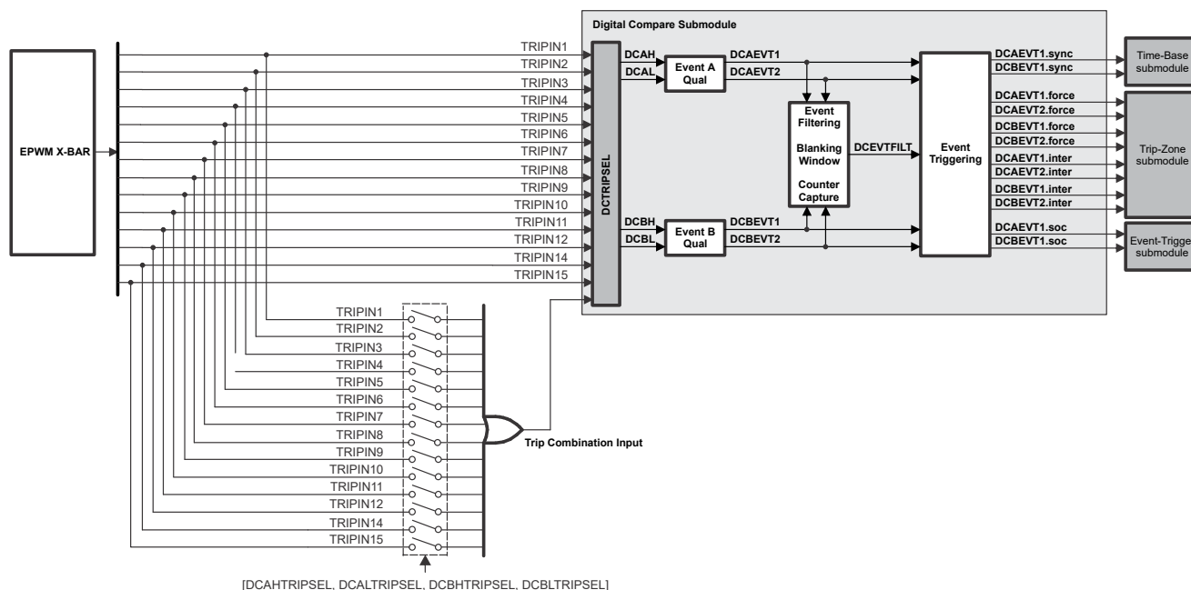
Figure 27-74. Digital-Compare Submodule High-Level Block Diagram
