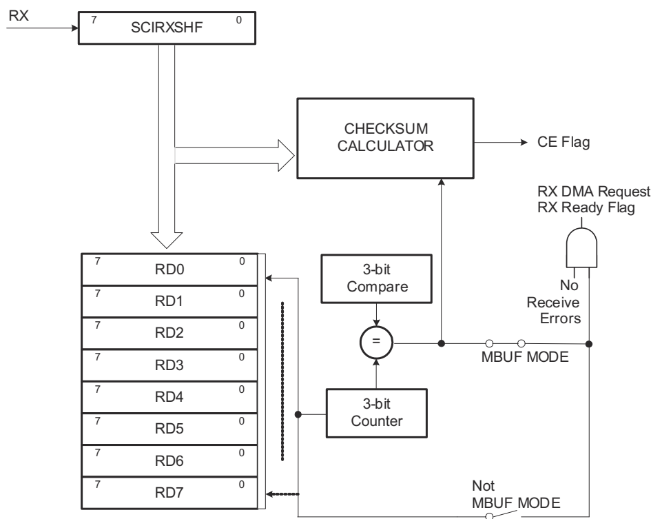
Figure 36-8. Receive Buffers
