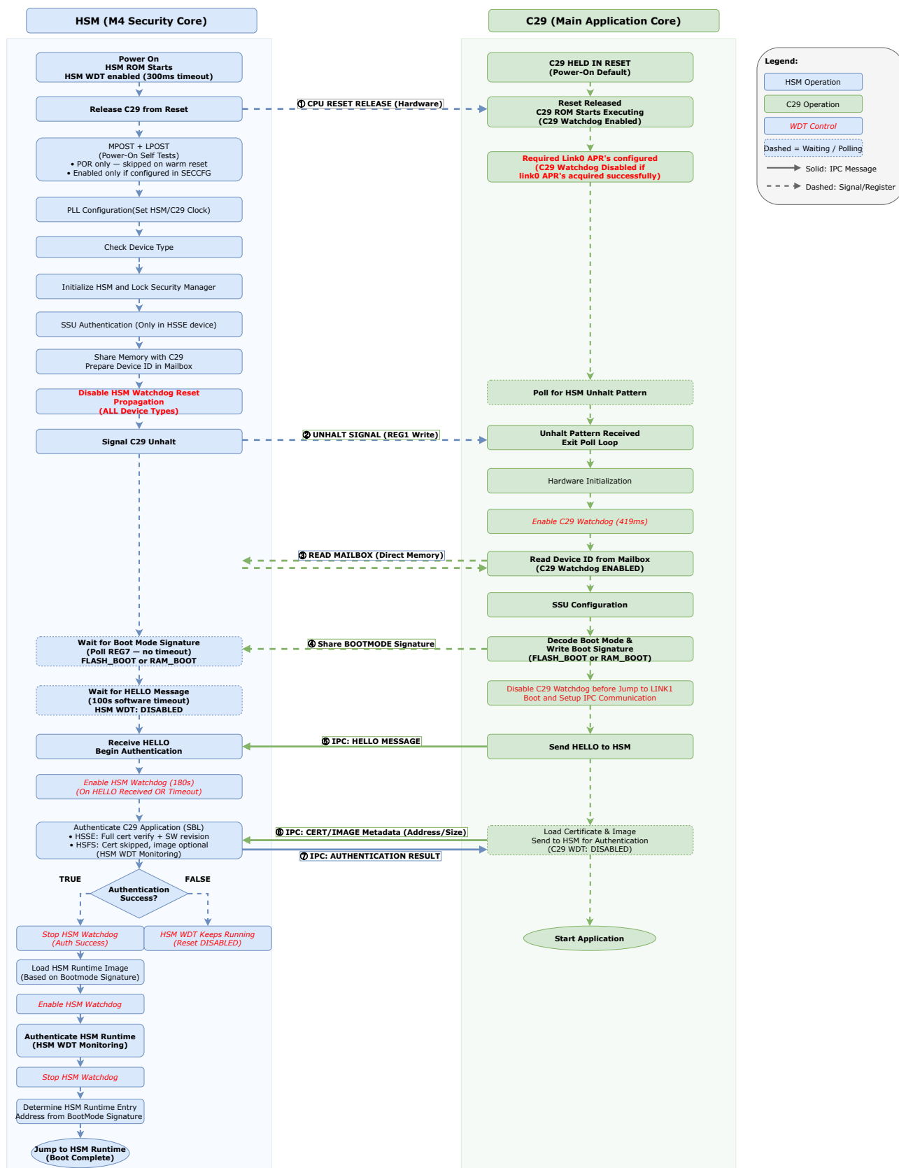
Figure 3-1. F29x device boot flow high level
