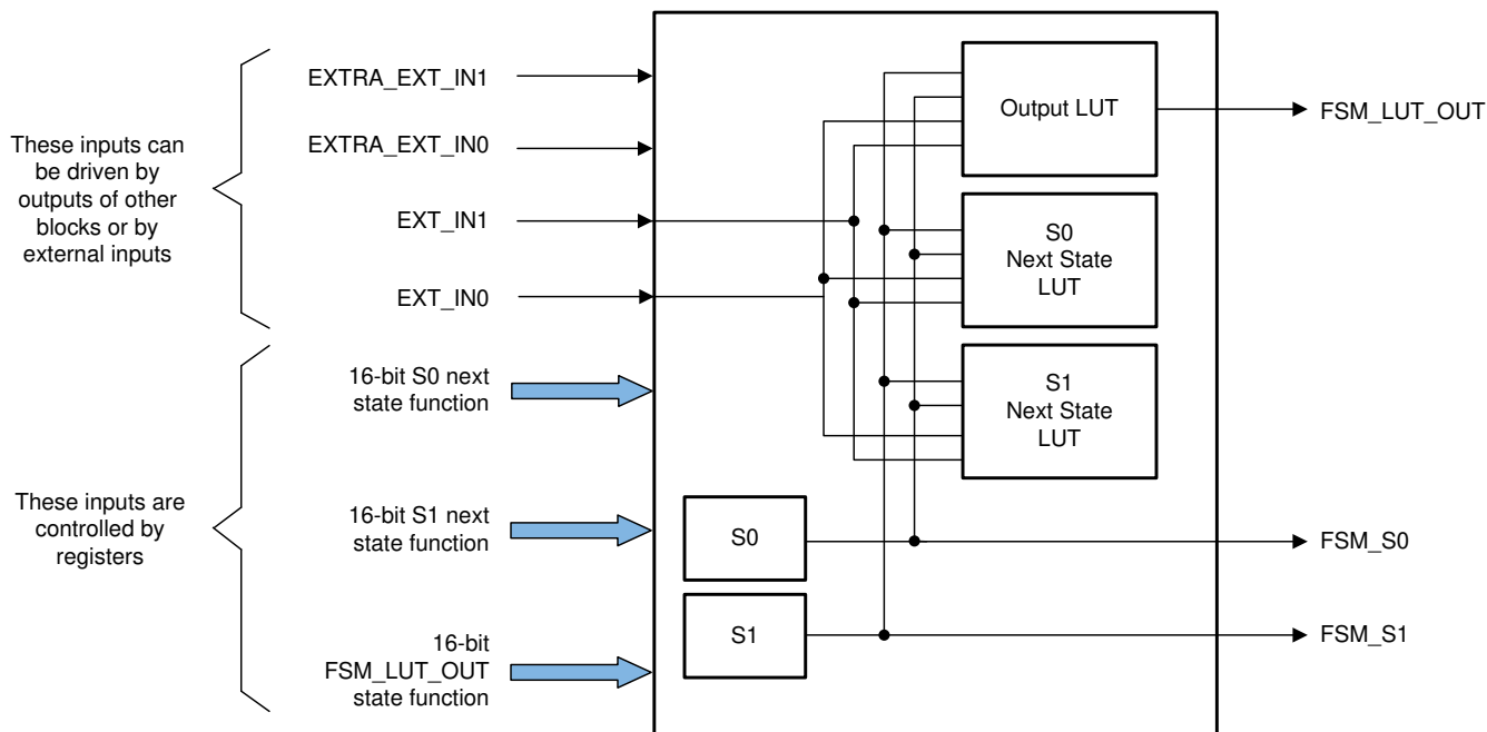
Figure 10-14. FSM Block
