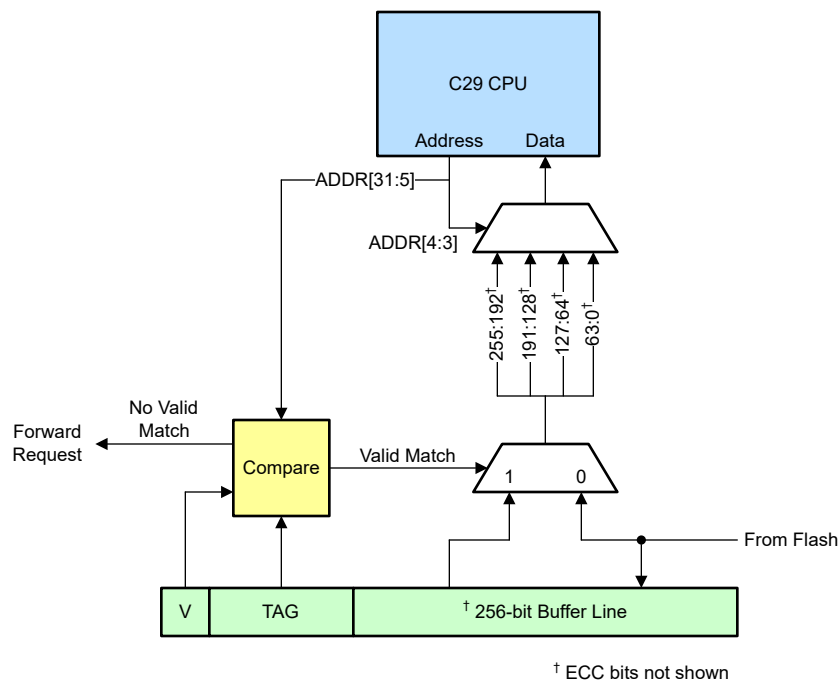
Figure 8-3. Flash Data Line Buffer for Interleaved Banks
