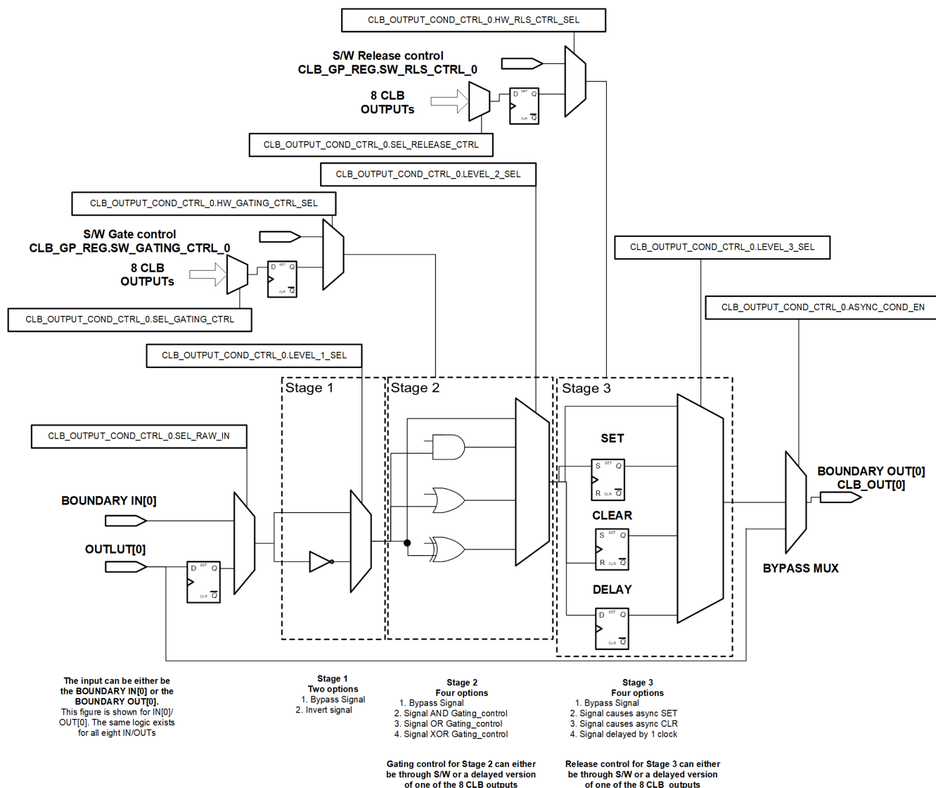
Figure 10-18. AOC Block
