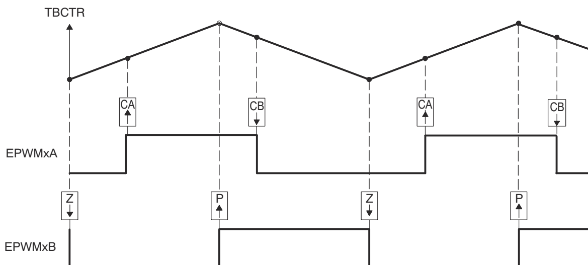
Figure 27-31. Up-Down Count, Dual-Edge Symmetric Waveform, with Independent Modulation on EPWMxA and EPWMxB — Complementary
