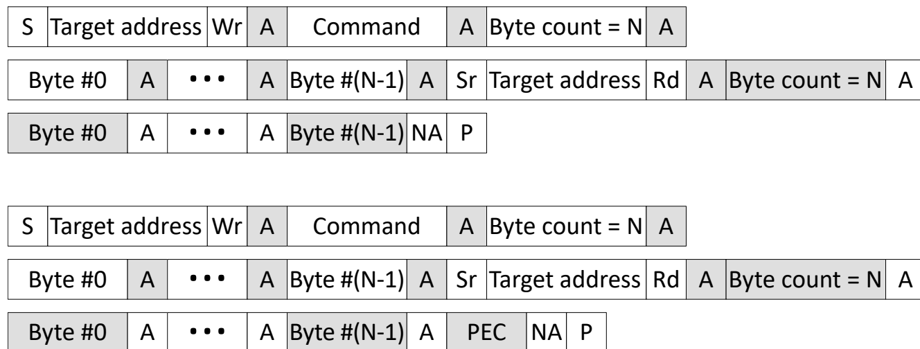
Figure 34-23. Block Write-Block Read Process Call Message With and Without PEC
