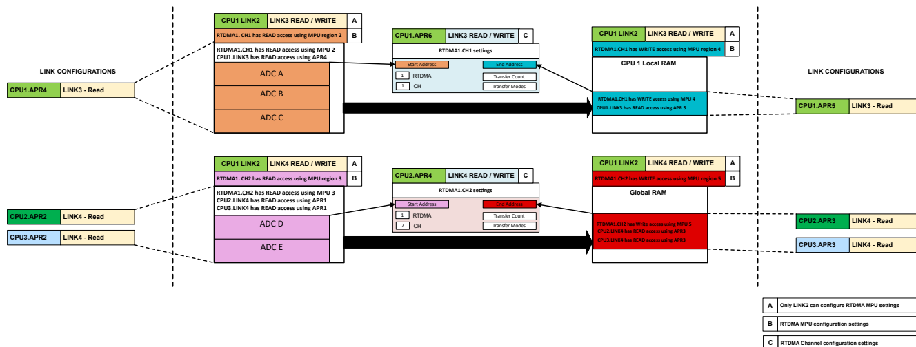
Figure 12-8. Peripheral-to-Memory Transfer Example
