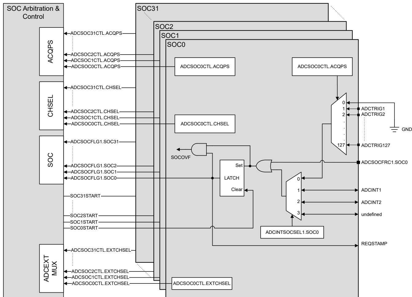
Figure 22-2. SOC Block Diagram
