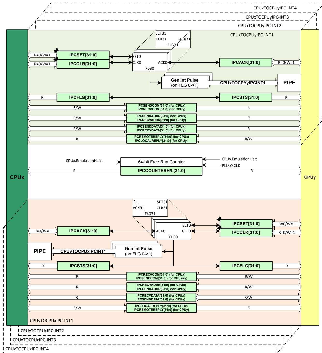
Figure 15-1. IPC Module Architecture
