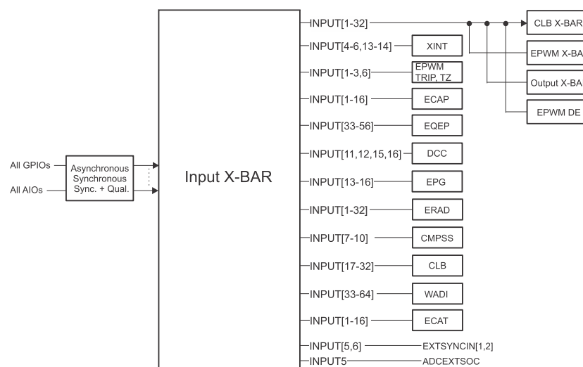
Figure 19-1. Input X-BAR
