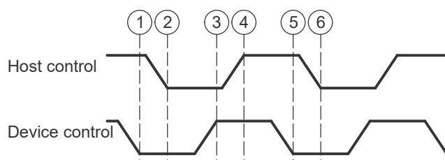
Figure 3-9. Parallel GPIO Bootloader Handshake Protocol
