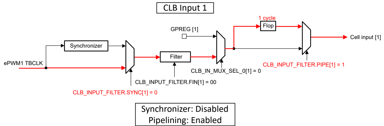
Figure 10-8. CLB Input Pipelining Example
