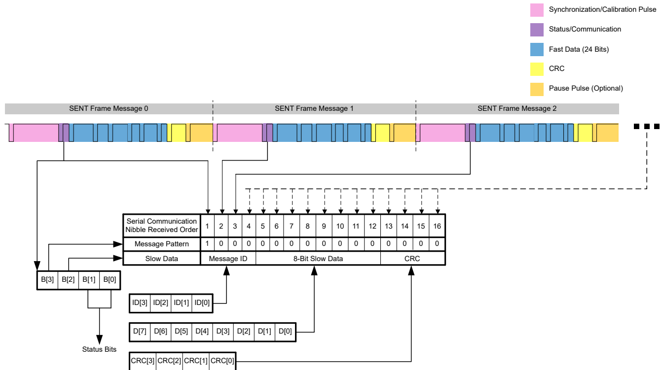
Figure 38-5. Short Serial Message
