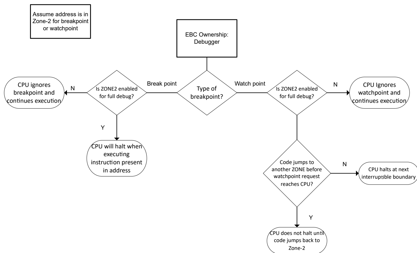
Figure 16-7. EBC Owned by Debugger
