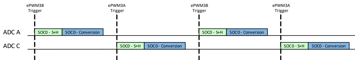
Figure 22-42. Example: Synchronous Equivalent Operation with Non-Overlapping Conversions
