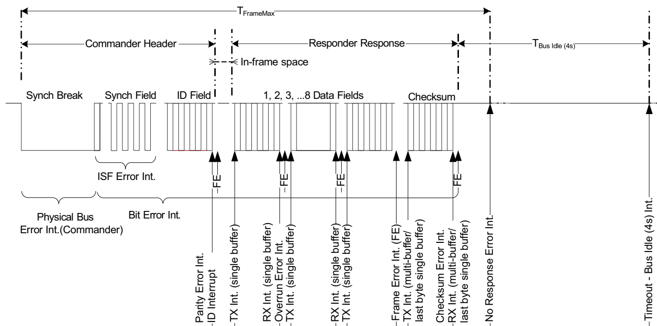
Figure 36-25. LIN Message Frame Showing LIN Interrupt Timing and Sequence
