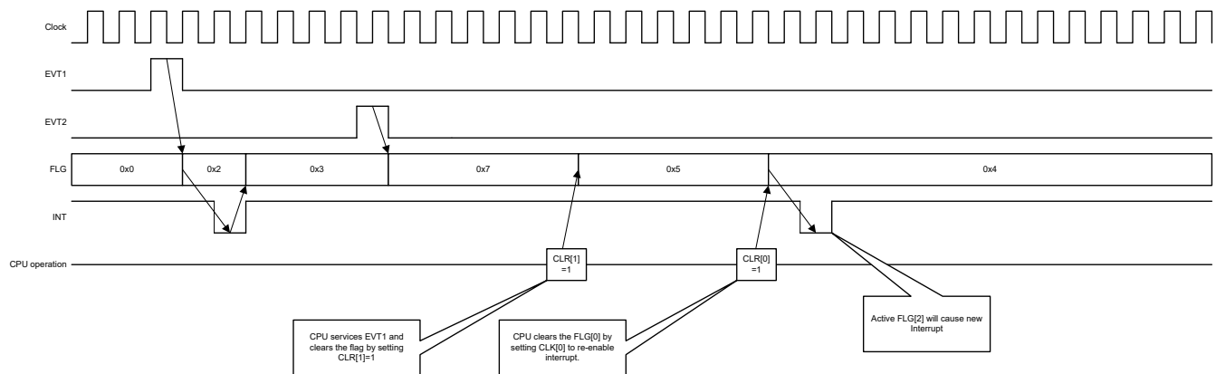
Figure 38-10. Interrupt Trigger Example
