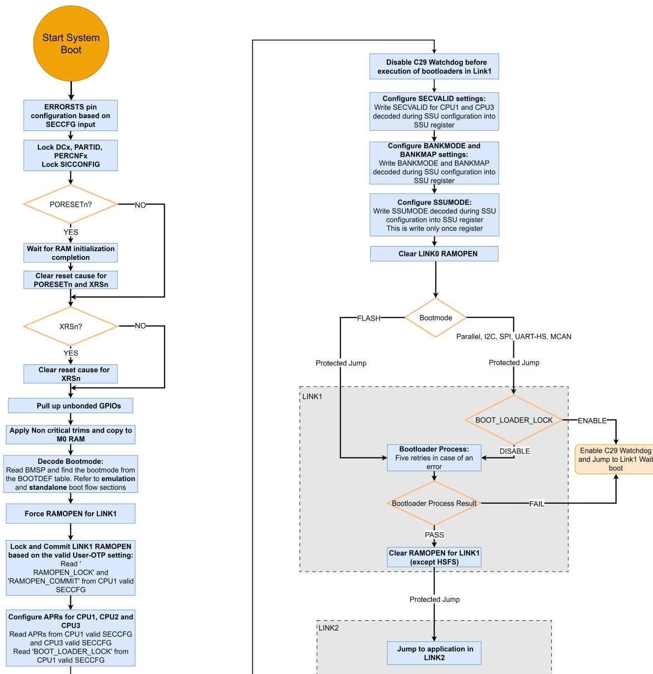
Figure 3-3. System Boot Flow to Application Code
