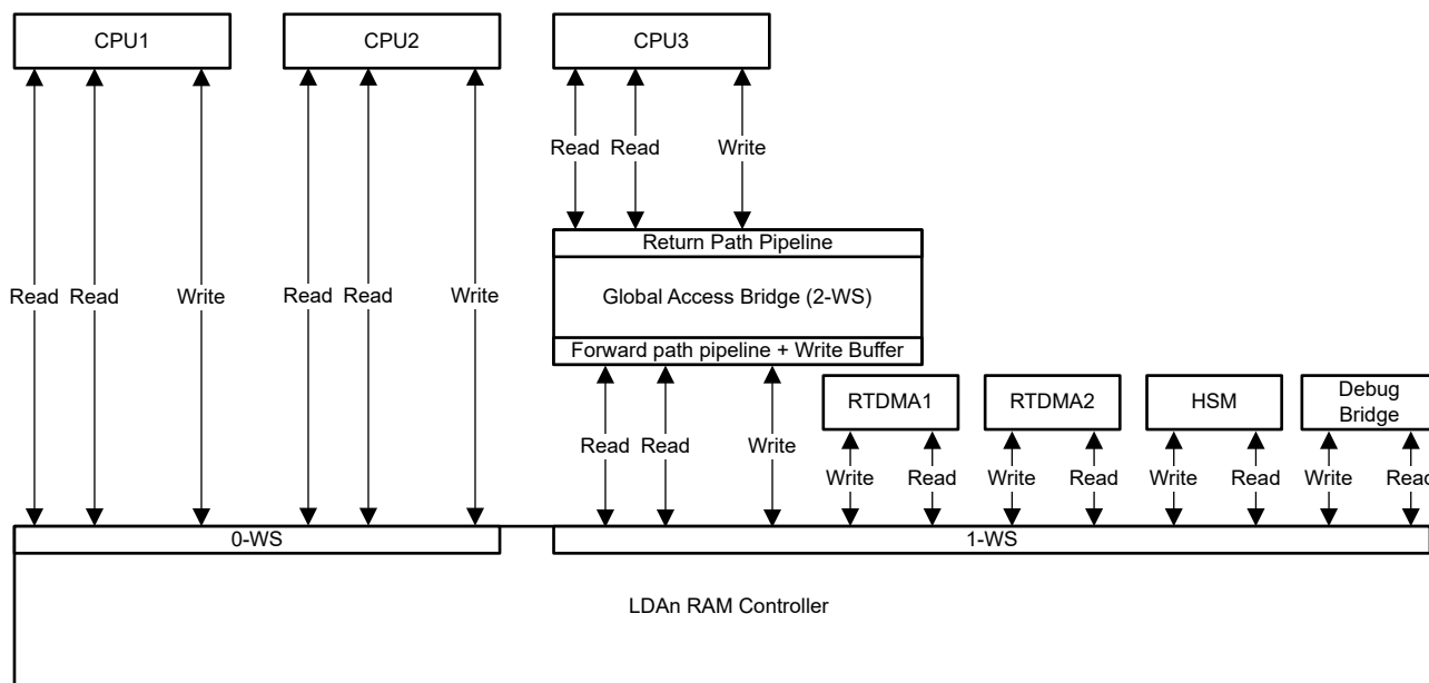
Figure 2-24. Global Access Bridge for LDAn RAMs
