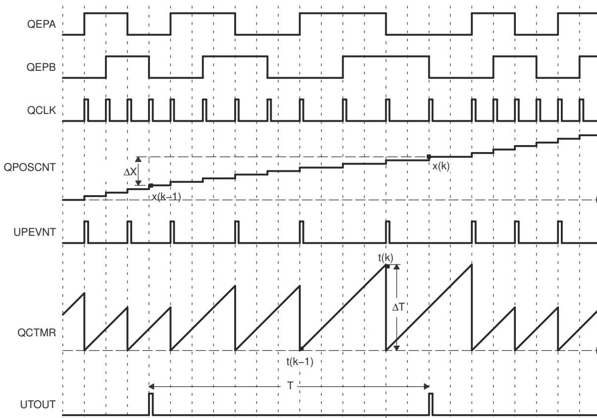
Figure 28-19. eQEP Edge Capture Unit - Timing Details
