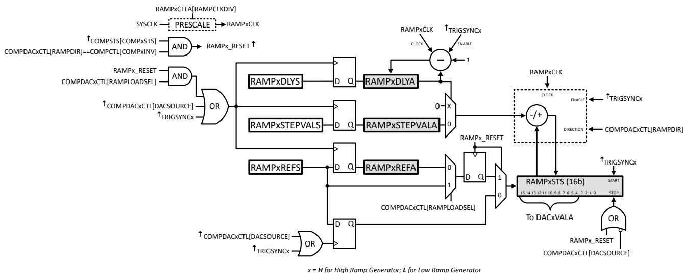
Figure 24-4. Ramp Generator Block Diagram
