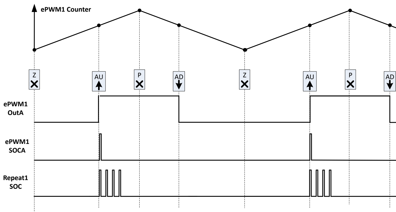
Figure 22-4. Oversampled ADC Trigger Example
