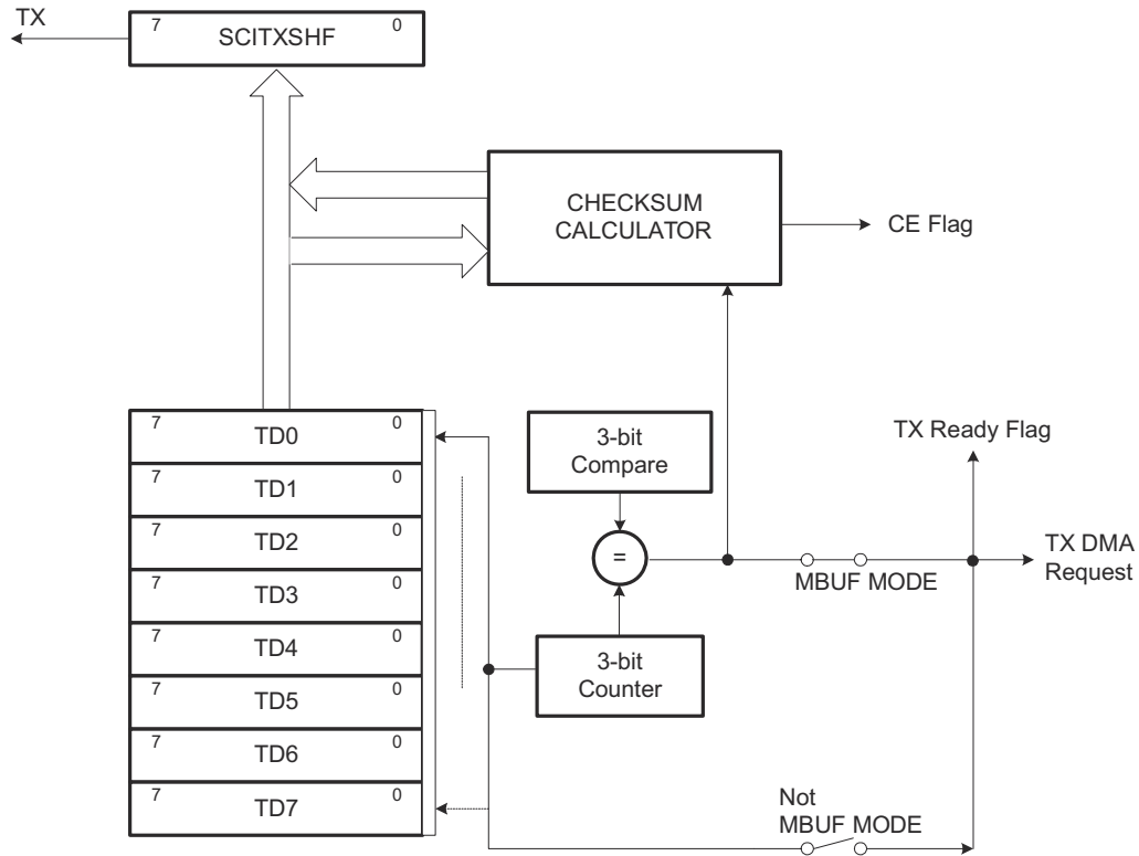
Figure 36-9. Transmit Buffers
