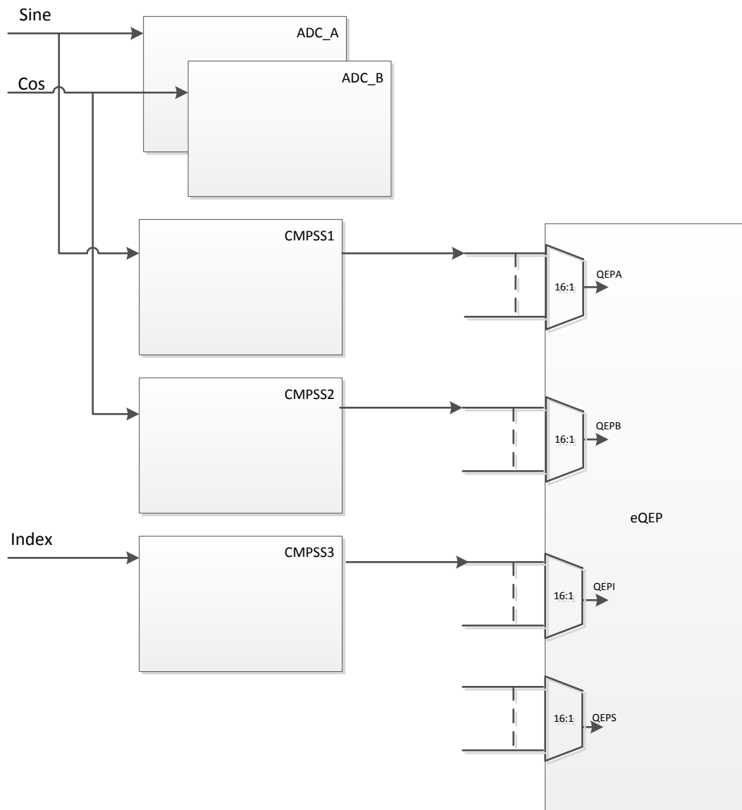
Figure 28-4. Using eQEP to Decode Signals from SinCos Transducer
