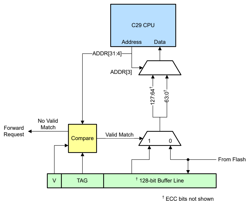
Figure 8-4. Flash Data Line Buffer for Single Bank
