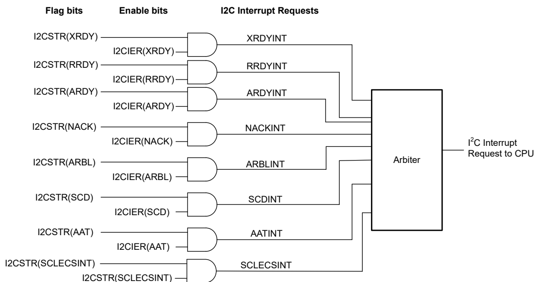
Figure 33-19. Enable Paths of the I2C Interrupt Requests
