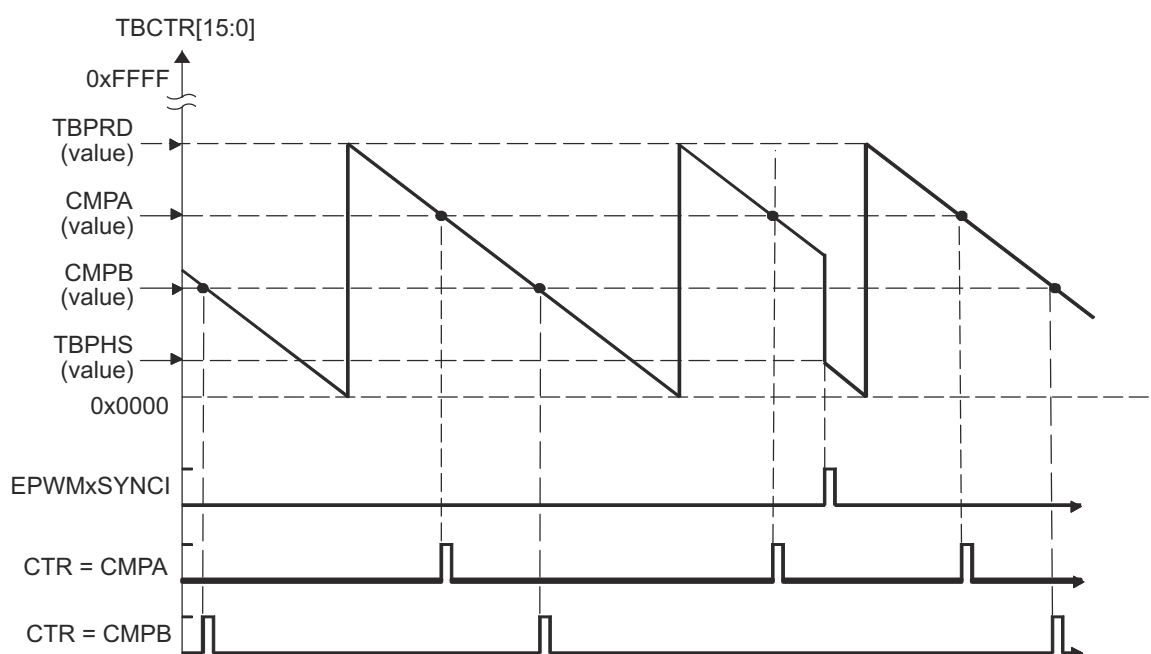
Figure 27-18. Counter-Compare Events in Down-Count Mode
