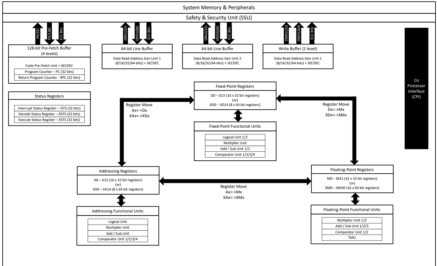
Figure 1-1. CPU Architecture Block Diagram
