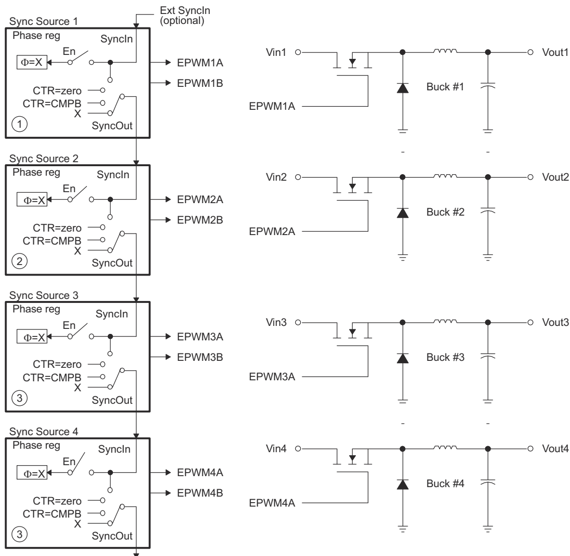
Figure 27-90. Control of Four Buck Stages. Here F_{PWM1} \neq F_{PWM2} \neq F_{PWM3} \neq F_{PWM4}
