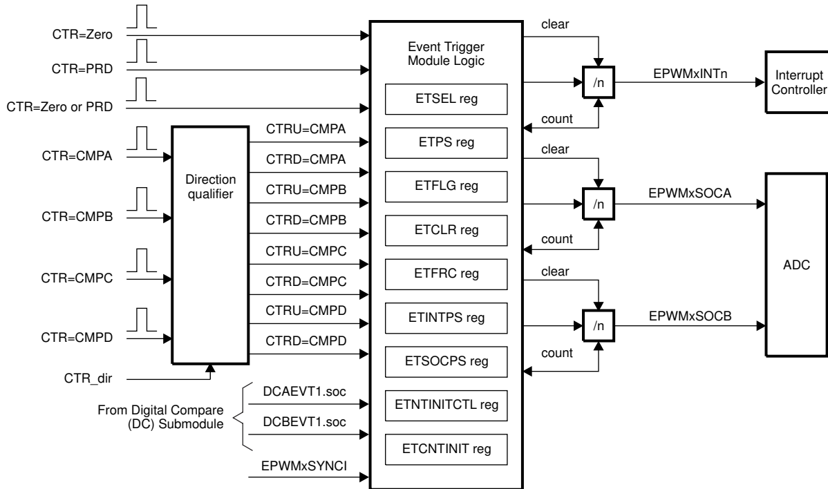
Figure 27-70. Event-Trigger Submodule Showing Event Inputs and Prescaled Outputs
