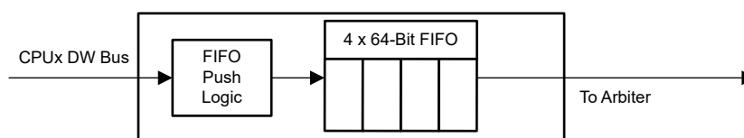
Figure 13-17. Write FIFO
