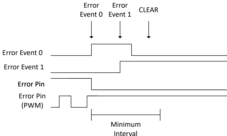
Figure 7-12. Error Pin Asserting with Interval Reset by Additional Error Event
