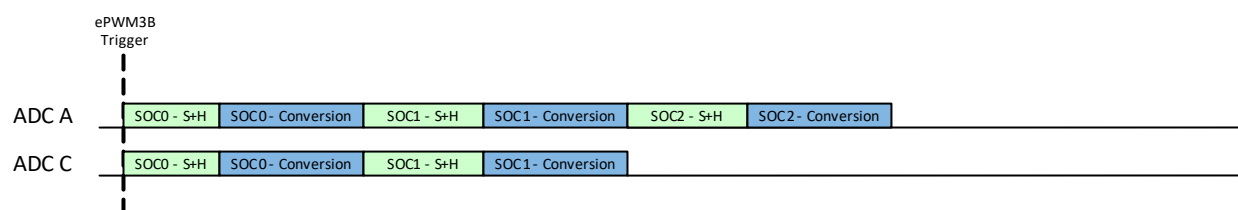
Figure 22-38. Example: Synchronous Operation with Uneven SOC Numbers
