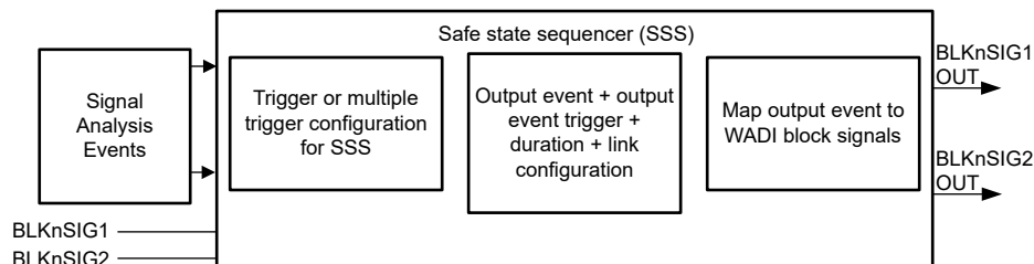
Figure 18-7. SSS High-Level Block Diagram
