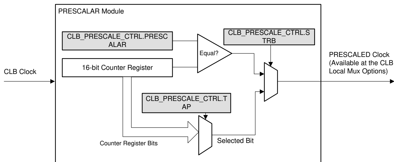
Figure 10-4. CLB Clock Prescalar
