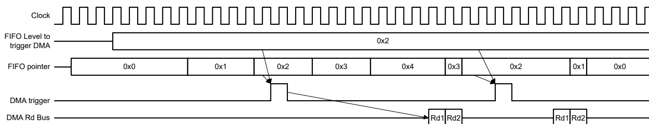
Figure 38-9. RTDMA Trigger Example
