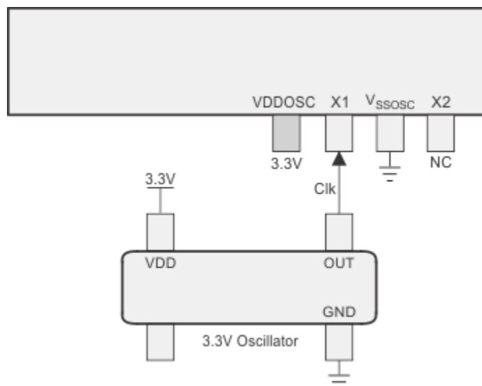
Figure 2-5. Single-ended 3.3V External Clock
