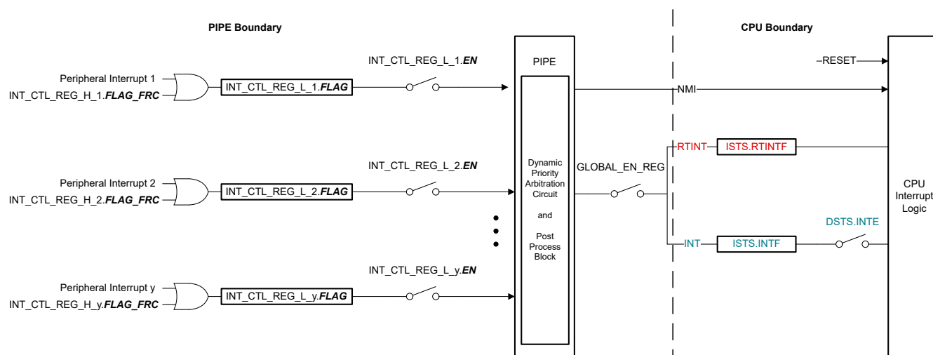
Figure 5-3. Interrupt Propagation
