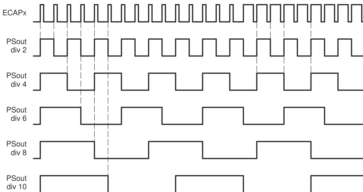
Figure 25-5. Prescale Function Waveforms
