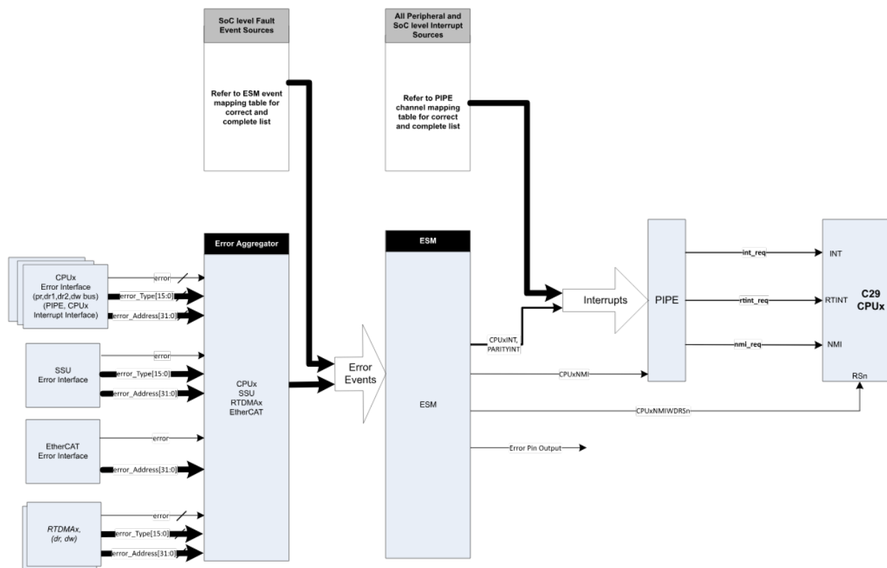
Figure 6-2. Error Propagation from Source to CPU
