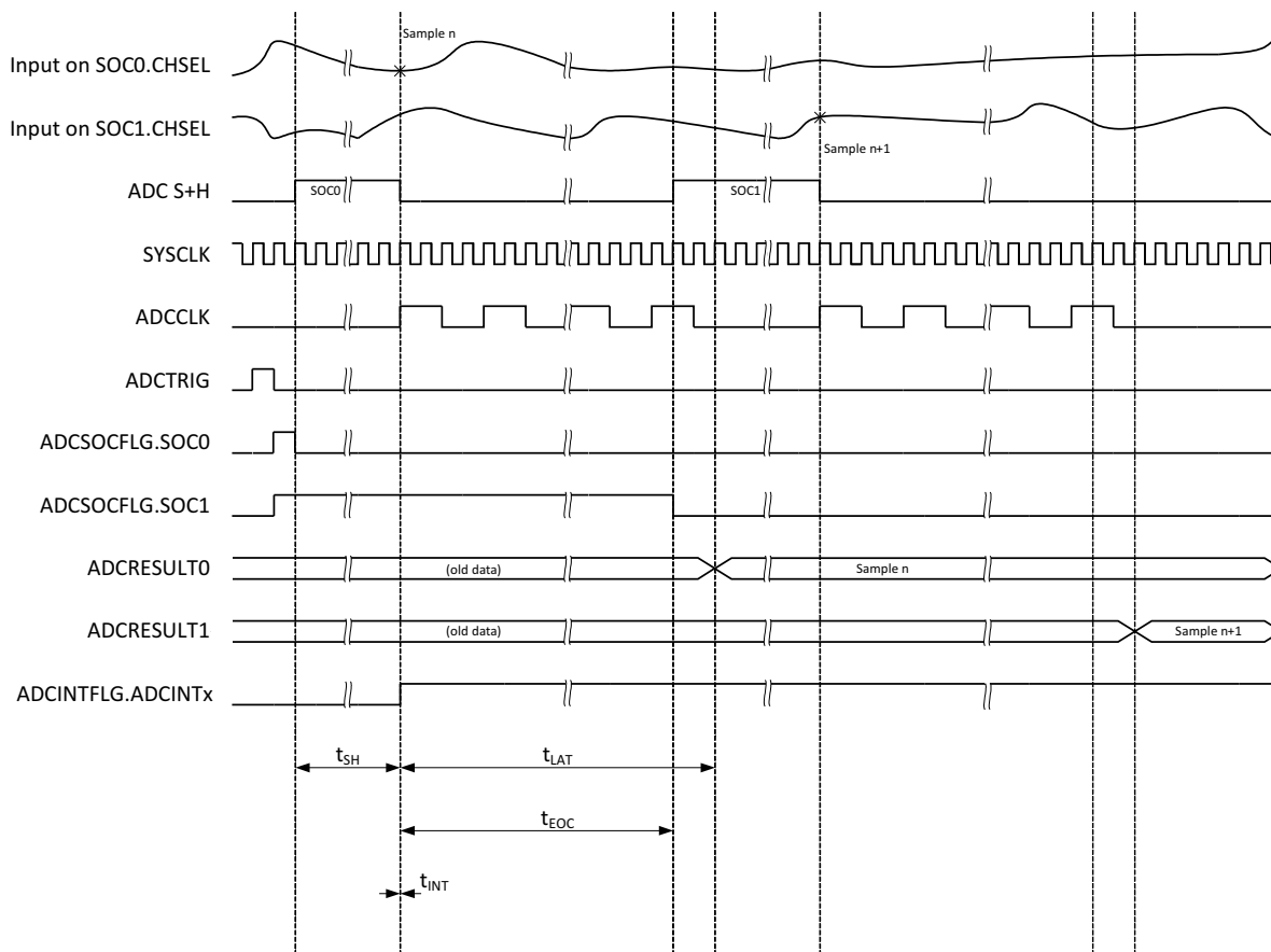
Figure 22-32. ADC Timings for 12-bit Mode in Early Interrupt Mode
