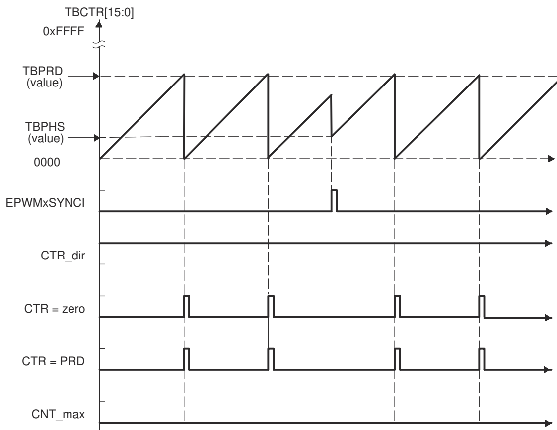
Figure 27-9. Time-Base Up-Count Mode Waveforms
