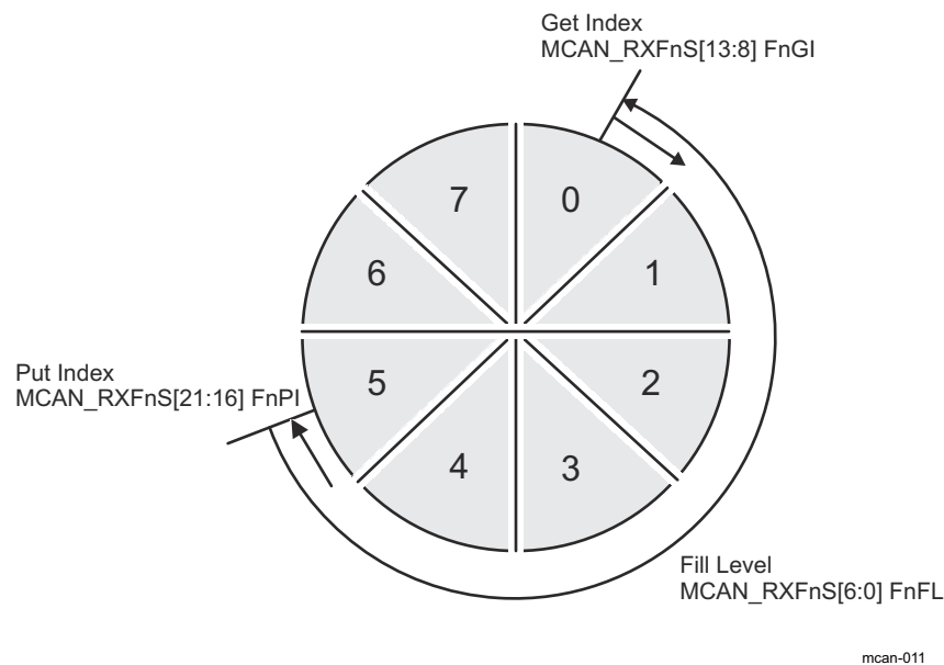
Figure 30-15. Rx FIFO Status
