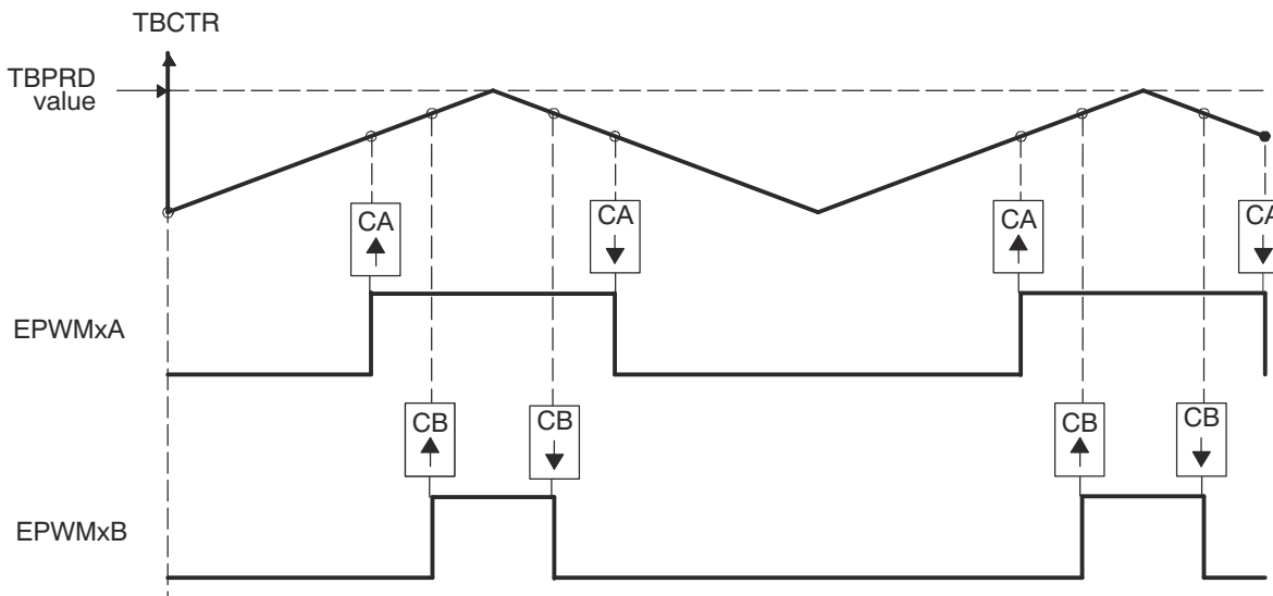
Figure 27-29. Up-Count, Pulse Placement Asymmetric Waveform With Independent Modulation on EPWMxA
