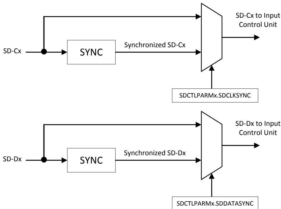
Figure 29-4. Input Qualification on SD-Cx and SD-Dx
