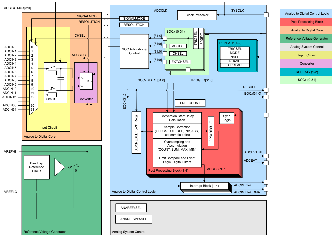
Figure 22-1. ADC Module Block Diagram
