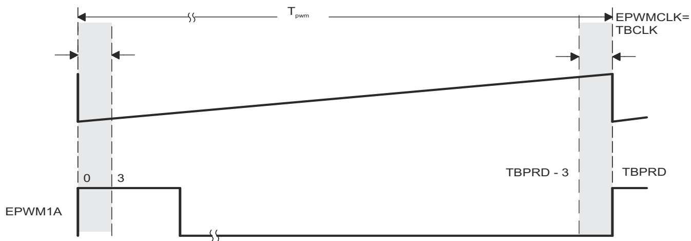
Figure 27-116. Up-Count Duty Cycle Range Limitation Example (HRPCTL[HRPE] = 1)
