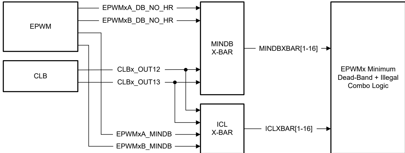
Figure 19-2. MINDB and ICL X-BAR
