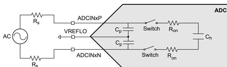
Figure 22-12. Differential Input Model
