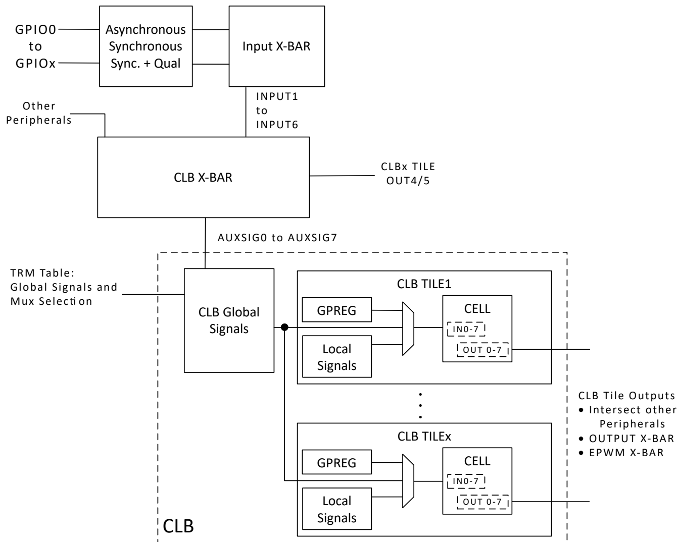
Figure 10-5. GPIO to CLB Tile Connections
