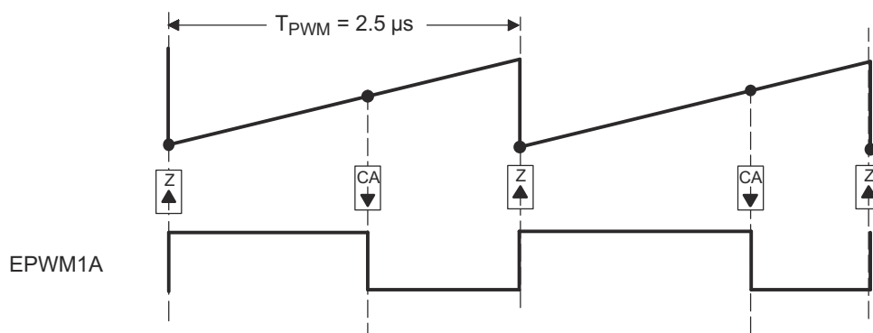
Figure 27-121. PWM Waveform Generated for the PWM DAC Function
