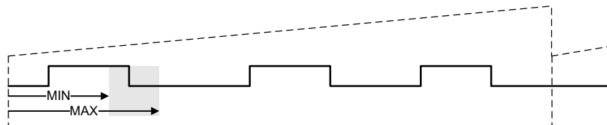
Figure 27-82. MIN, MAX Settings and Window for Capture Event Detection
