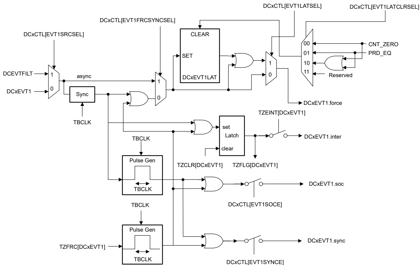
Figure 27-76. DCxEVT1 Event Triggering
