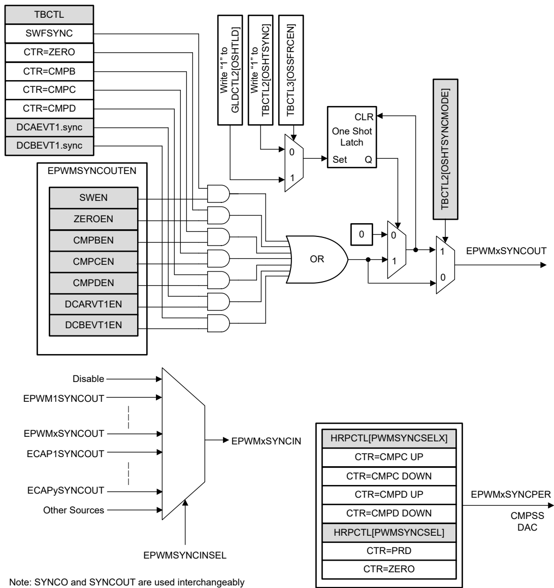
Figure 27-7. Time-Base Counter Synchronization Scheme
