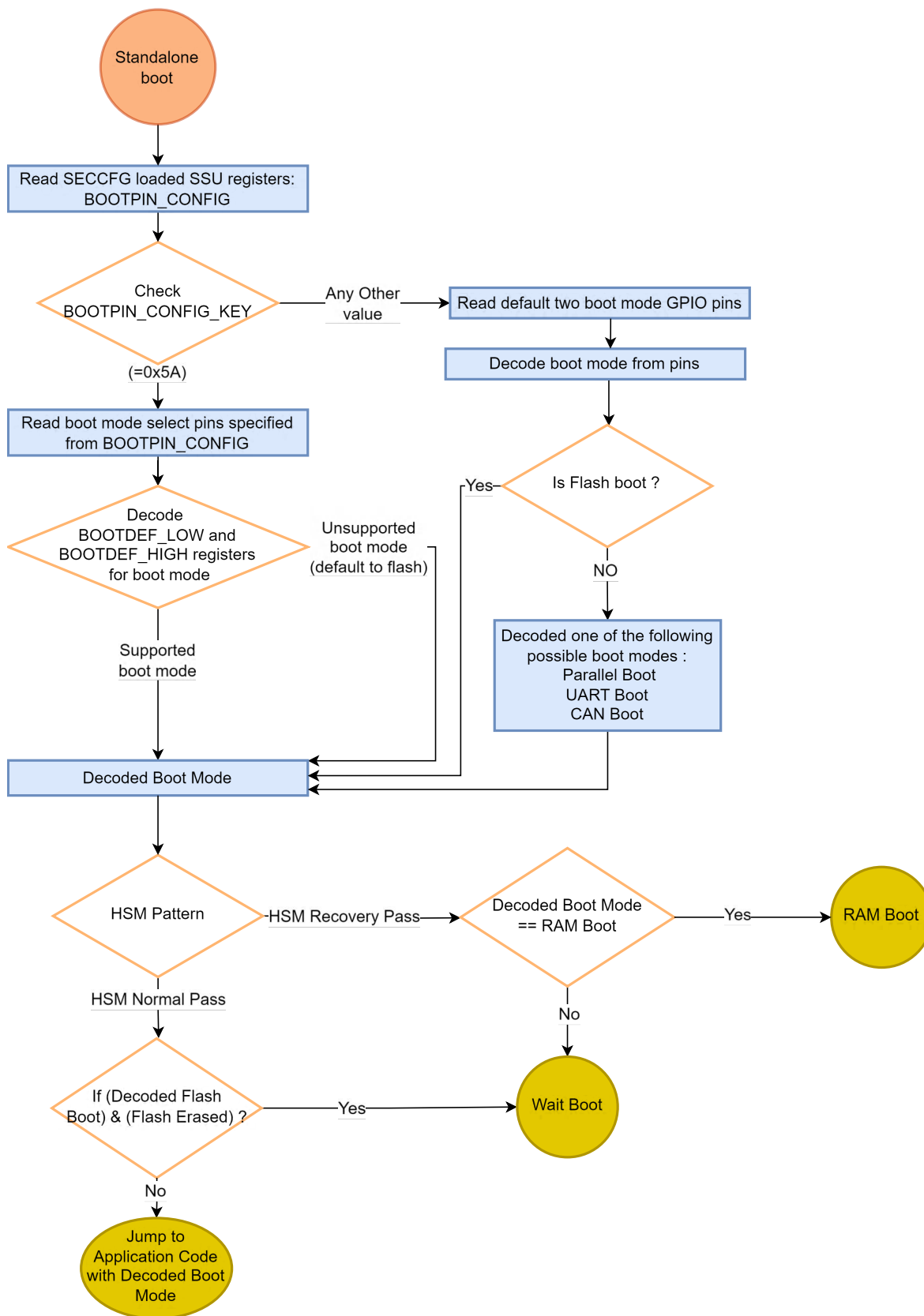
Figure 3-5. Standalone Boot Flow
