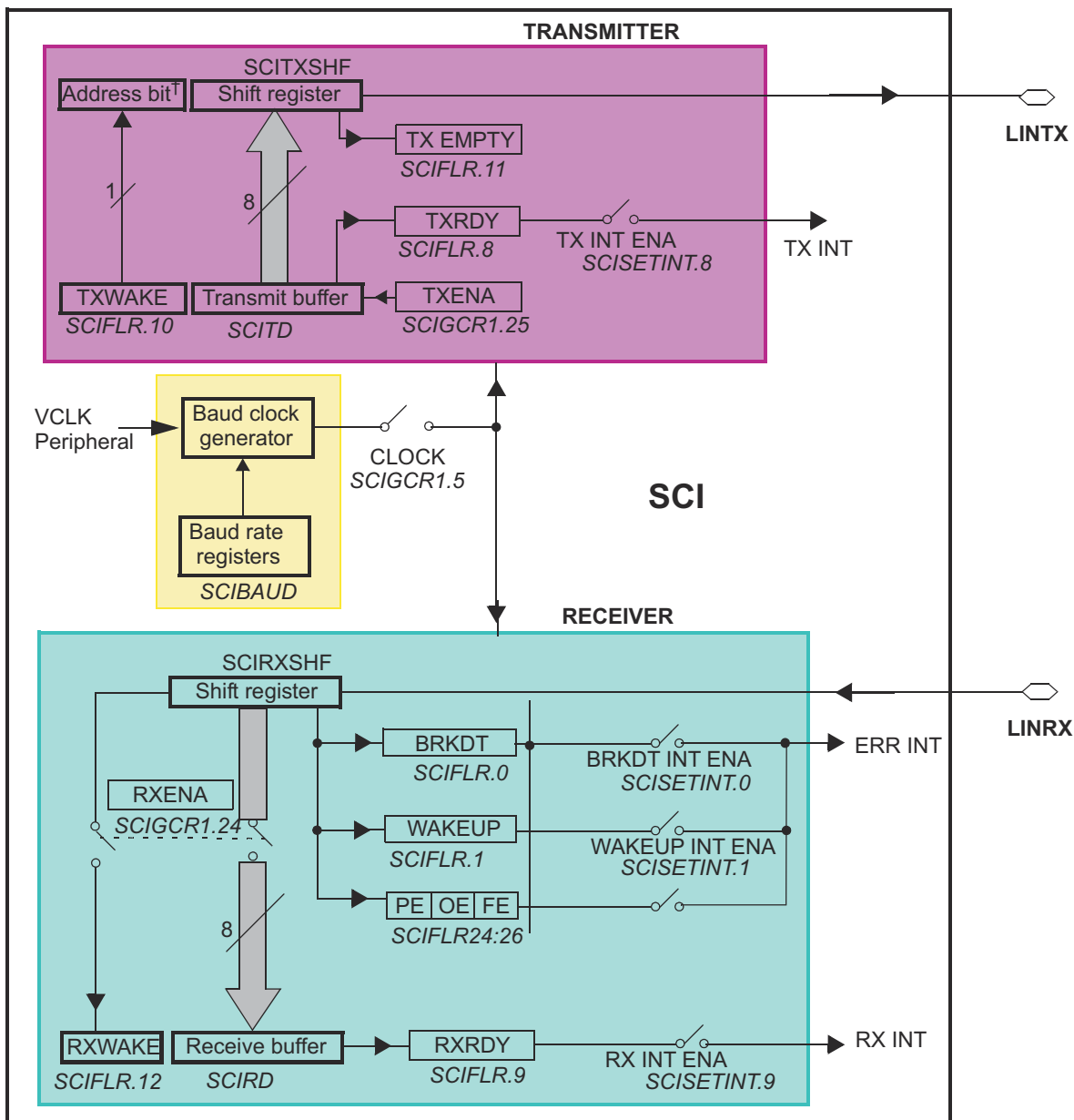
Figure 36-1. SCI Block
