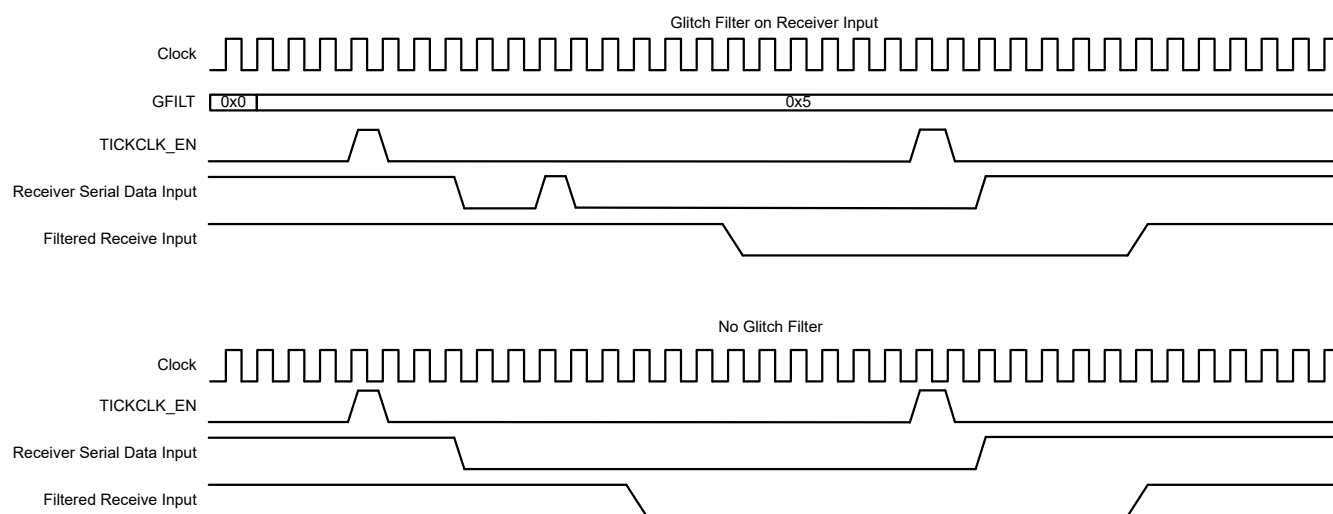
Figure 38-12. Glitch Filter Examples
