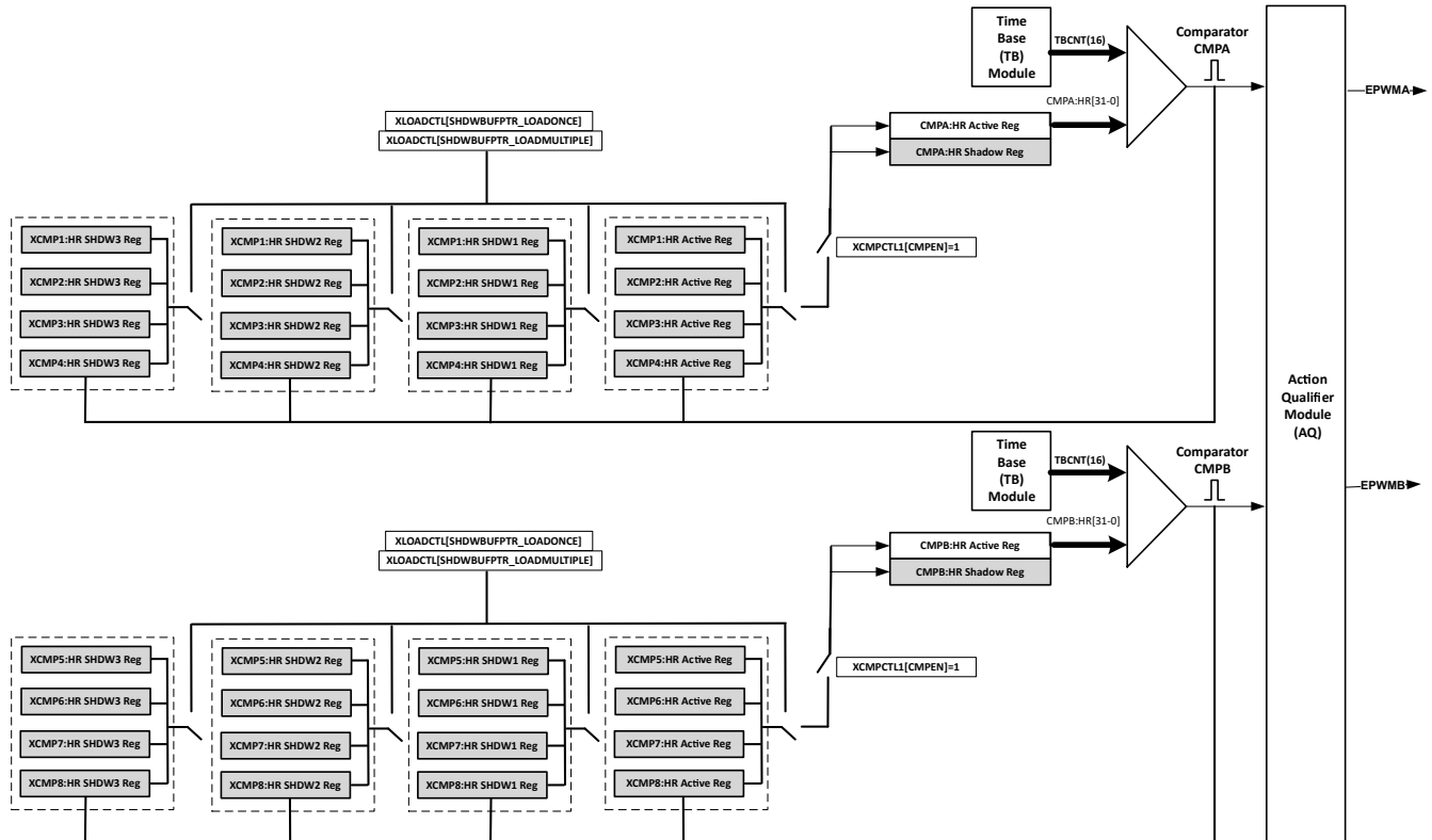
Figure 27-35. XCMP1-4 Allocated to CMPA and XCMP5-8 Allocated to CMPB
