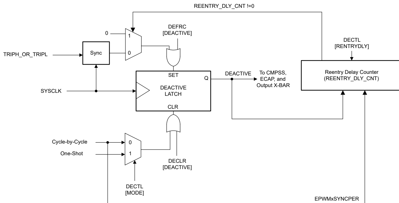
Figure 27-54. DEACTIVE Flag Functionality
