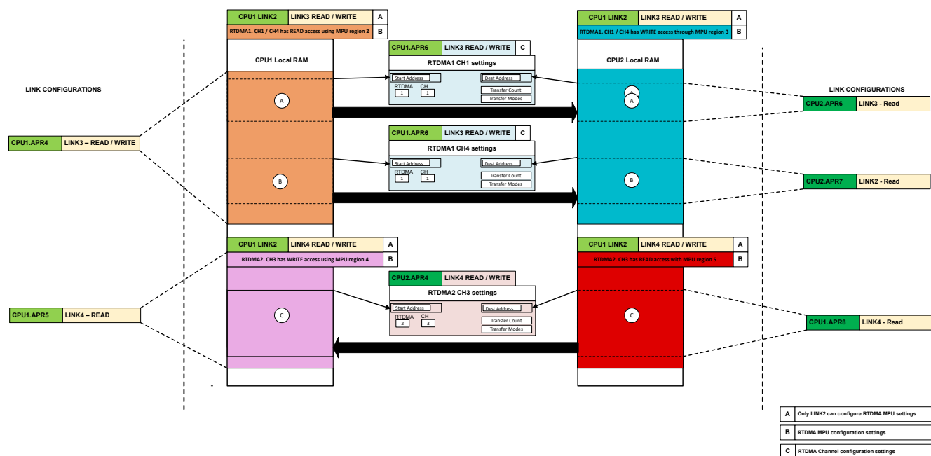
Figure 12-9. Memory-to-Memory Transfer Example
