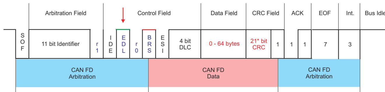
Figure 30-5. CAN FD Frame
