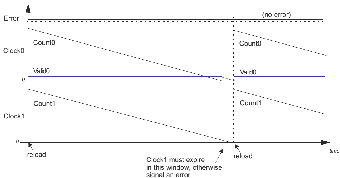
Figure 11-3. Counter Relationship
