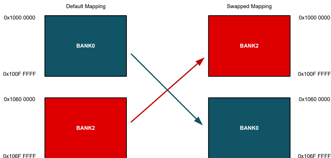
Figure 9-5. Bank Swap Mapping Example
