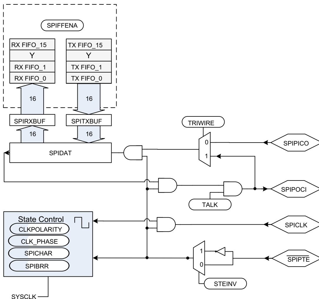
Figure 37-6. SPI Module Peripheral Configuration
