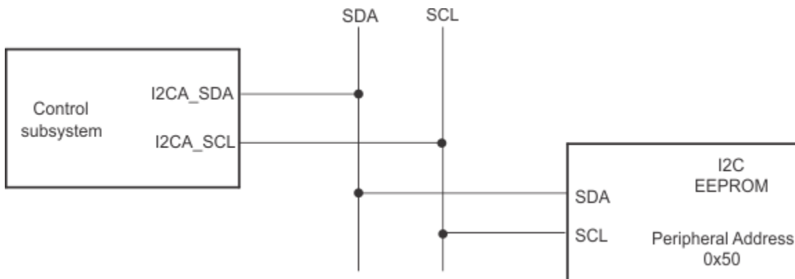
Figure 3-7. EEPROM Device at Address 0x50
