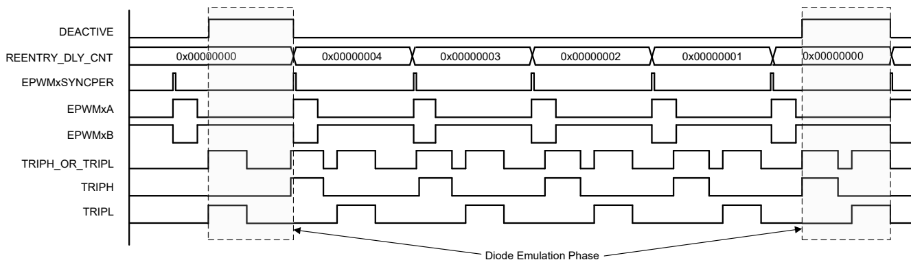
Figure 27-57. DE Mode Reentry Sequence
