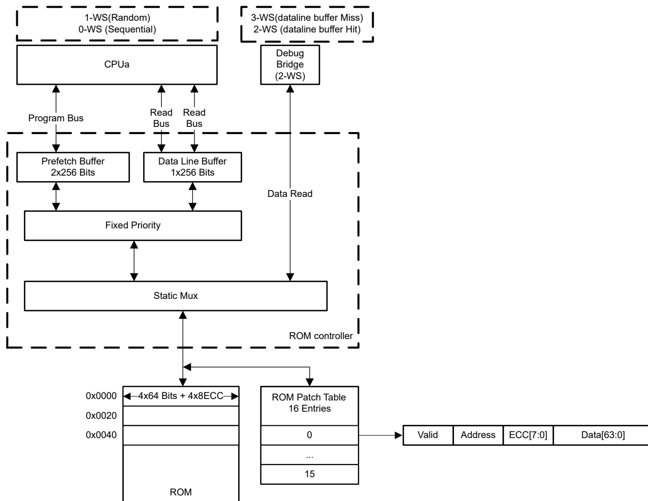
Figure 2-27. ROM Controller
