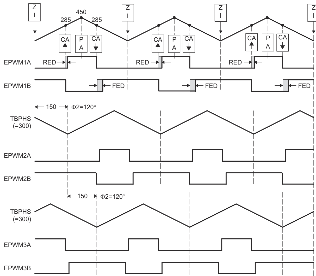
Figure 27-101. 3-Phase Interleaved DC/DC Converter Waveforms for Control of 3-Phase Interleaved DC/DC Converter
