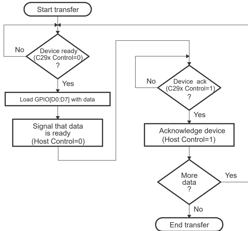
Figure 3-10. Parallel GPIO Mode - Host Transfer Flow
