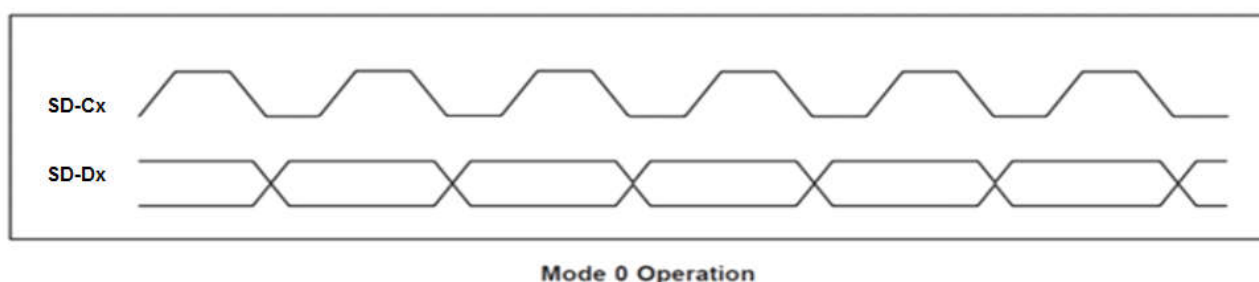
Figure 29-5. Different Modulator Modes Supported
