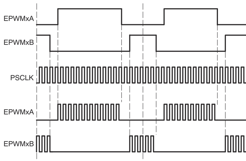
Figure 27-45. Simple PWM Chopper Submodule Waveforms Showing Chopping Action Only
