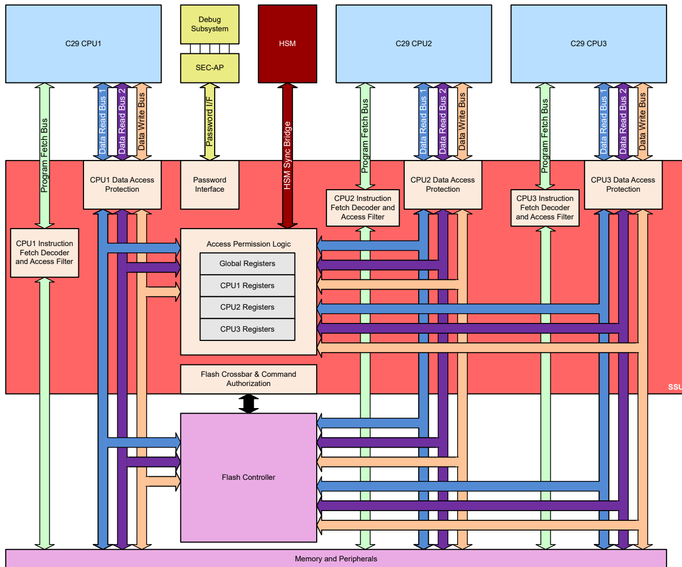
Figure 9-1. Real-Time Security Architectural Block Diagram
