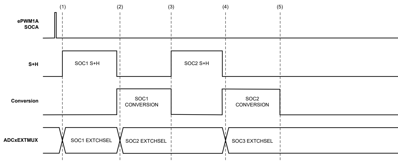
Figure 22-16. ADC External Channel Timing Example in Preselect Mode
