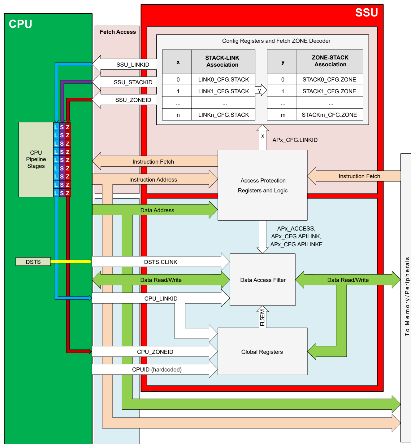
Figure 9-4. SSU-CPU Tightly Coupled Interface
