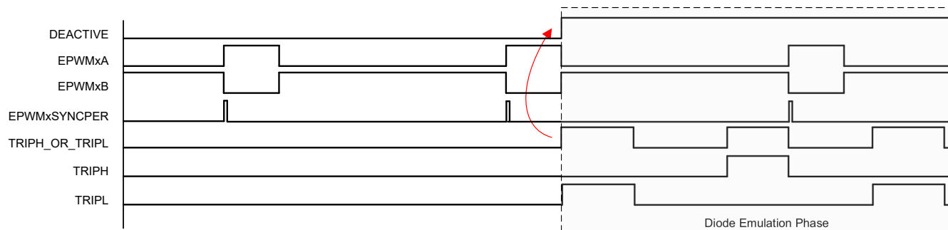
Figure 27-55. Example Timing Sequence Illustrating DE Mode Entry
