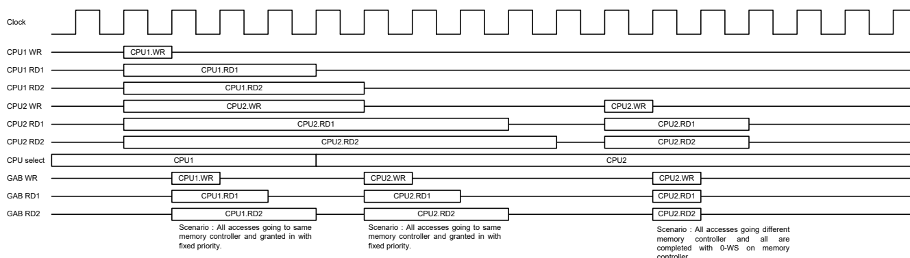
Figure 2-25. Global Access Bridge Arbitration
