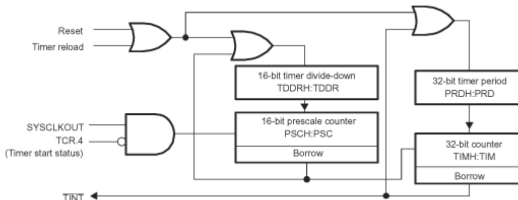
Figure 2-12. CPU Timers
