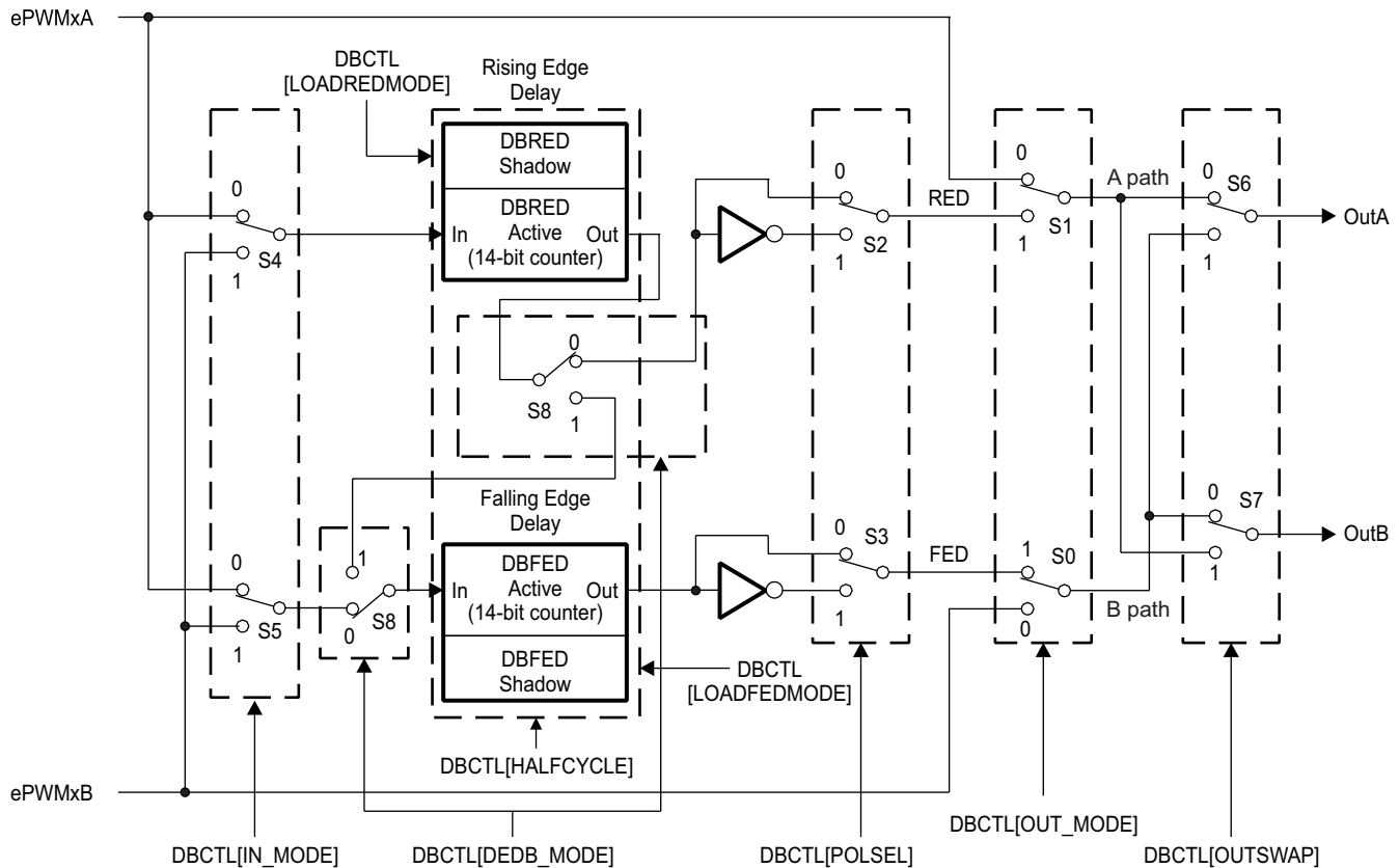
Figure 27-41. Configuration Options for the Dead-Band Submodule
