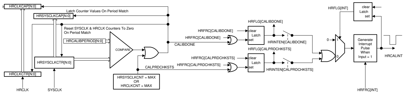
Figure 26-2. HRCAP Calibration
