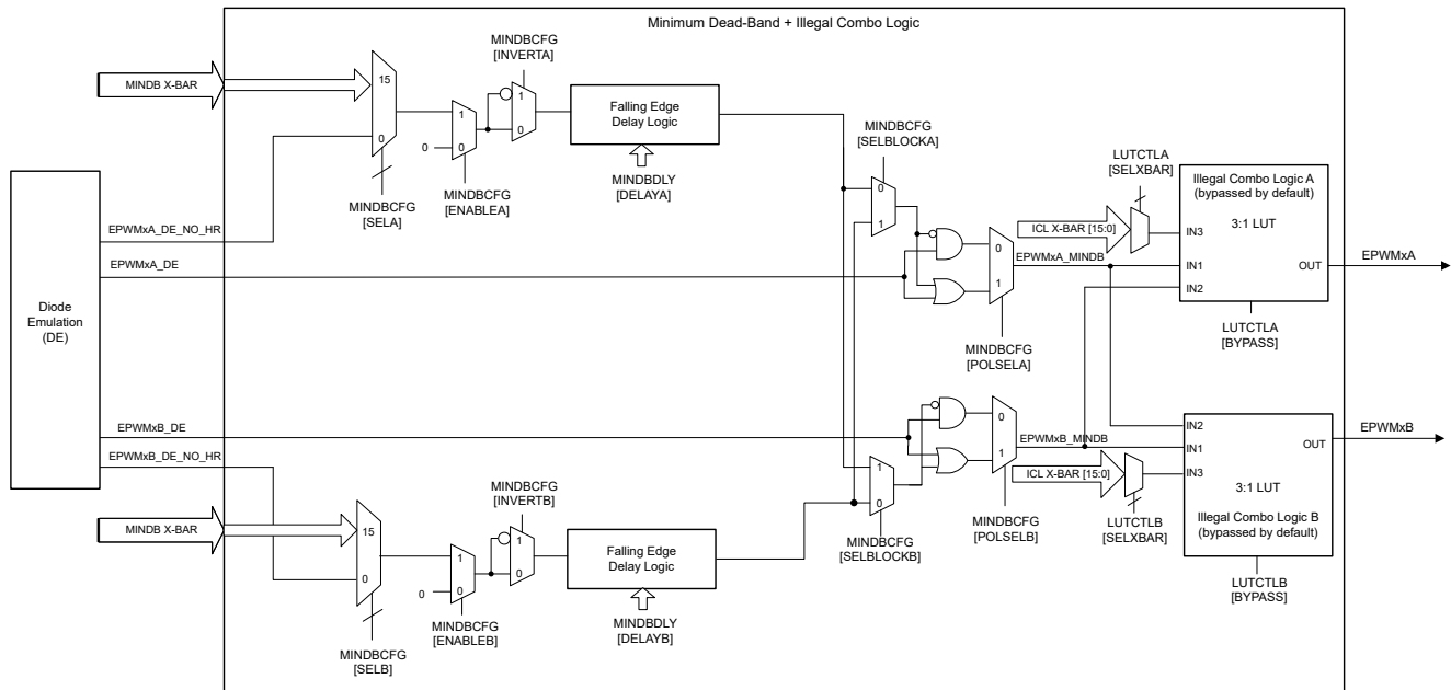
Figure 27-62. Minimum Dead-Band and Illegal Combo Logic Block Diagram
