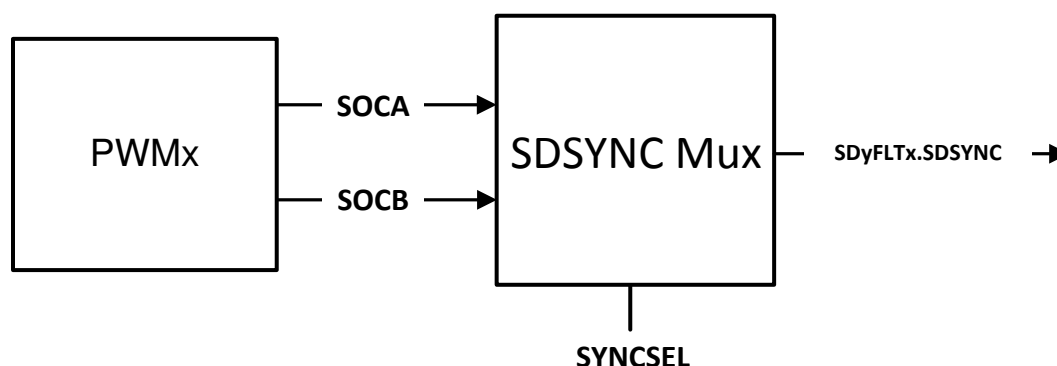
Figure 29-10. SDSYNC Event
