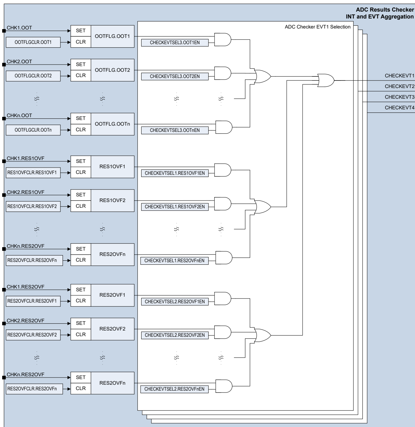
Figure 22-29. ADC Result Checker Event Aggregation
