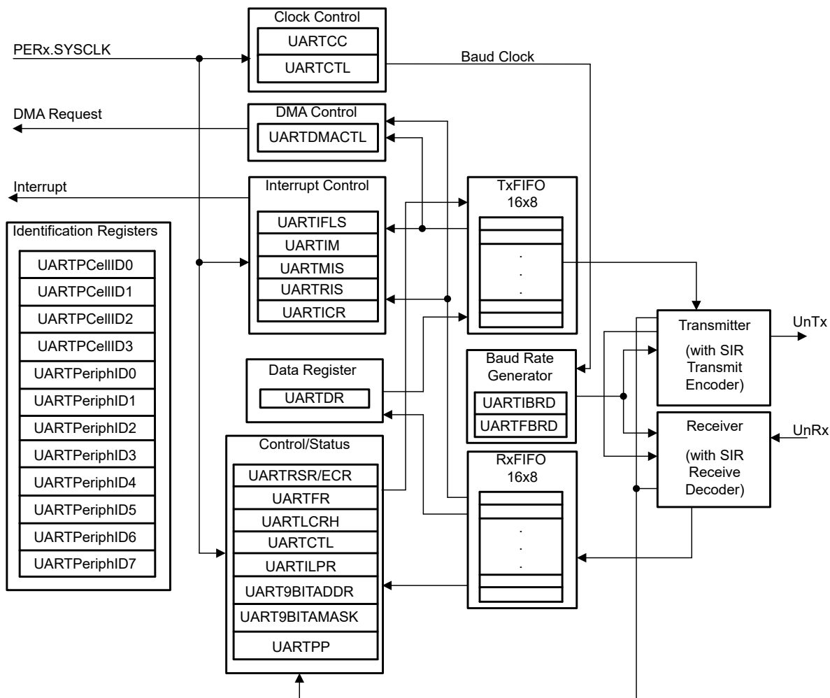
Figure 35-1. UART Module Block Diagram
