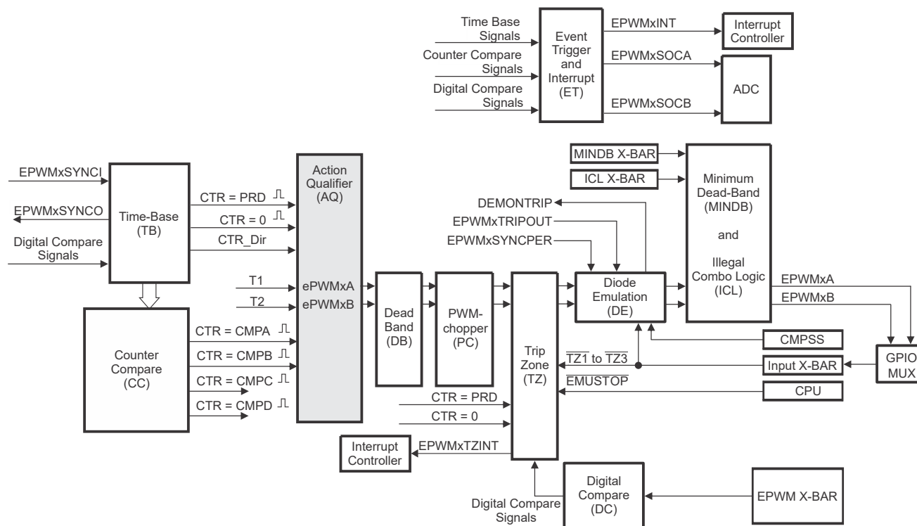
Figure 27-21. Action-Qualifier Submodule
