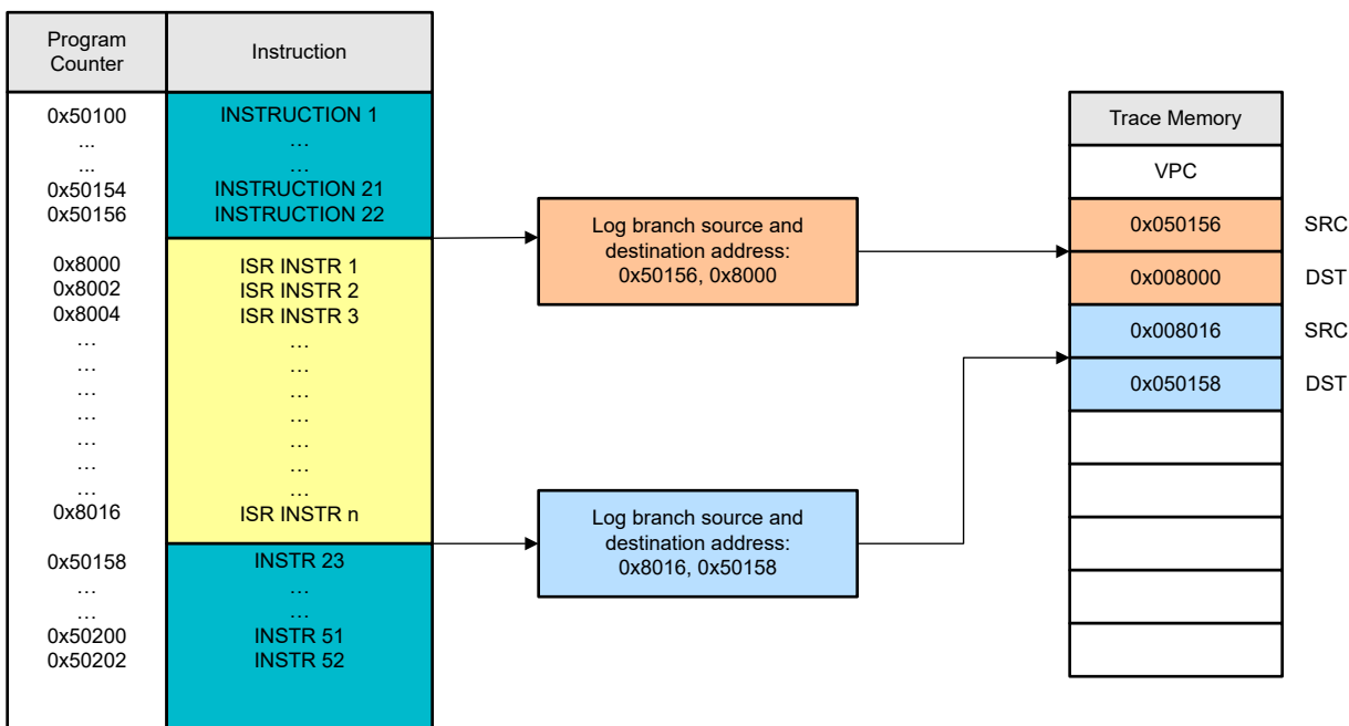
Figure 16-4. PC Trace Operation
