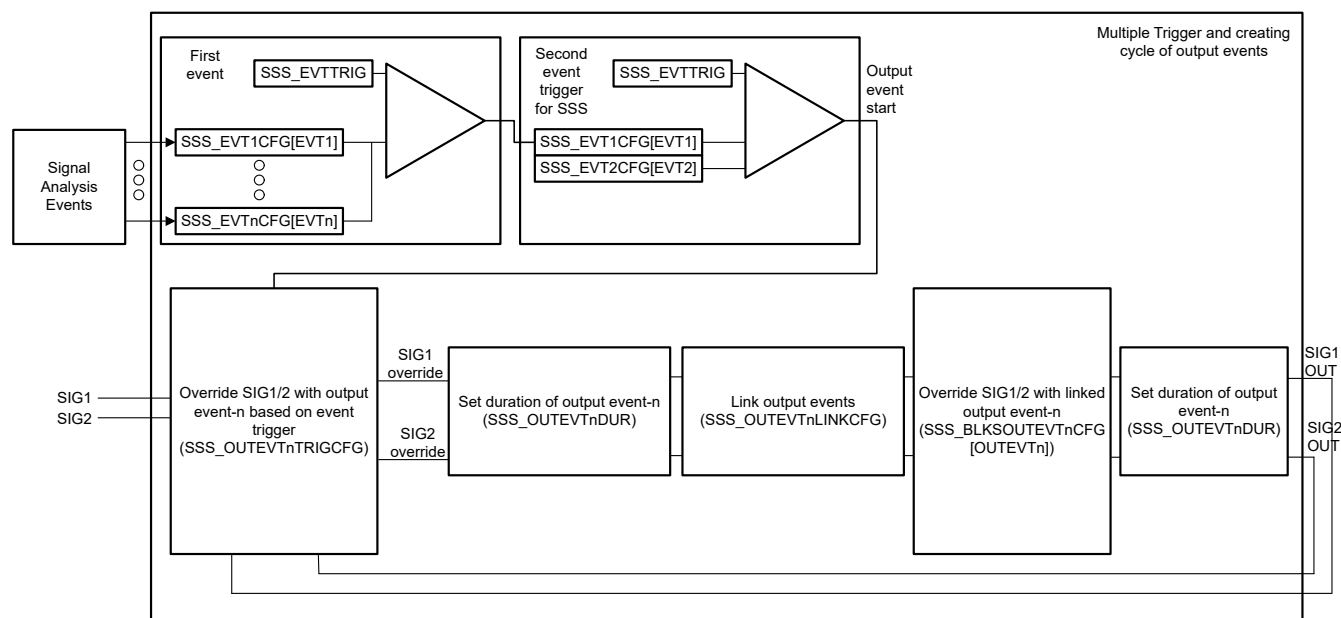
Figure 18-12. Multiple Trigger with Cyclic Pattern Output Events
