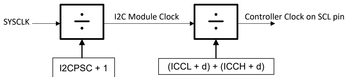
Figure 33-3. Clocking Diagram for the I2C Module
