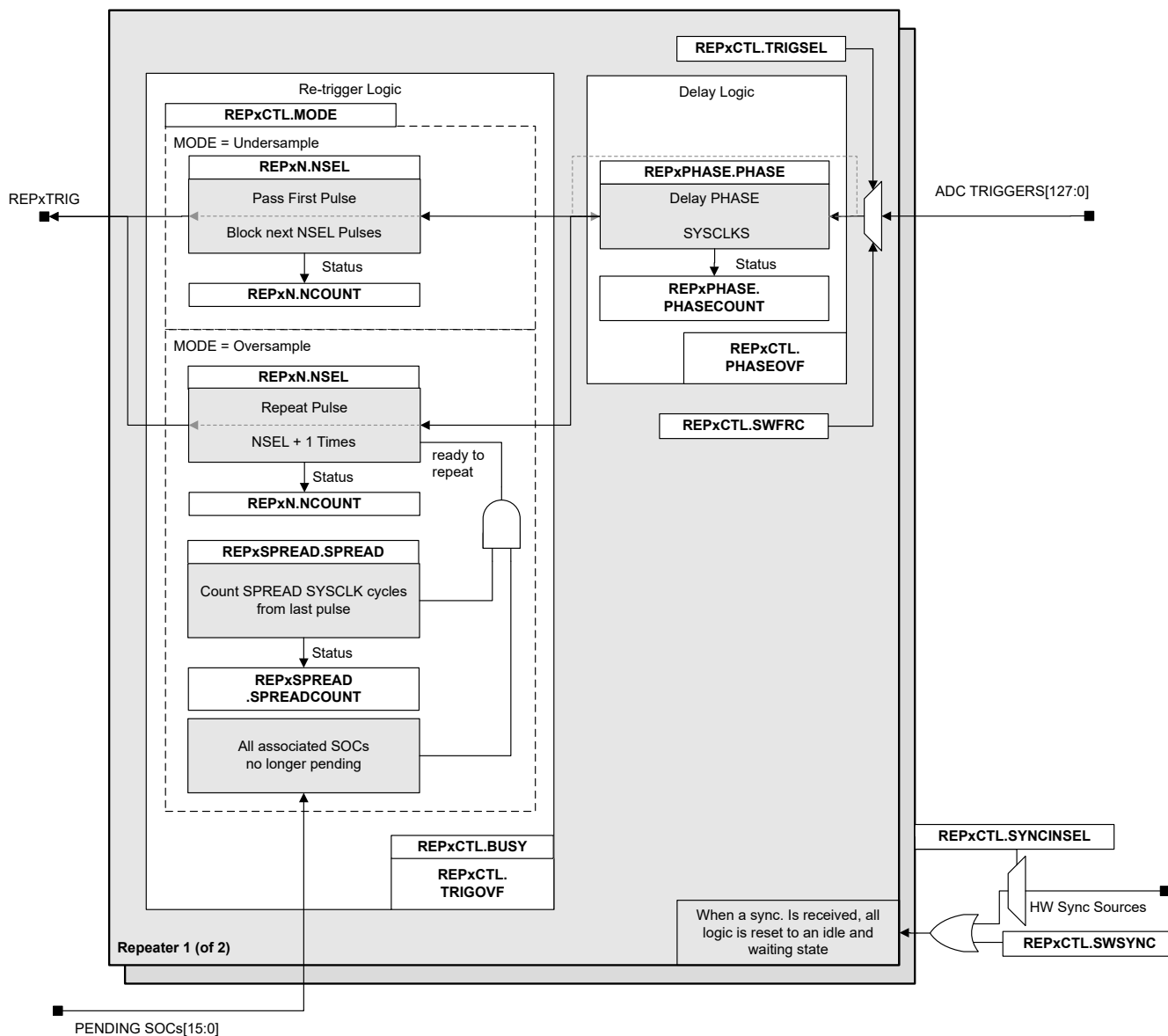
Figure 22-3. ADC Trigger Repeater Block Diagram
