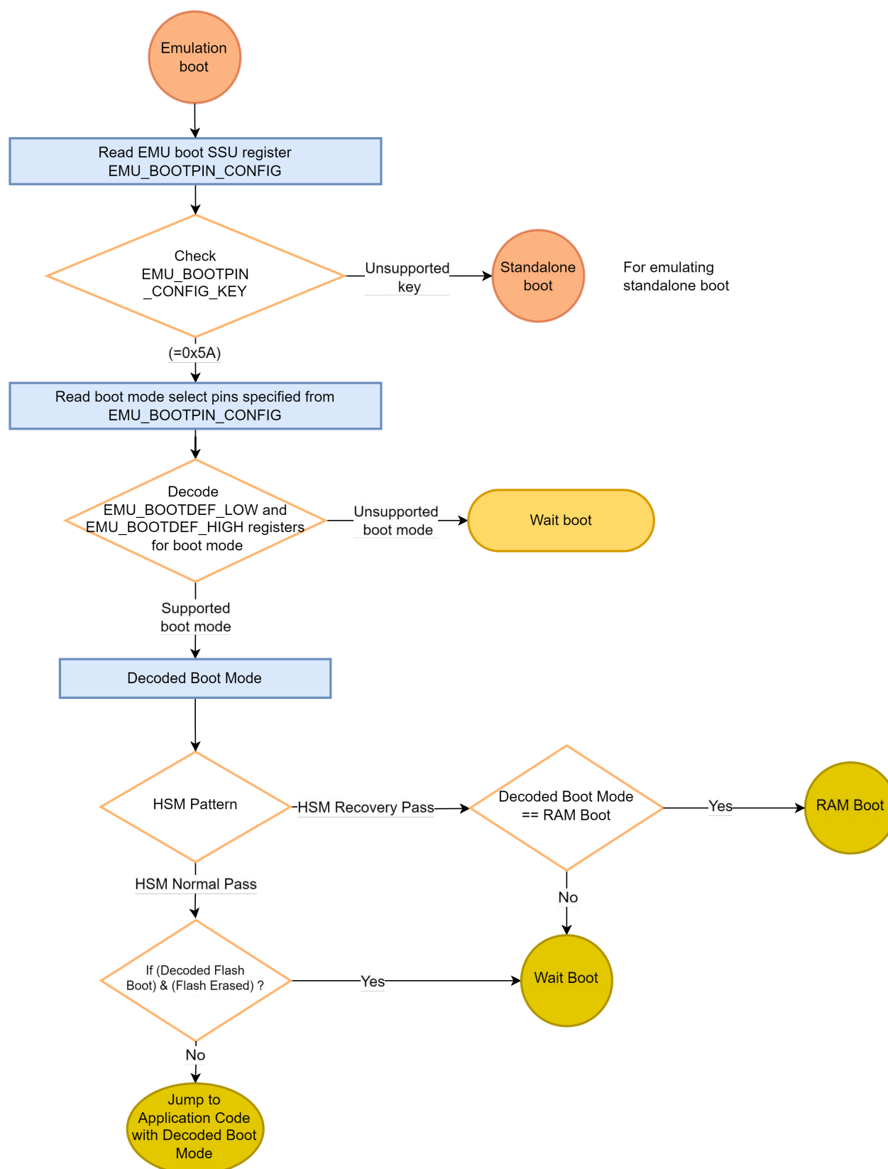
Figure 3-4. Emulation Boot Flow
