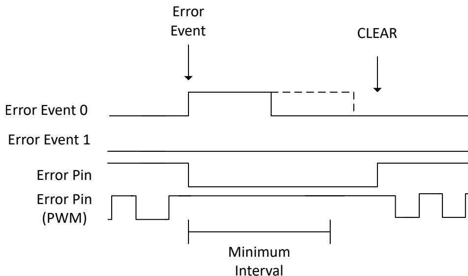
Figure 7-11. Error Pin Asserting with CLEAR after Minimum Interval
