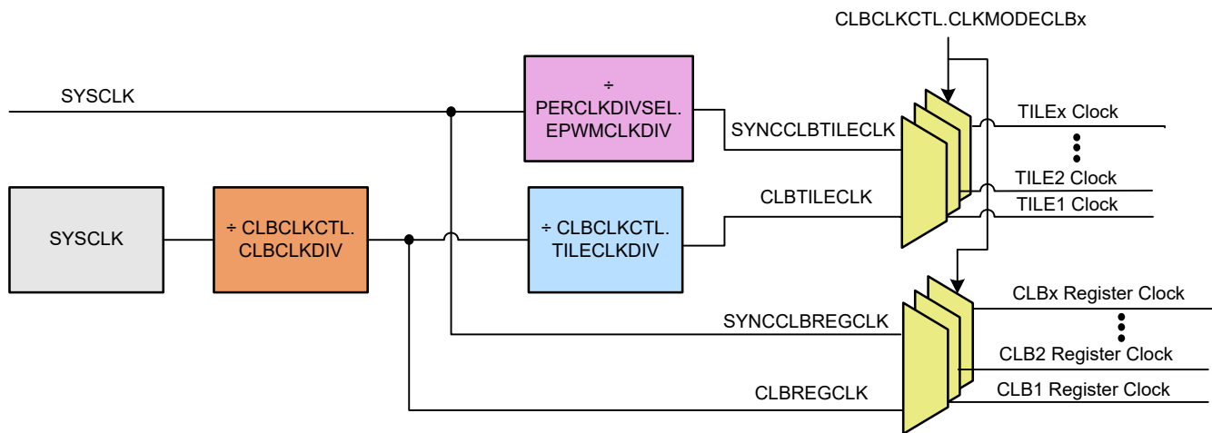
Figure 10-3. CLB Clocking
