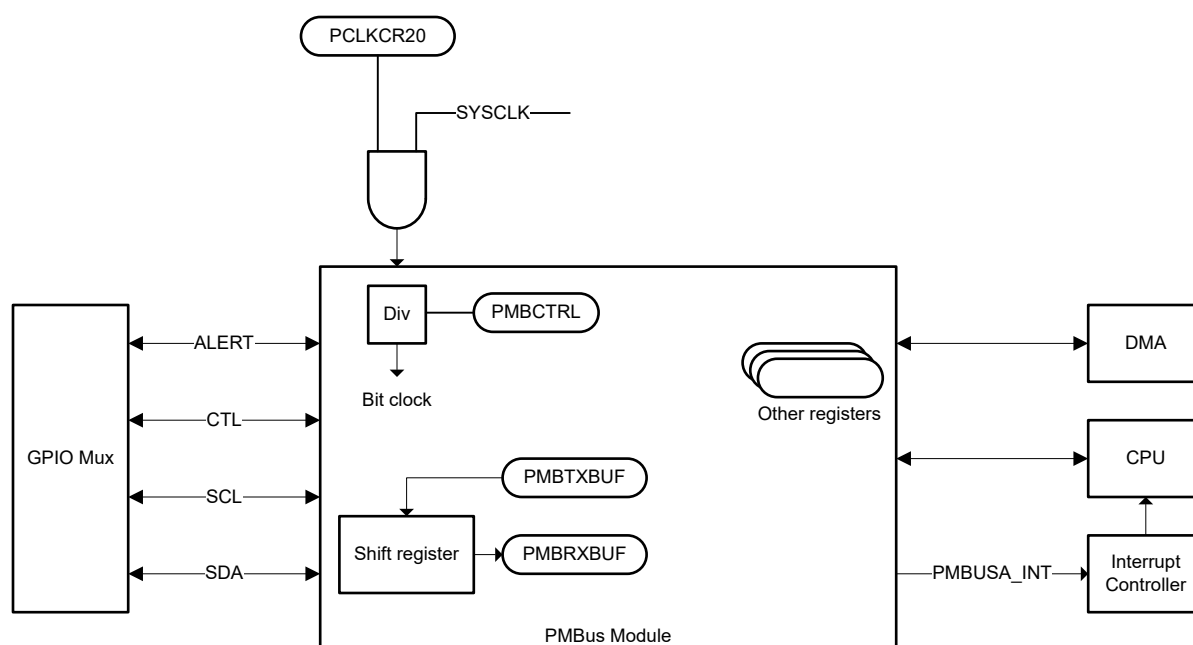
Figure 34-1. PMBus Module Block Diagram
