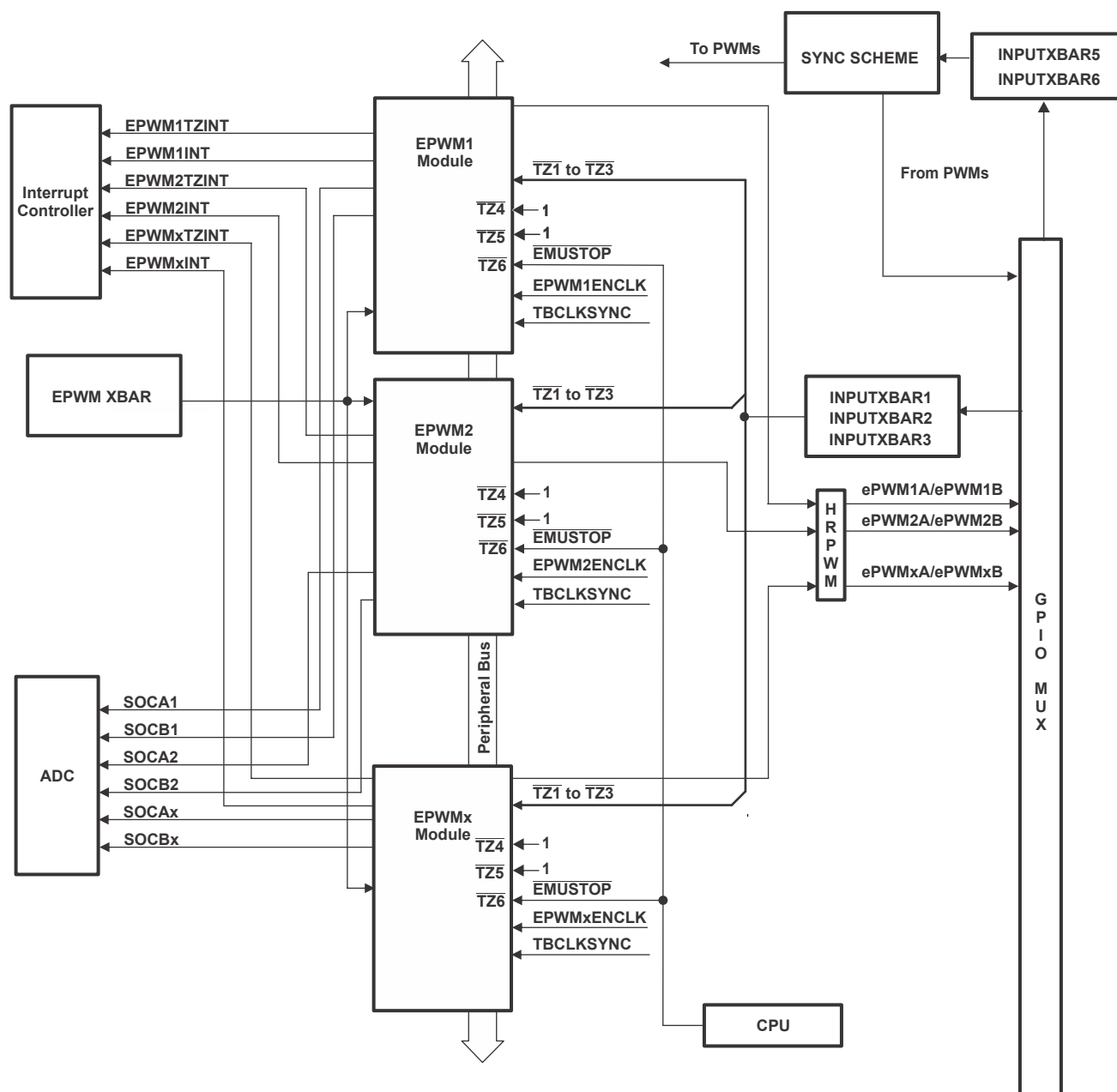
Figure 27-1. Multiple ePWM Modules
