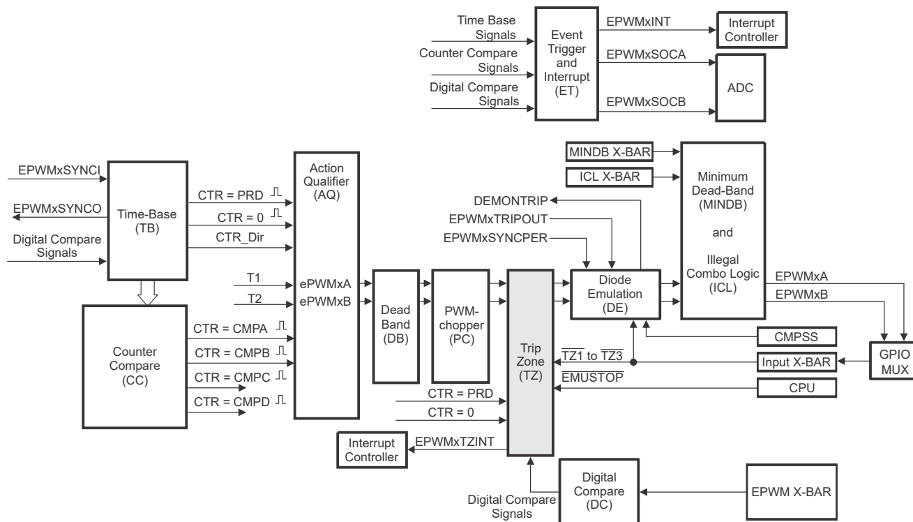
Figure 27-48. Trip-Zone Submodule
