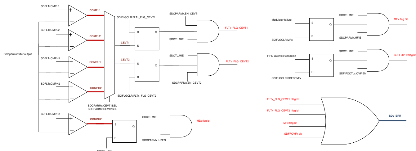
Figure 29-13. SDFM Error (SDy_ERR) Interrupt Sources
