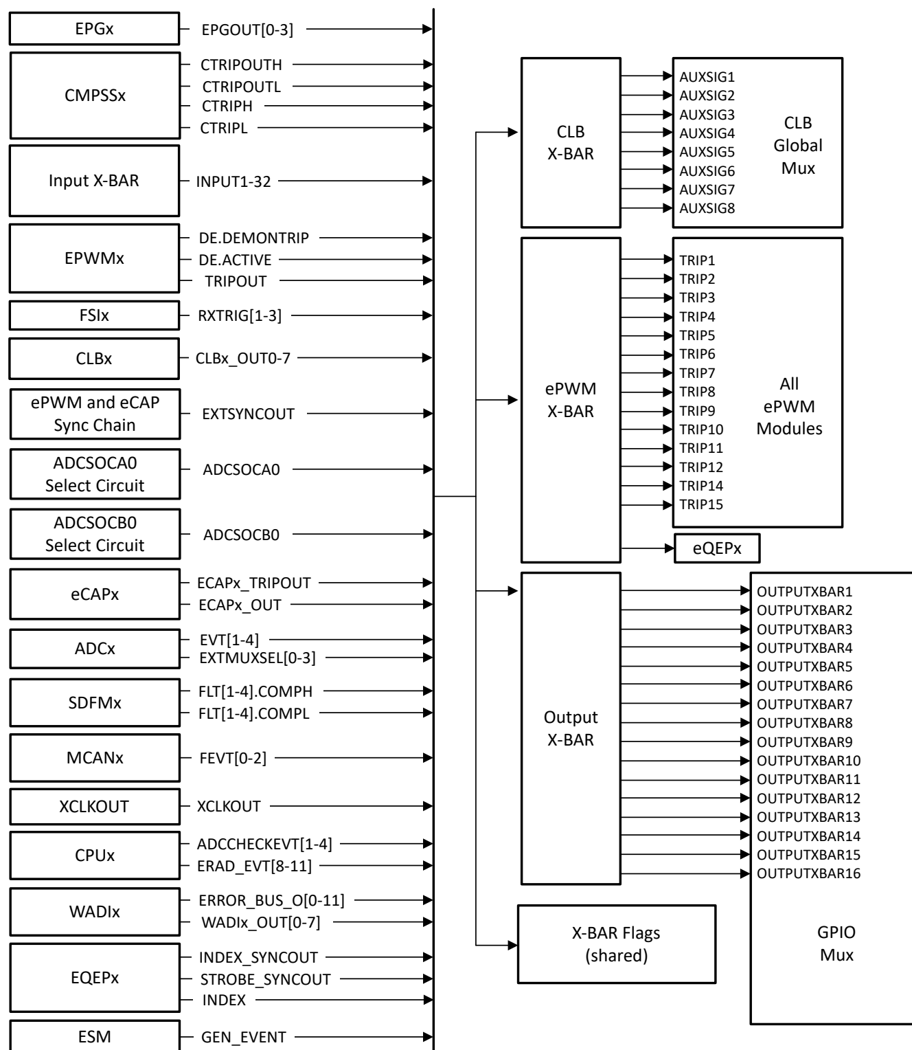
Figure 19-7. X-BAR Input Sources
