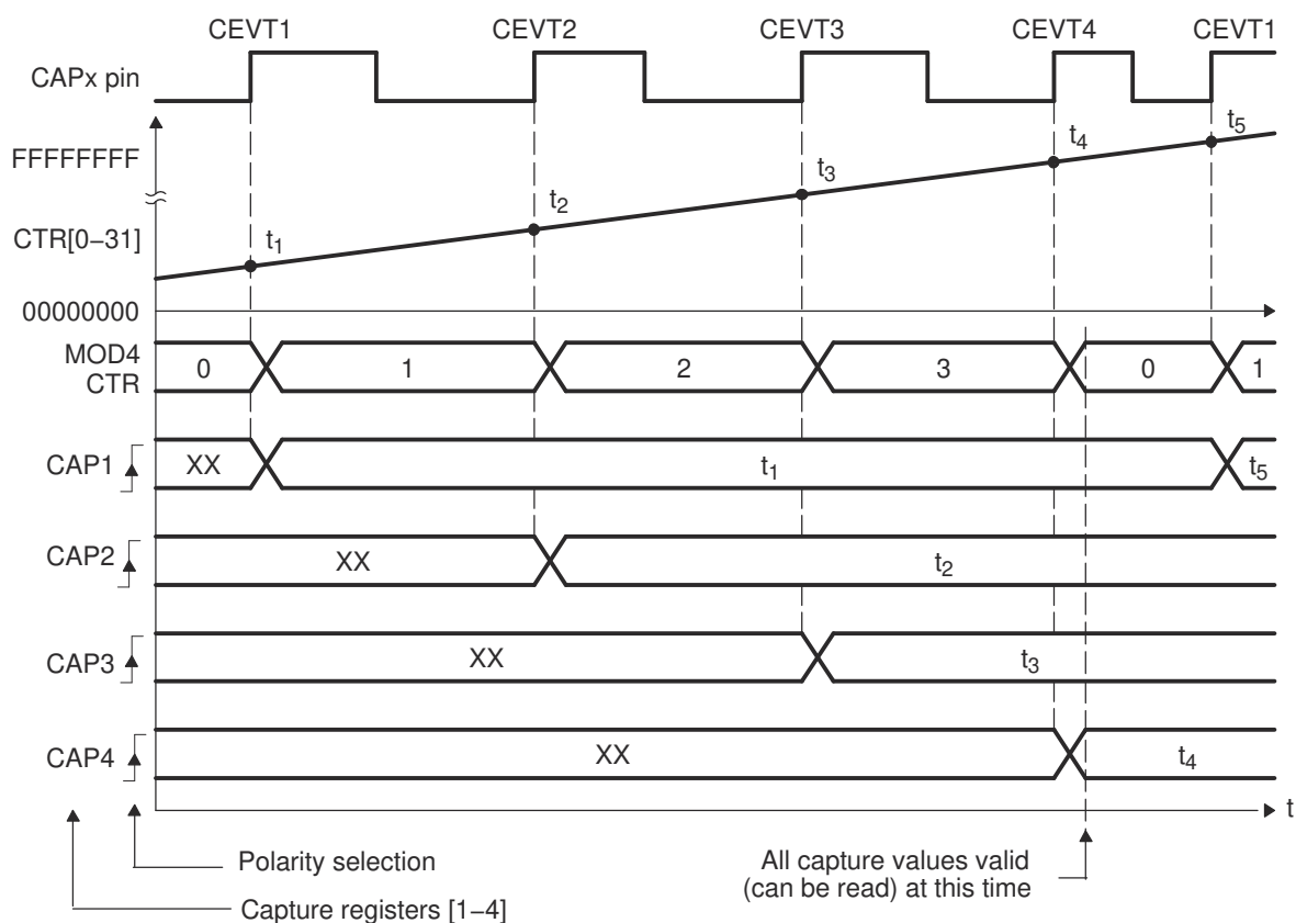
Figure 25-14. Capture Sequence for Absolute Time-stamp and Rising-Edge Detect
