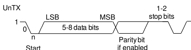
Figure 35-2. UART Character Frame
