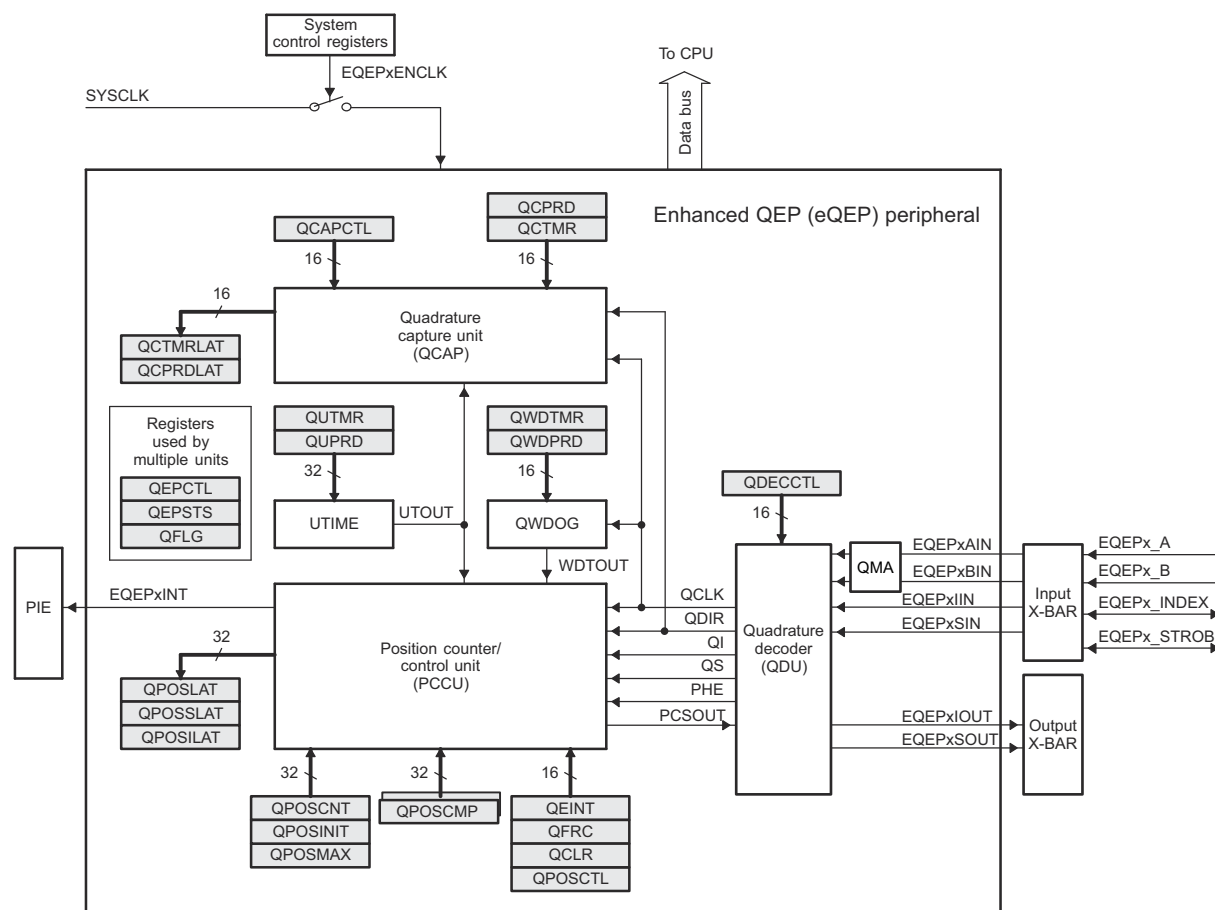
Figure 28-5. Functional Block Diagram of the eQEP Peripheral
