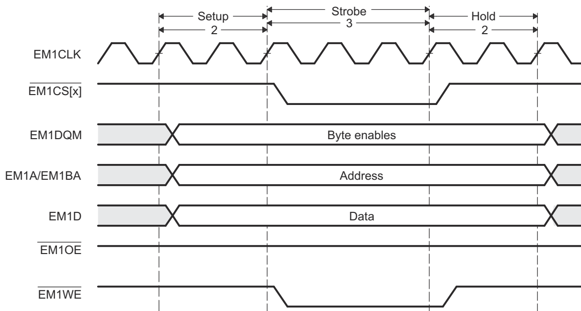
Figure 13-14. Timing Waveform of an Asynchronous Write Cycle in Select Strobe Mode
