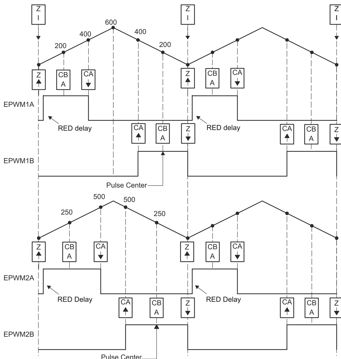
Figure 27-95. Half-H Bridge Waveforms for Control of Two Half-H Bridge Stages (Note: Here F_{PWM2} = F_{PWM1} )
