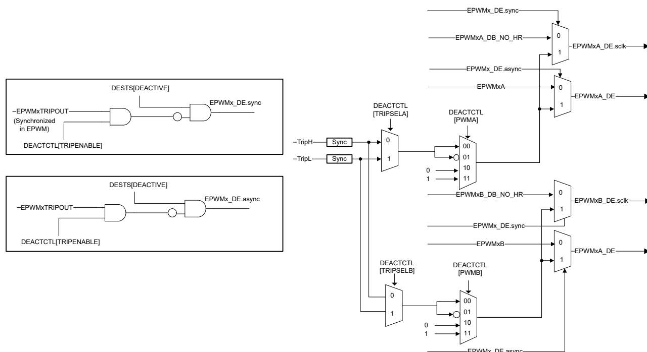
Figure 27-58. Diode Emulation Circuit
