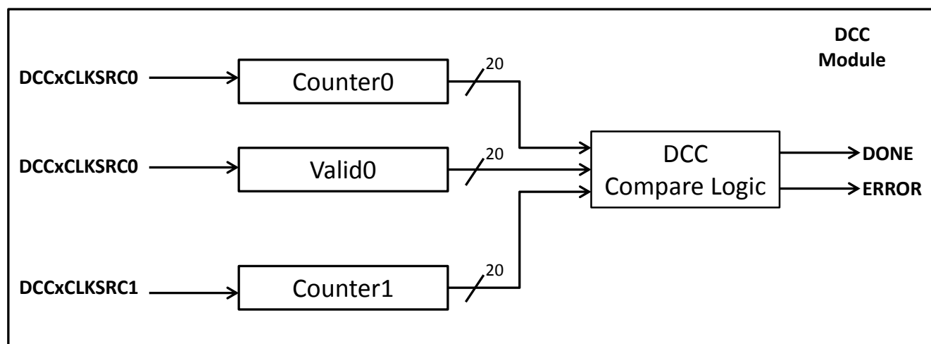
Figure 11-2. DCC Operation
