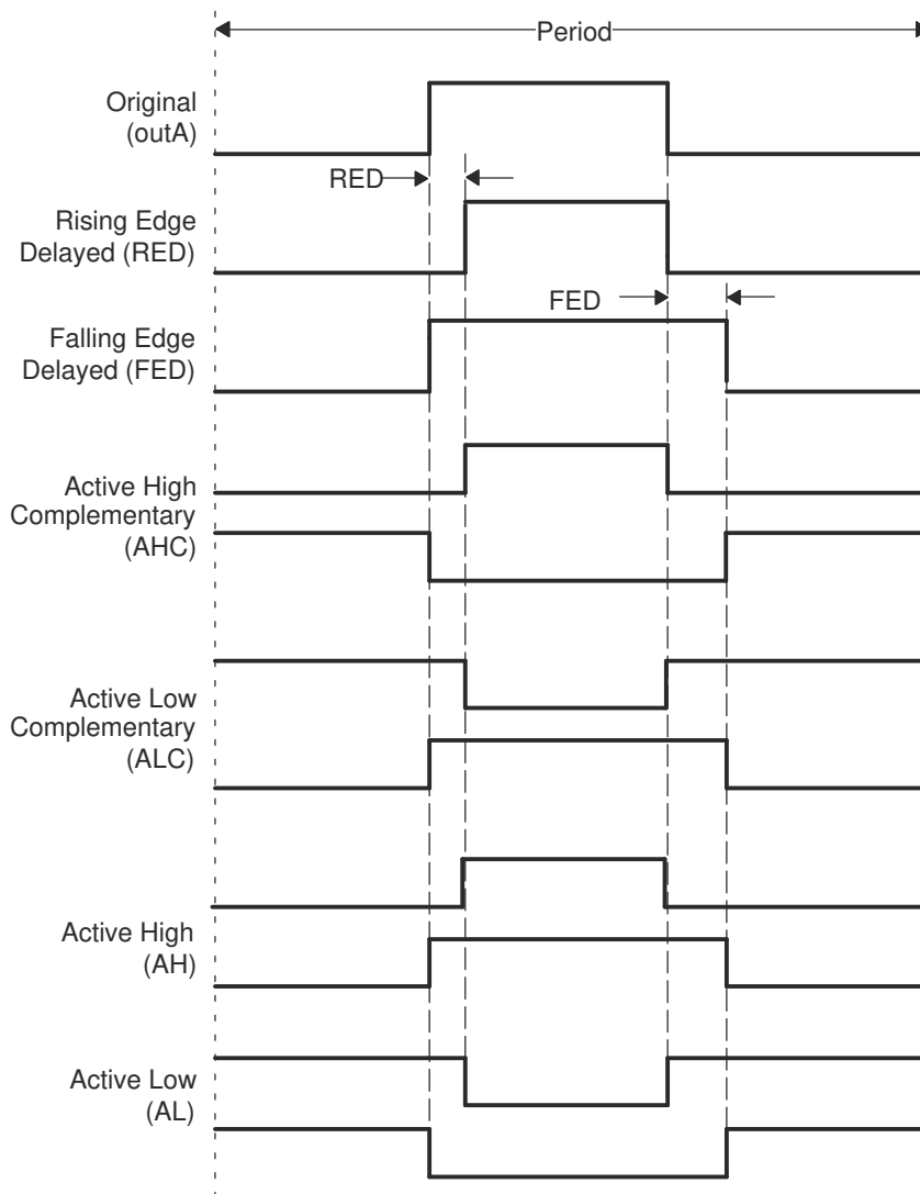
Figure 27-42. Dead-Band Waveforms for Typical Cases (0% < Duty < 100%)
