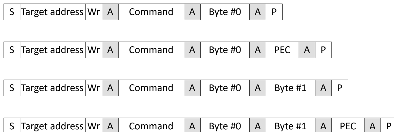
Figure 34-5. Write Byte and Write Word Messages With and Without PEC
