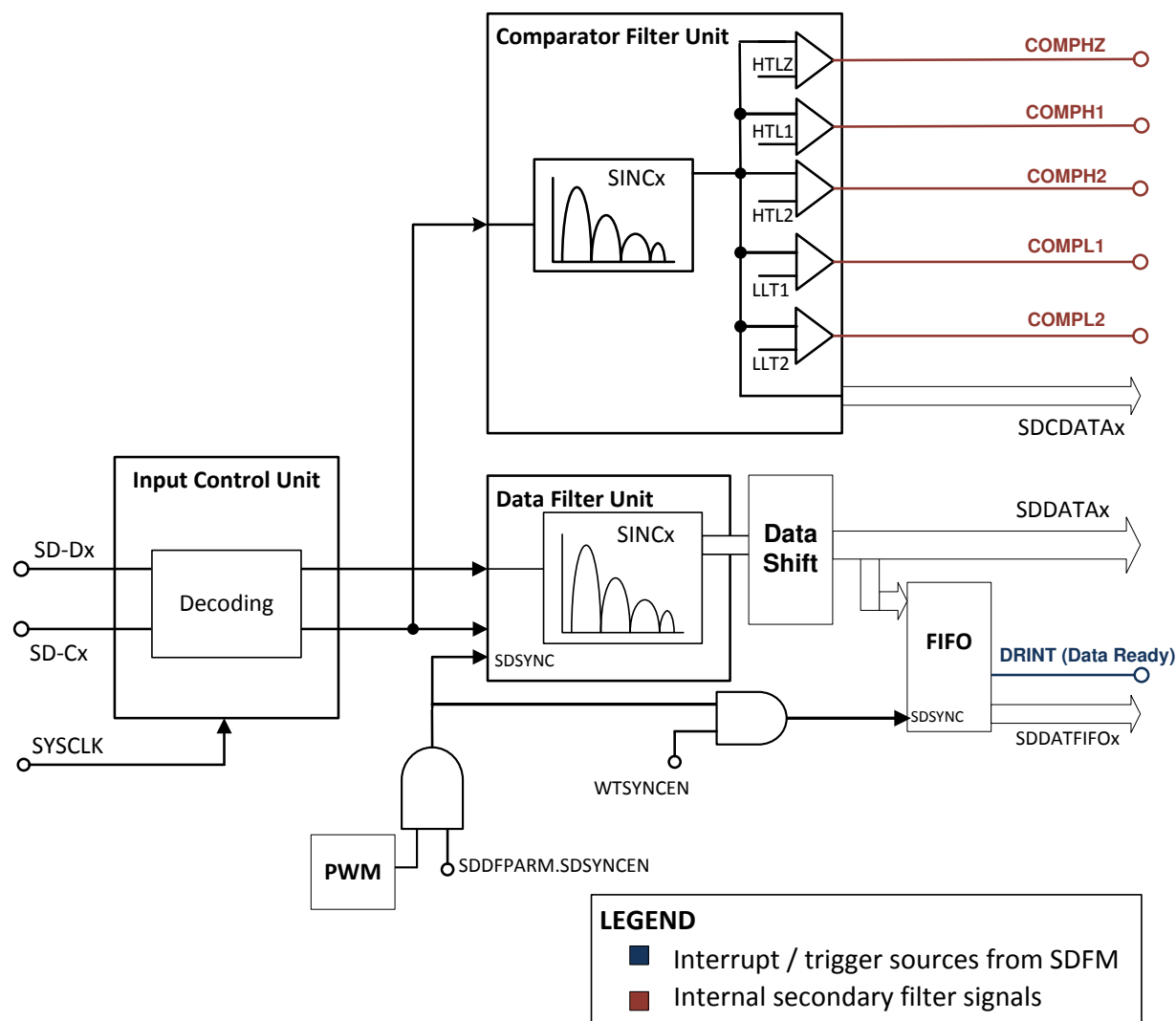
Figure 29-3. Block Diagram of One Filter Module
