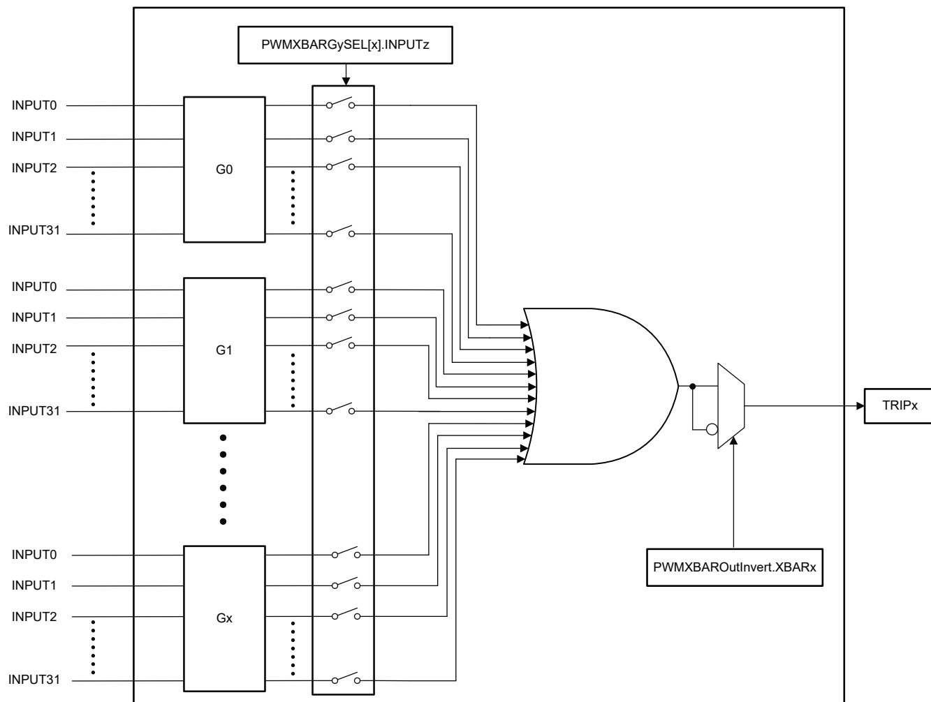
Figure 19-3. ePWM X-BAR Architecture - Single Output
