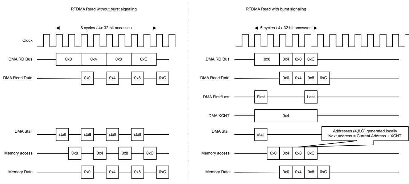
Figure 2-19. RTDMA Read
