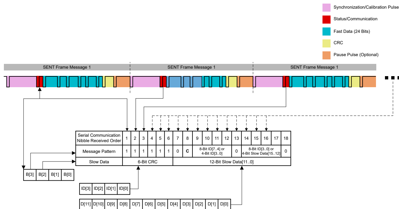
Figure 38-6. Enhanced Serial Message
