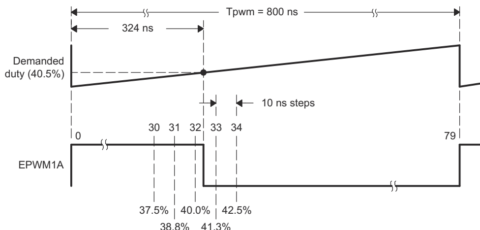
Figure 27-113. Required PWM Waveform for a Requested Duty = 40.5%
