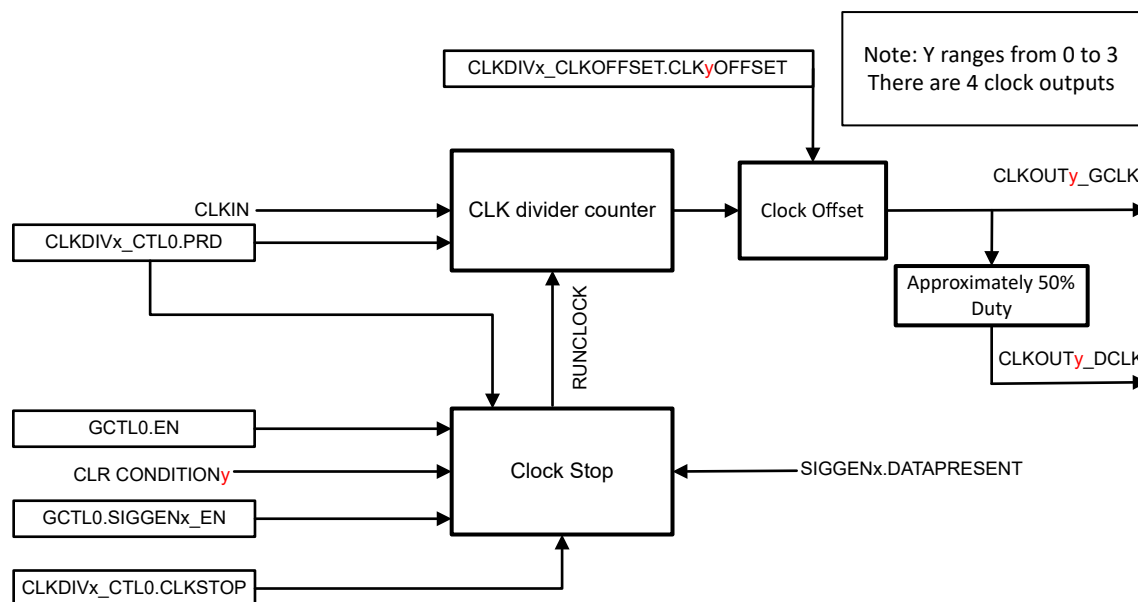
Figure 20-3. EPG Clock Generator
