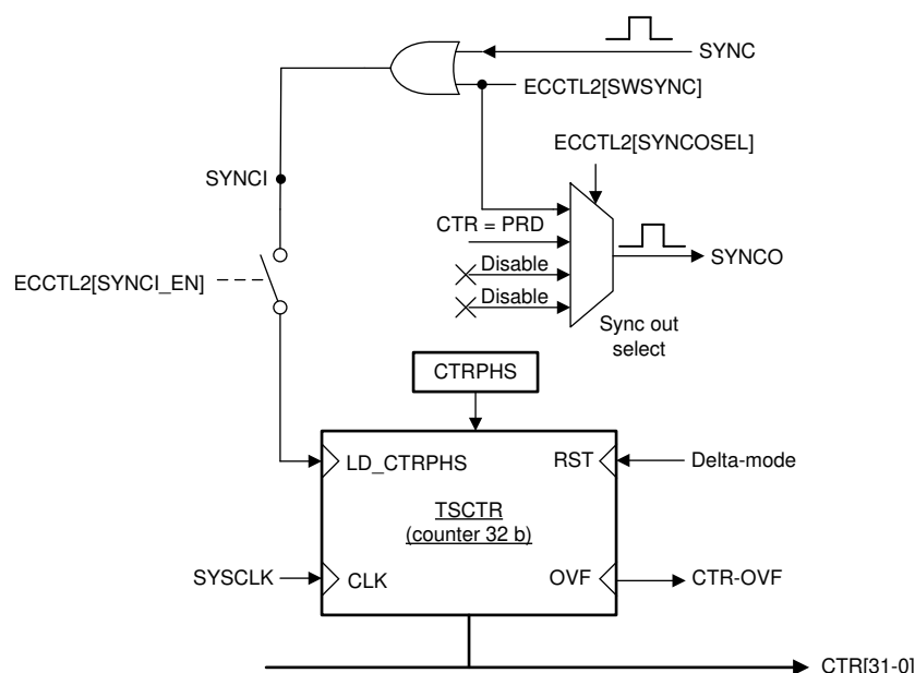
Figure 25-7. ECAP Counter and Synchronization Block
