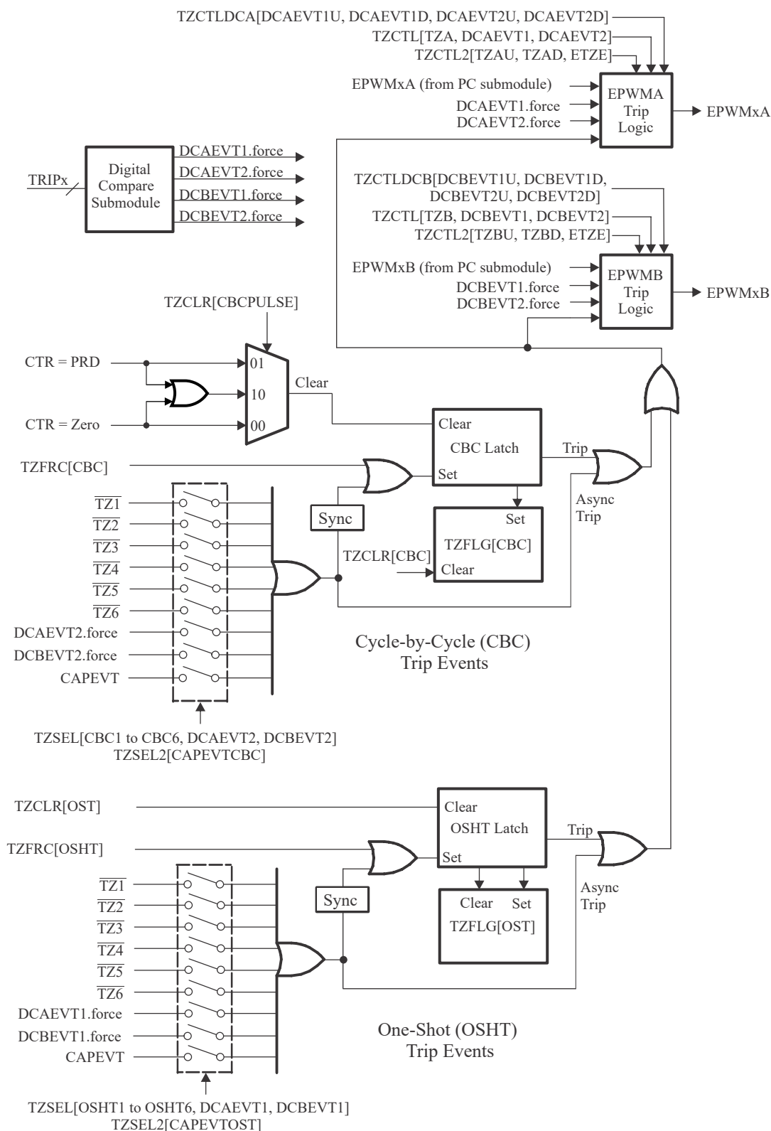
Figure 27-50. Trip-Zone Submodule Mode Control Logic
