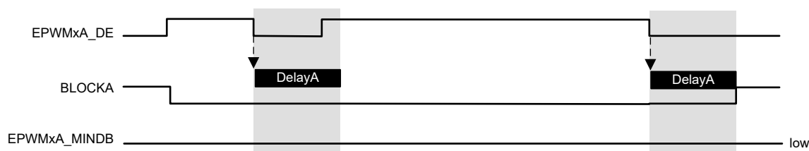
Figure 27-66. Rising Edge During Delay
