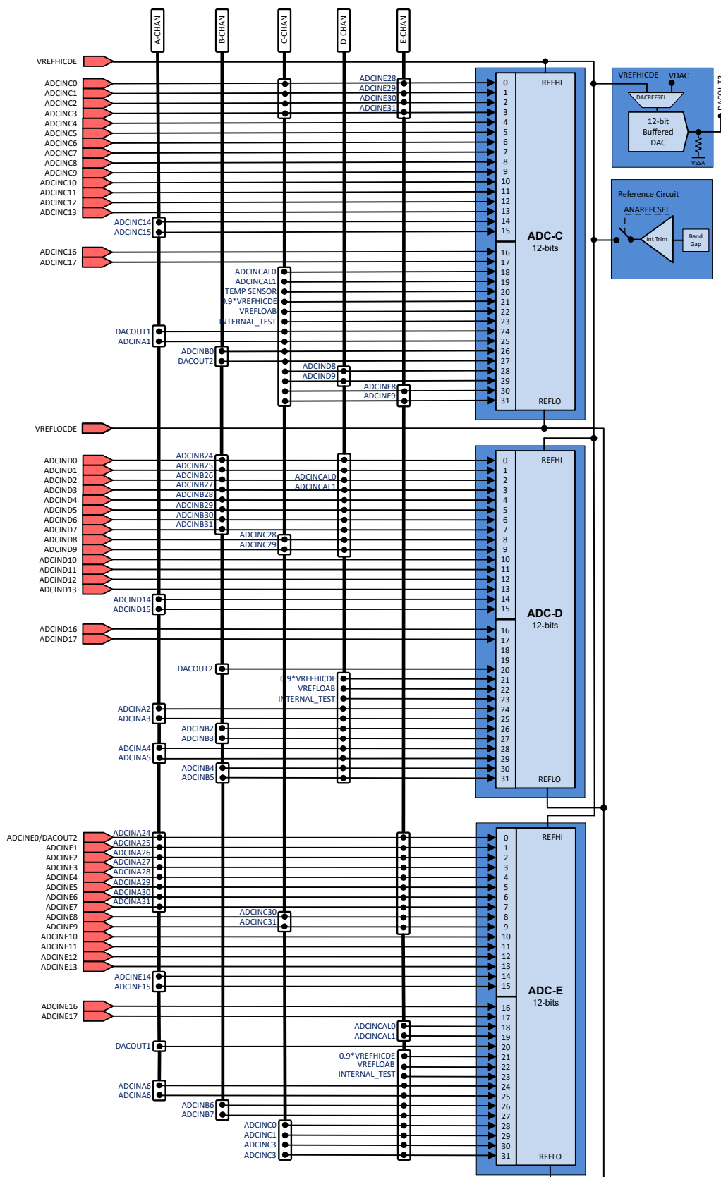
Figure 21-2. Analog Subsystem Block Diagram (ADC C, ADC D, and ADC E)
