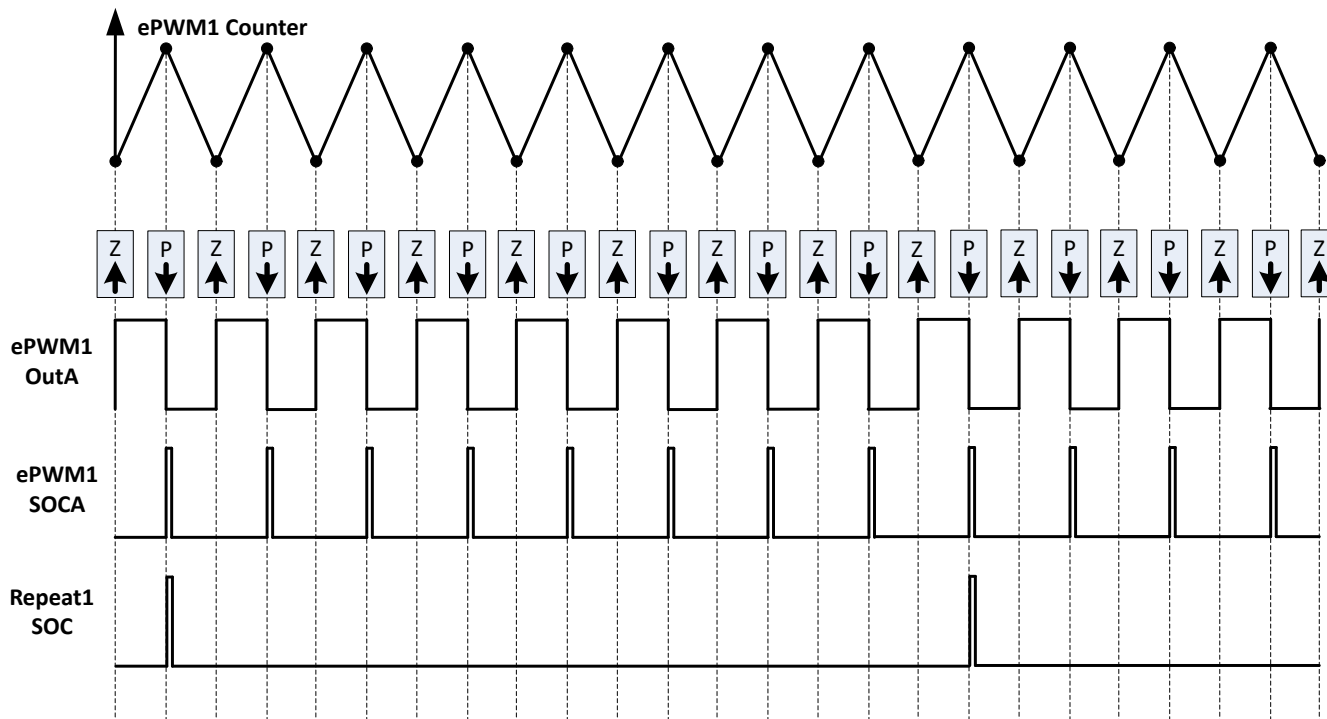
Figure 22-5. Undersampled ADC Trigger Example
