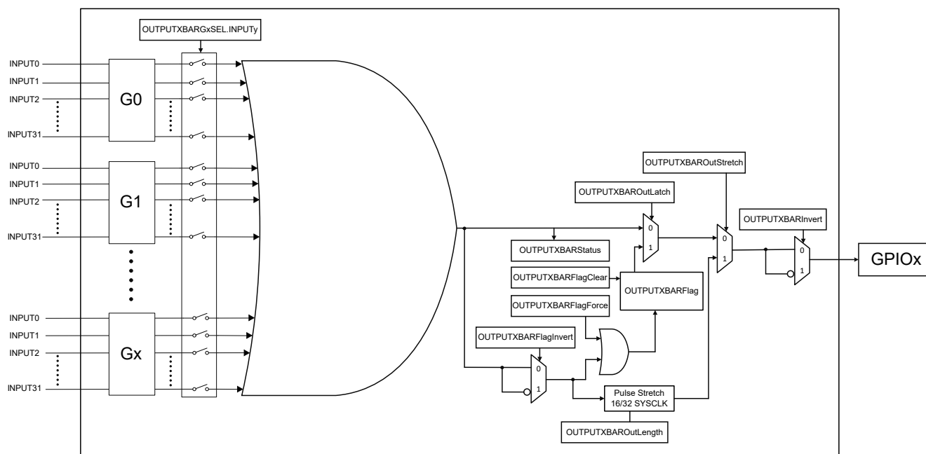
Figure 19-6. GPIO Output X-BAR Architecture
