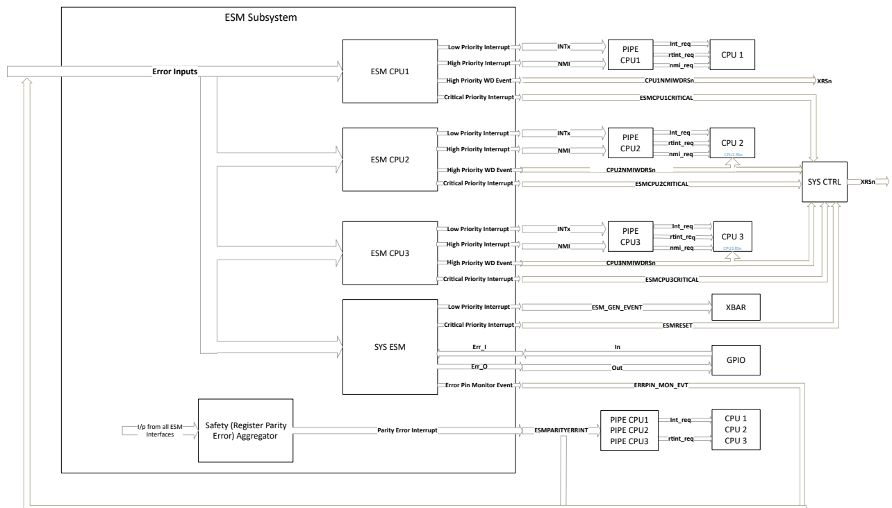
Figure 7-4. ESM Subsystem Integration View
