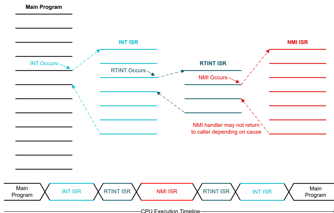
Figure 5-4. Interrupt Nesting Example Diagram
