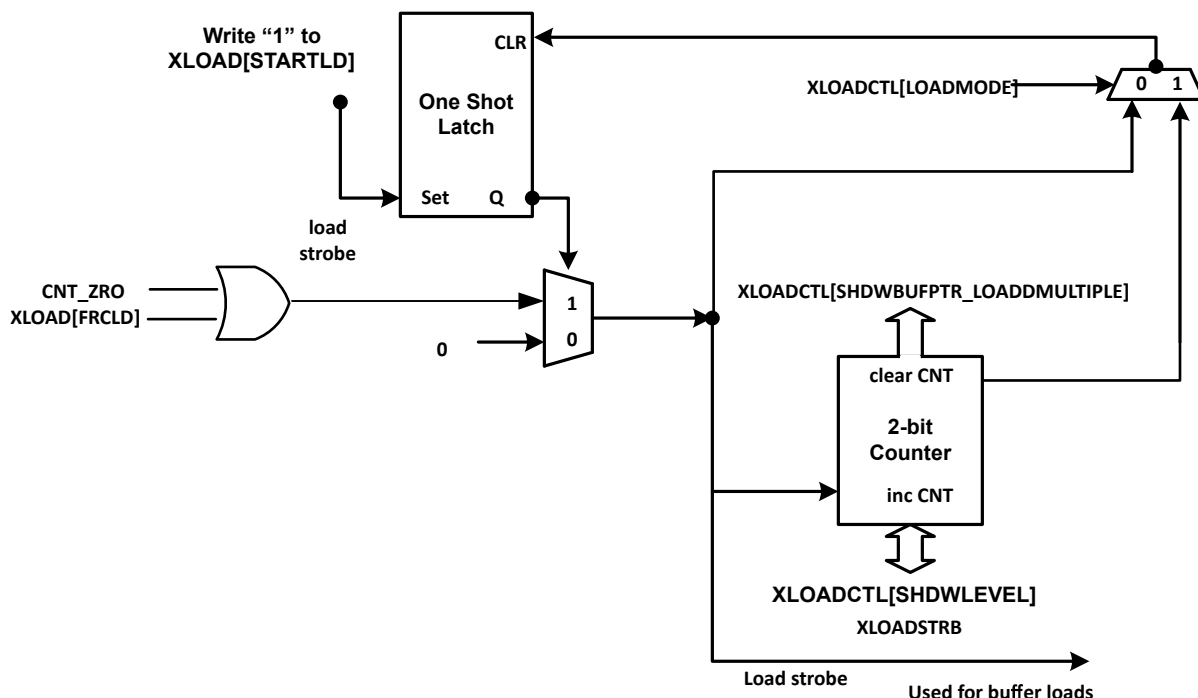
Figure 27-38. Global Load: Signals and Registers
