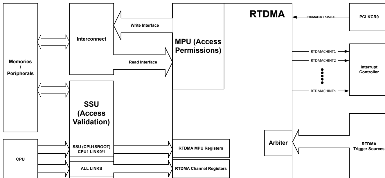
Figure 12-1. RTDMA Block Diagram
