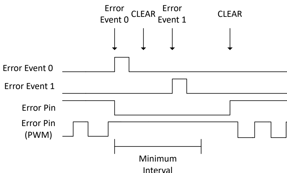
Figure 7-14. Error Pin Asserting with New Error During Minimum Time Interval
