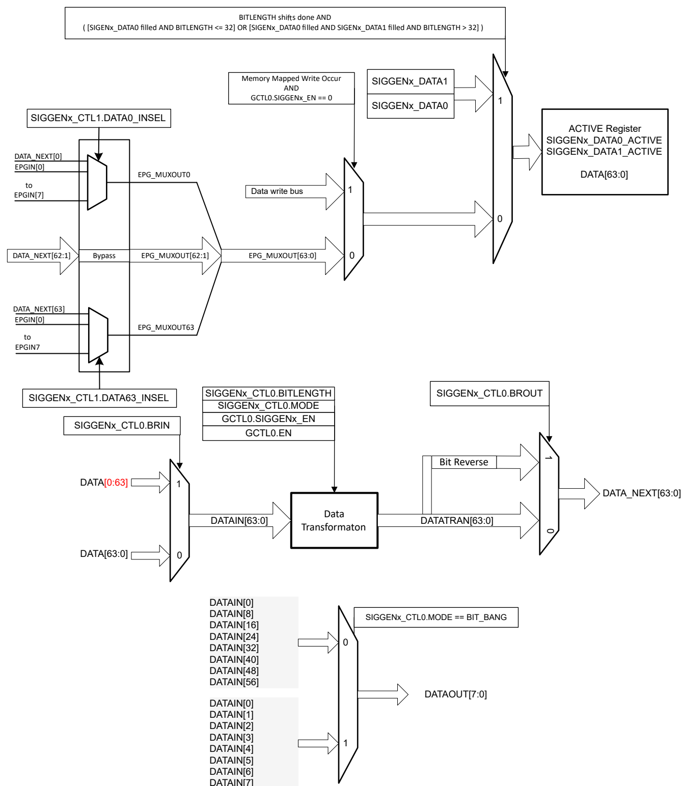
Figure 20-5. EPG Signal Generator Detailed Overview
