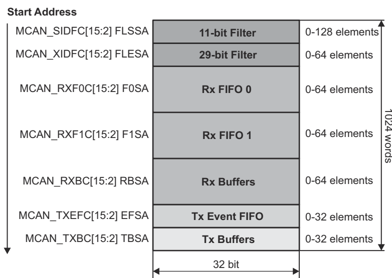
Figure 30-19. Message RAM Configuration
