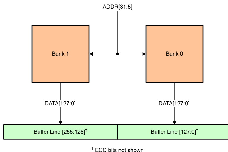
Figure 8-5. Interleaved Bank to Buffer Mapping
