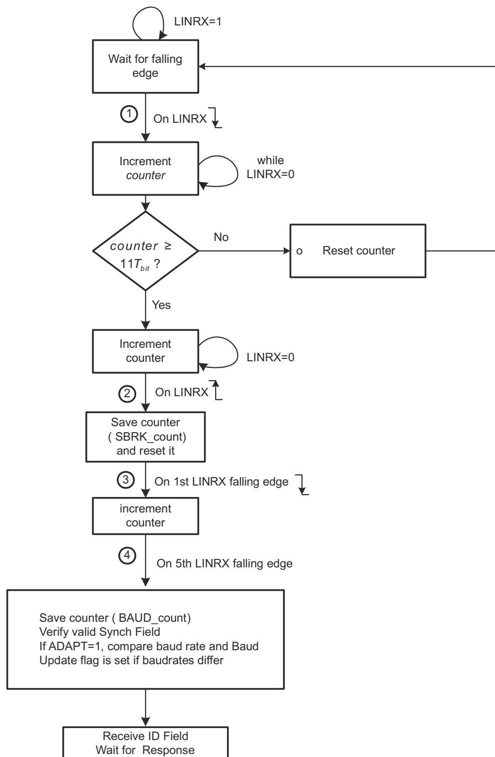
Figure 36-18. Synchronization Validation Process and Baud Rate Adjustment
