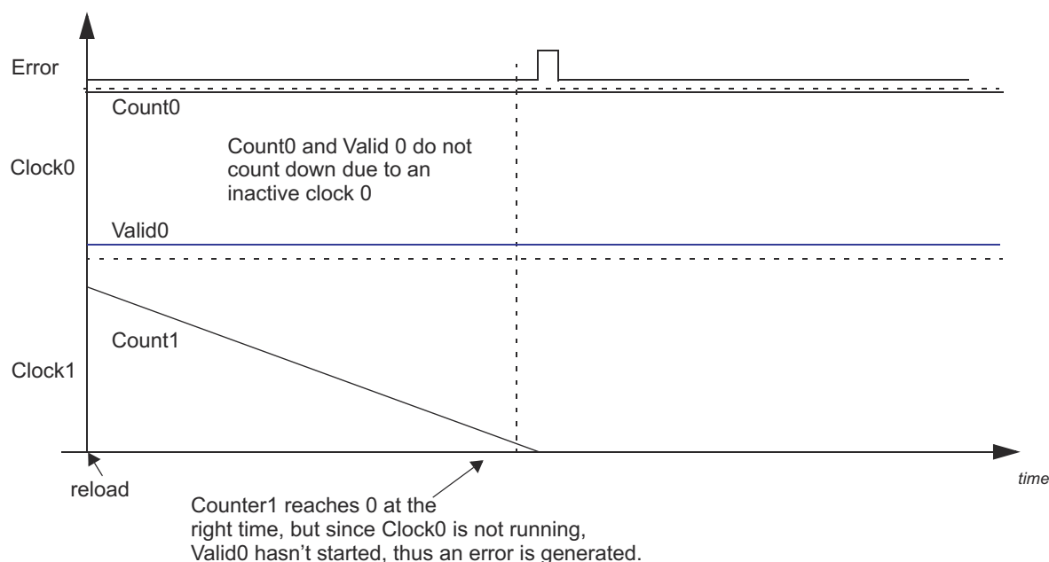
Figure 11-7. Clock0 Not Present - Results in an Error and Stops Counting
