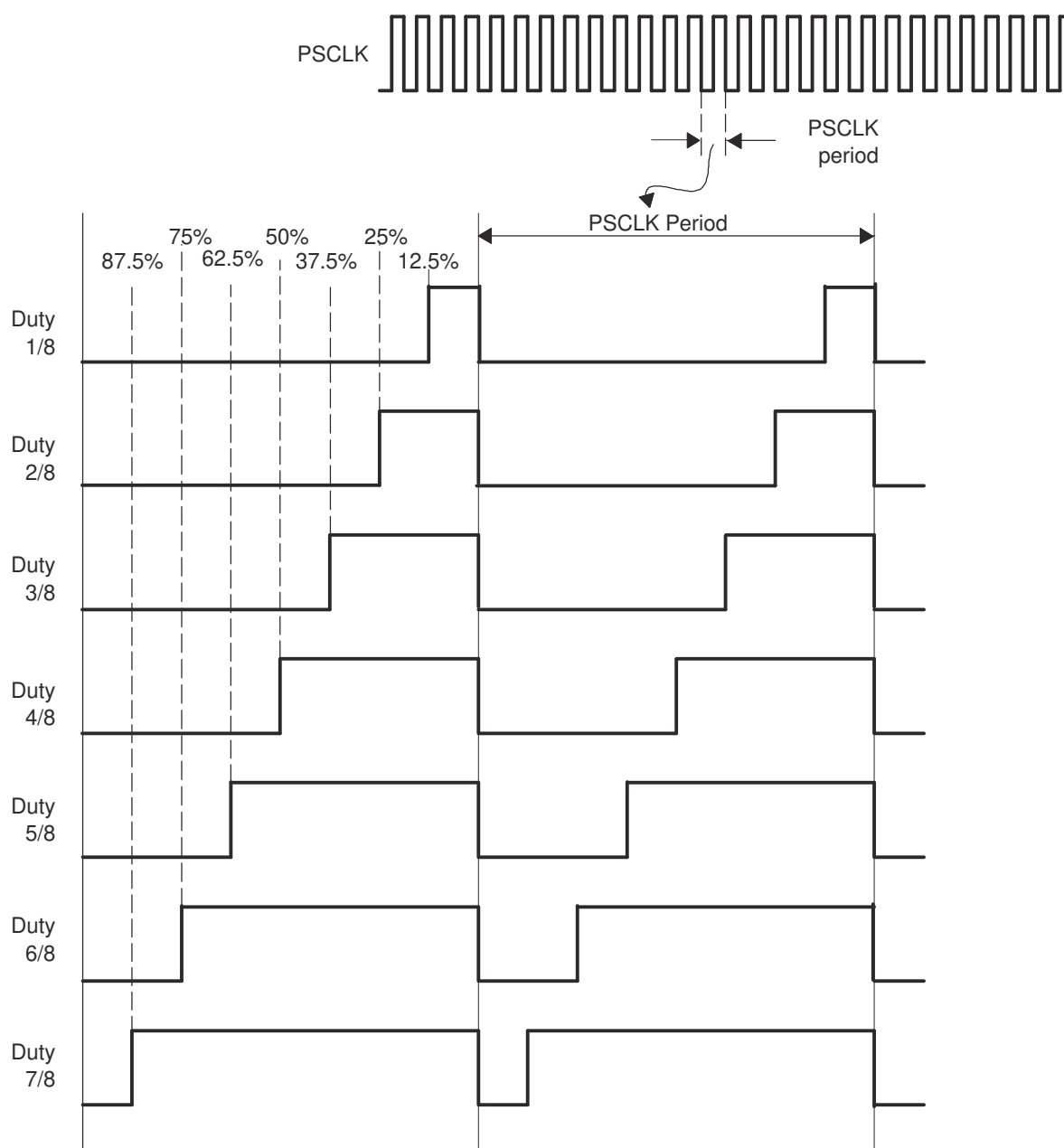
Figure 27-47. PWM Chopper Submodule Waveforms Showing the Pulse Width (Duty Cycle) Control of Sustaining Pulses
