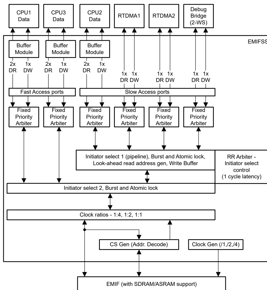
Figure 13-15. EMIFSS Block Diagram
