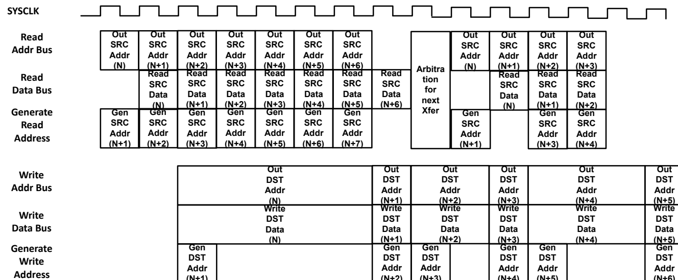
Figure 12-6. 3-stage Pipeline: With Multicycle Write Stall
