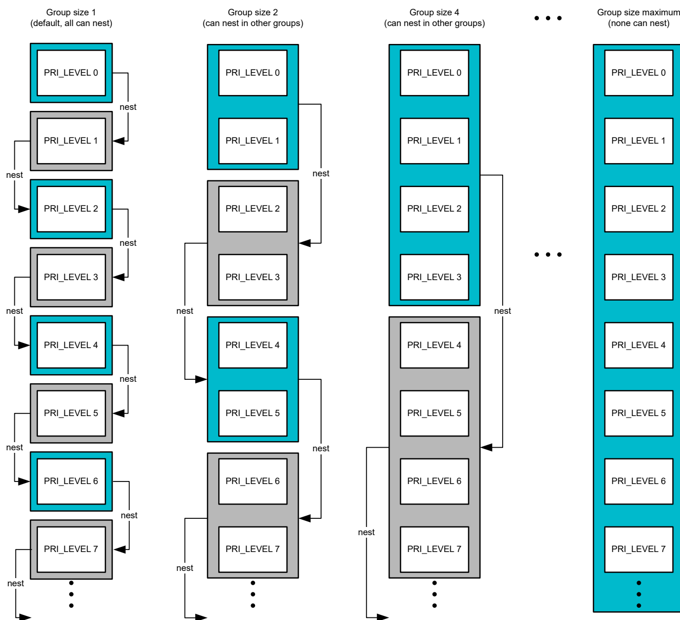
Figure 5-5. Interrupt Grouping
