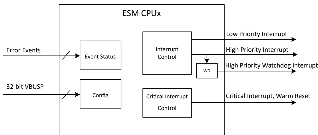
Figure 7-5. ESM CPU Block Diagram
