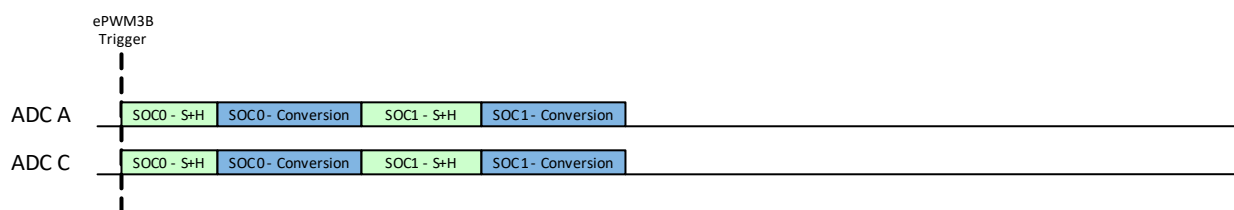
Figure 22-36. Example: Basic Synchronous Operation
