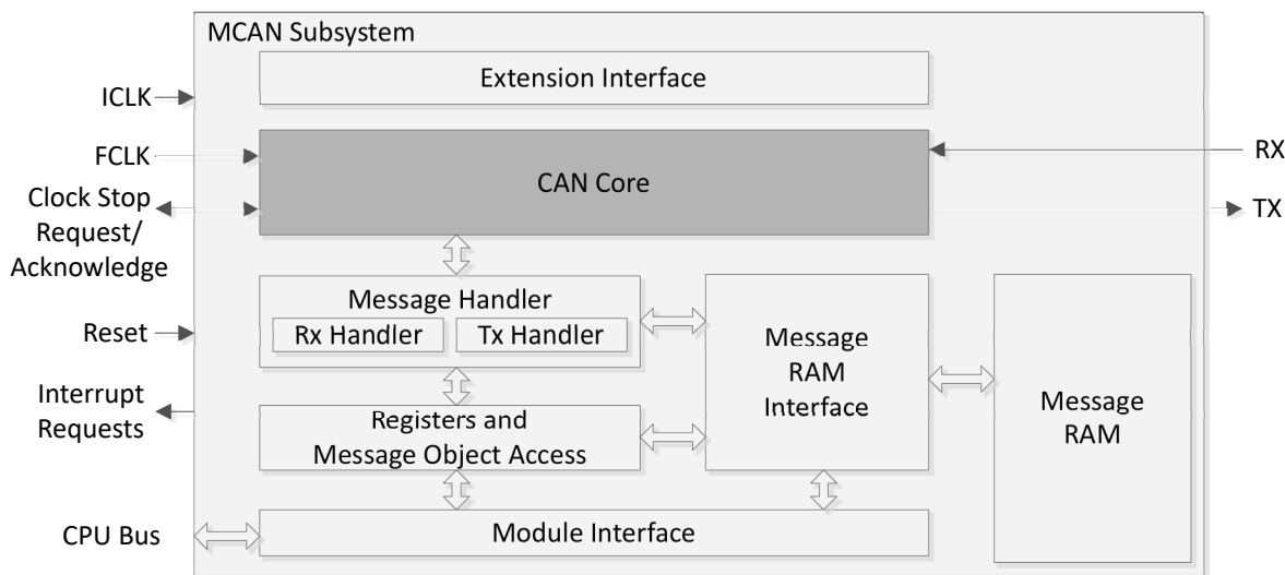
Figure 30-4. MCAN Block Diagram
