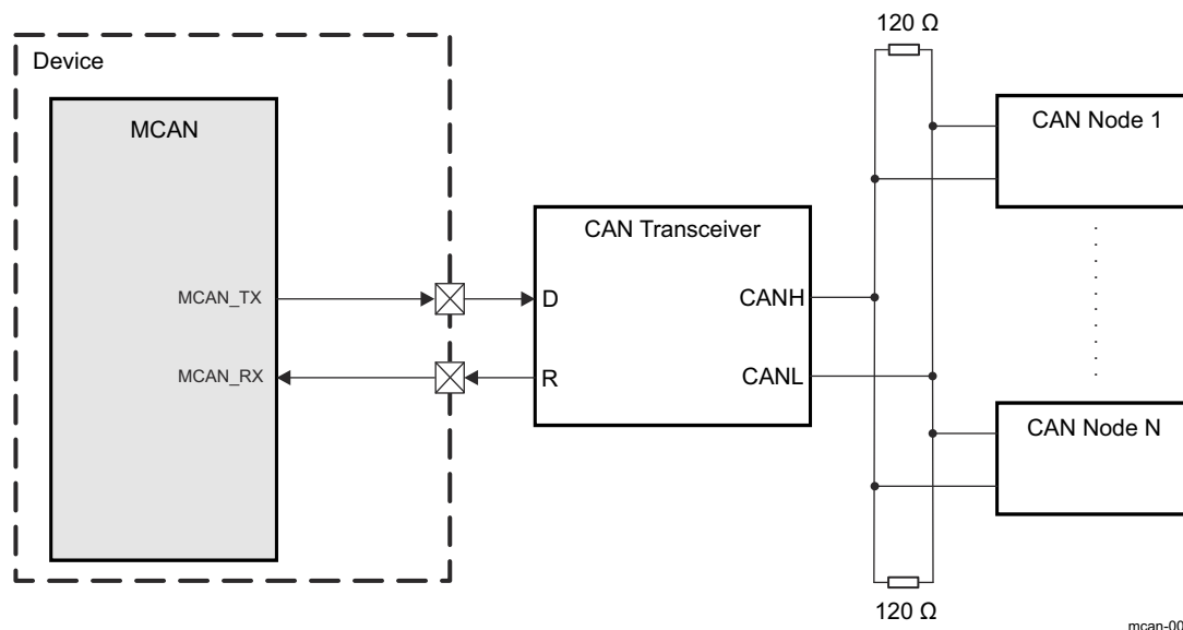
Figure 30-2. MCAN Typical Bus Wiring
