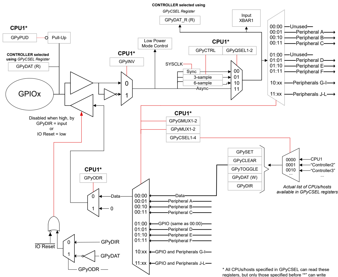
Figure 14-1. GPIO Logic for a Single Pin
