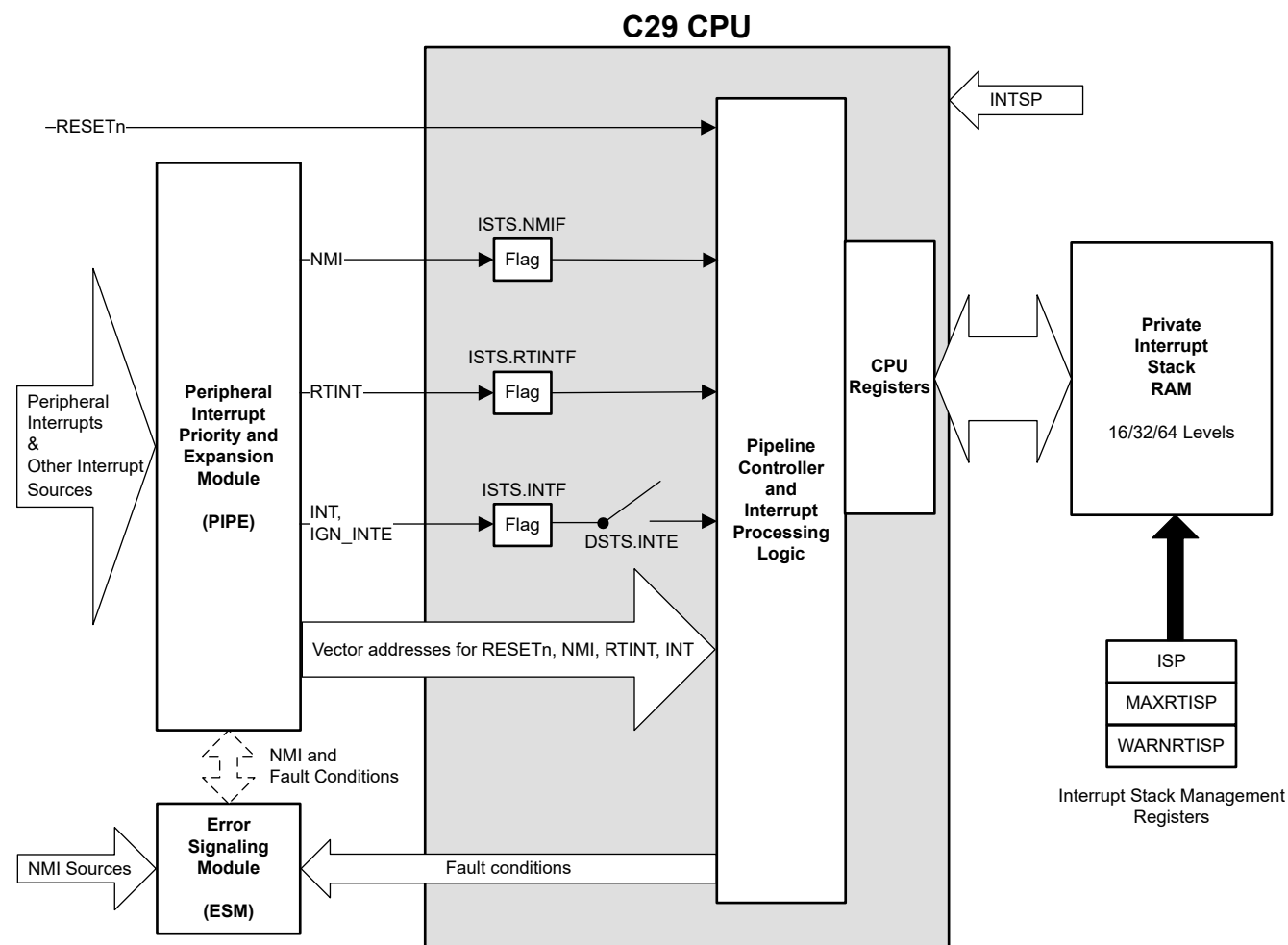
Figure 5-1. C29x CPU Interrupts Architecture Block Diagram
