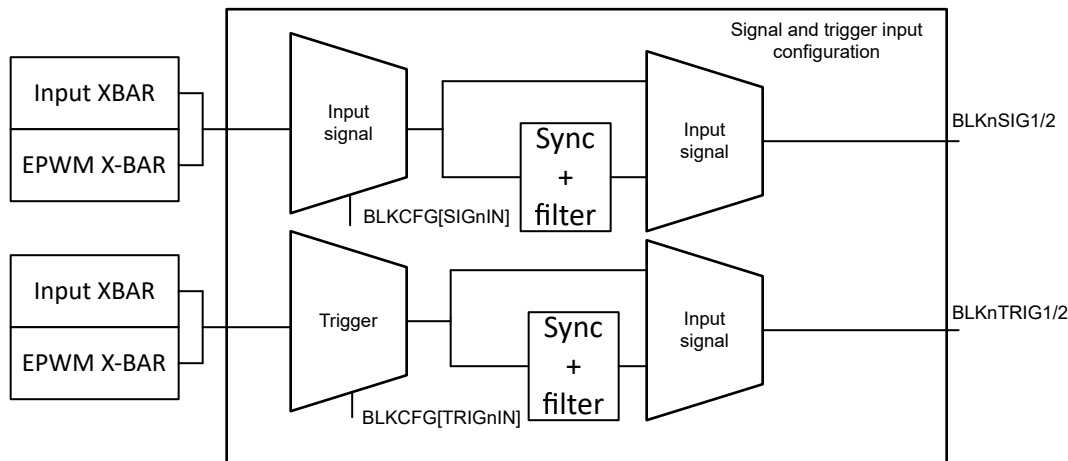
Figure 18-2. WADI Signal Input and Trigger Configuration
