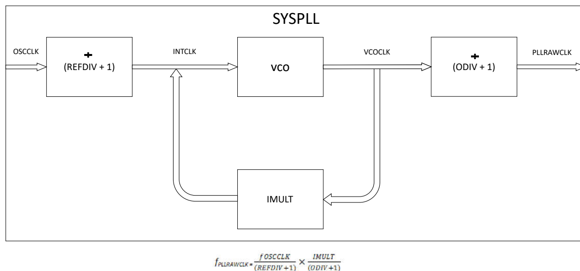
Figure 2-9. PLL
