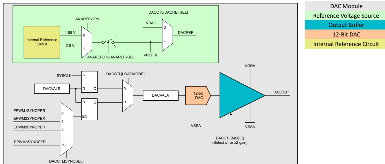
Figure 23-1. DAC Module Block Diagram
