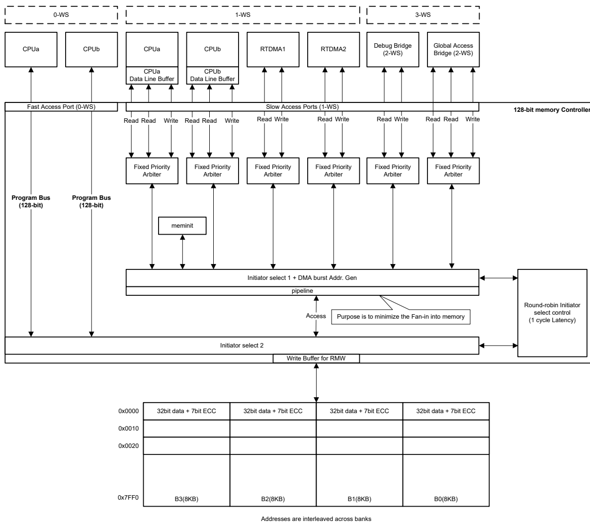
Figure 2-16. 128-Bit Memory Controller
