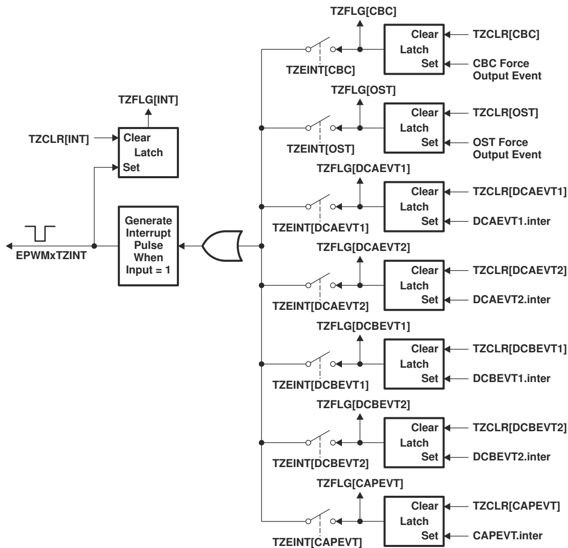
Figure 27-51. Trip-Zone Submodule Interrupt Logic
