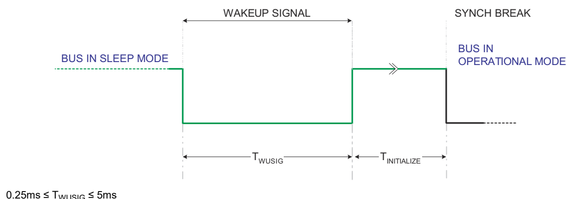
Figure 36-26. Wakeup Signal Generation
