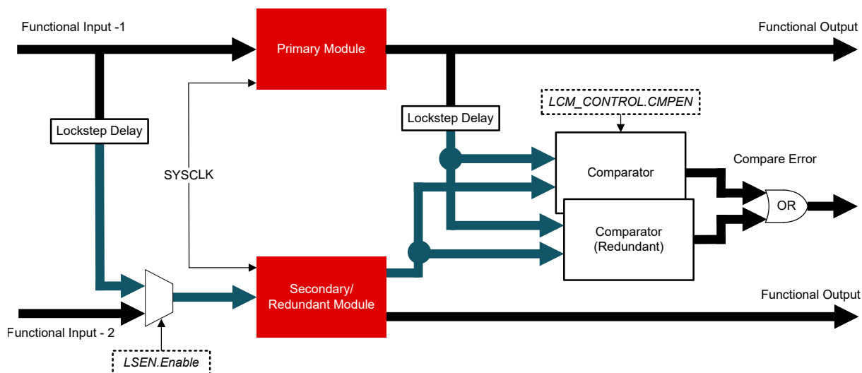
Figure 4-1. LCM Block Diagram
