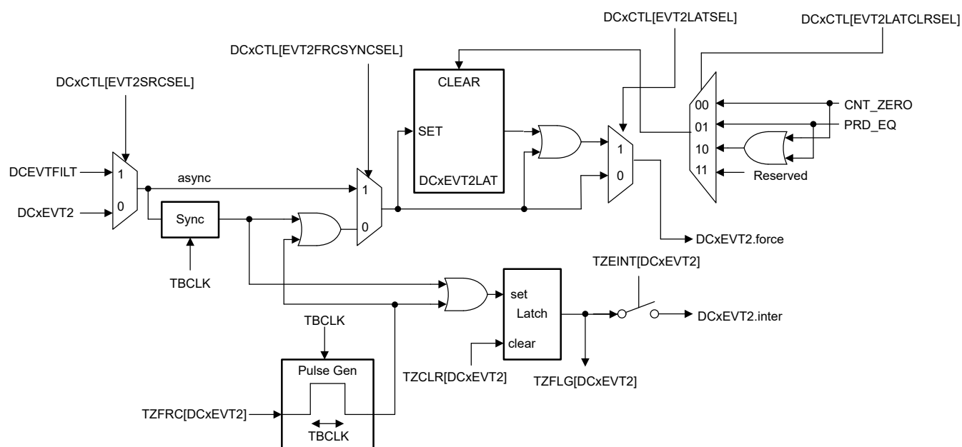
Figure 27-77. DCxEVT2 Event Triggering
