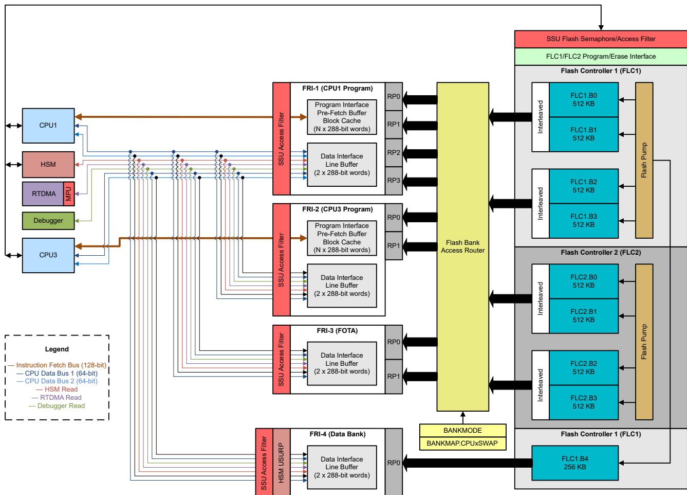
Figure 8-1. Flash Subsystem Block Diagram
