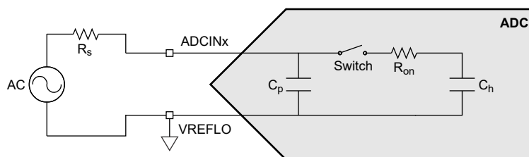
Figure 22-11. Single-Ended Input Model
