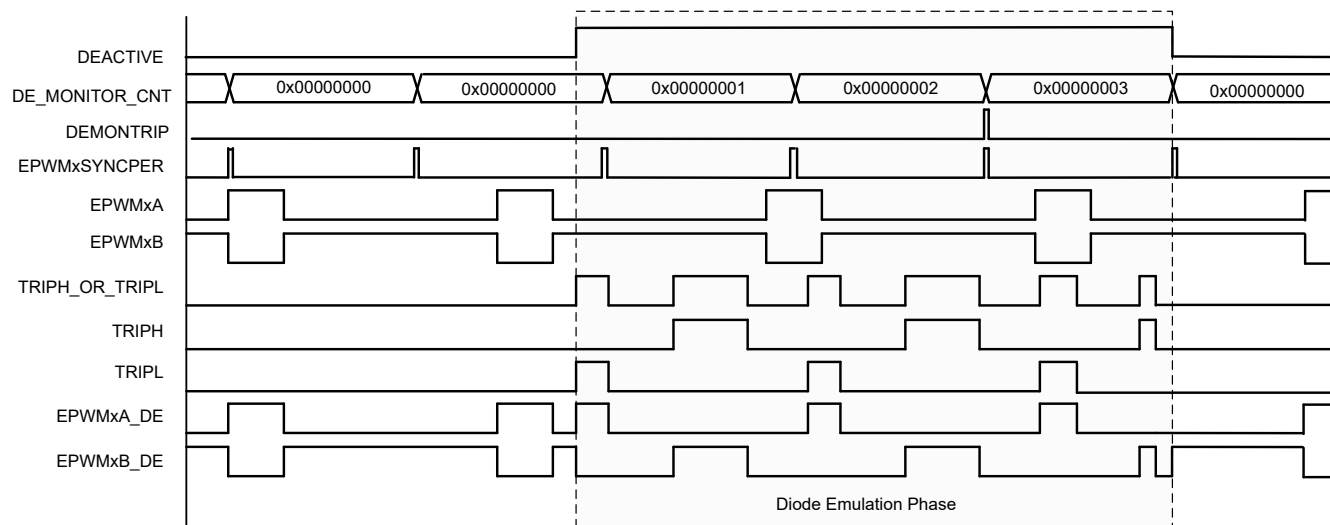
Figure 27-60. DE Mode Monitor Sequence
