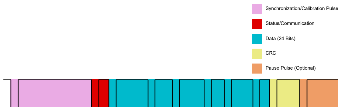
Figure 38-4. Fast Message
