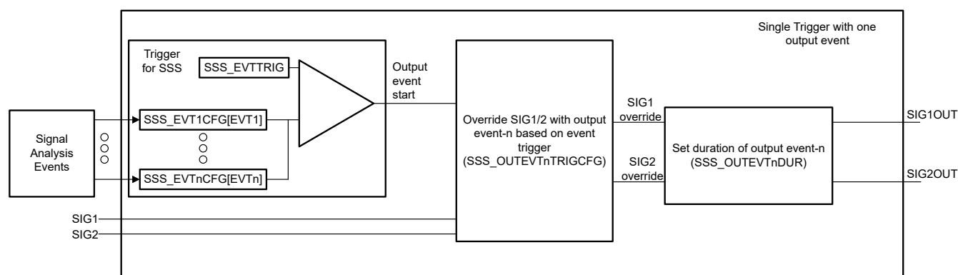
Figure 18-9. Single Trigger with Single Pattern Output Event
