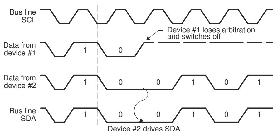
Figure 33-17. Arbitration Procedure Between Two Controller-Transmitters
