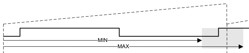
Figure 27-86. Capture Logic Boundary Condition
