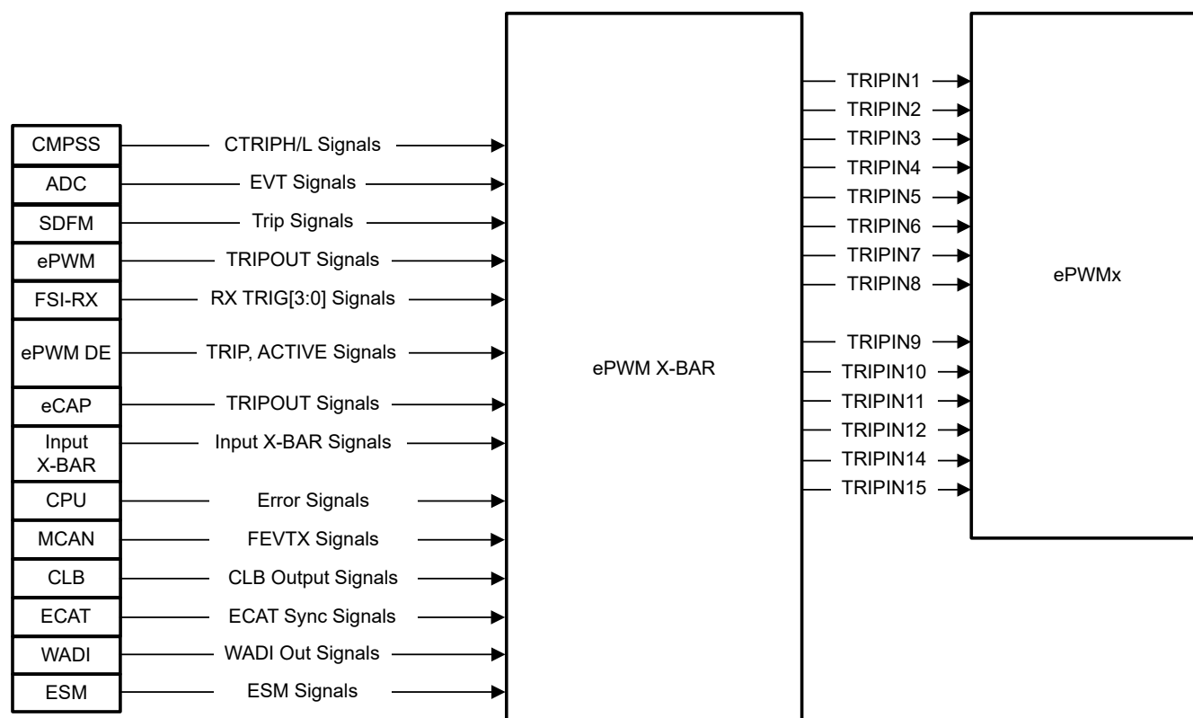
Figure 27-87. ePWM X-BAR
