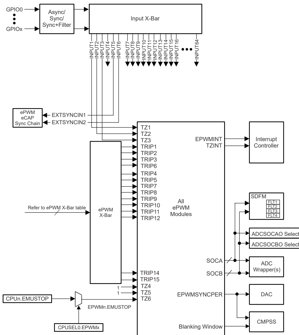
Figure 27-75. GPIO MUX-to-Trip Input Connectivity
