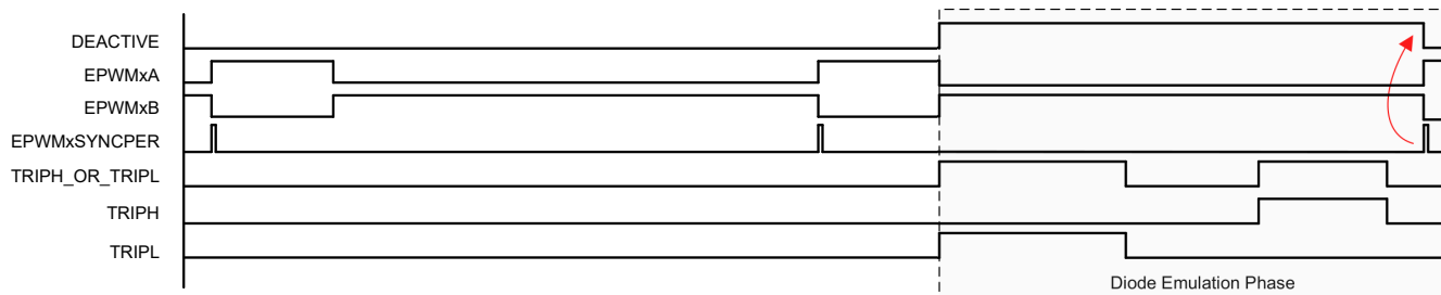
Figure 27-56. Cycle-by-Cycle Mode
