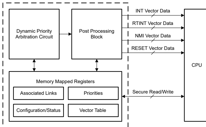
Figure 5-2. PIPE Architecture
