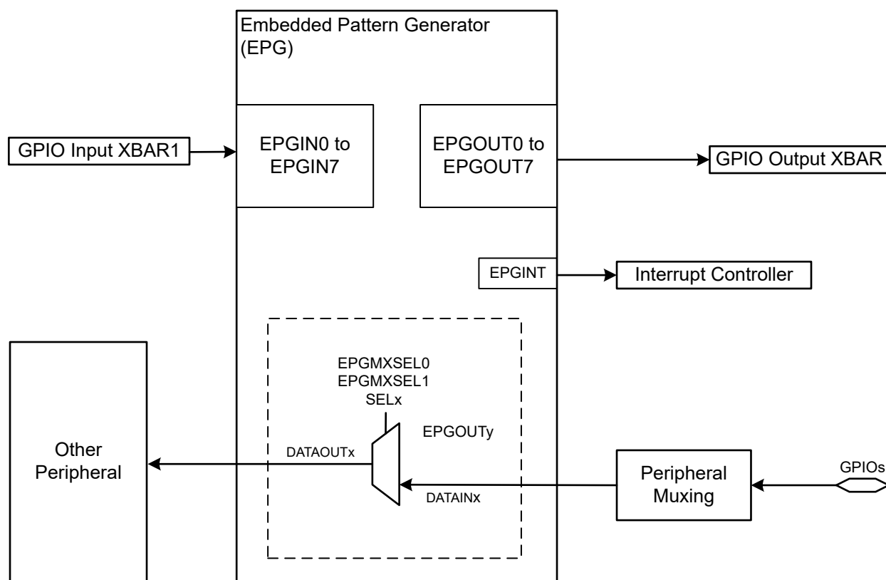
Figure 20-6. EPG Peripheral Signal Muxing
