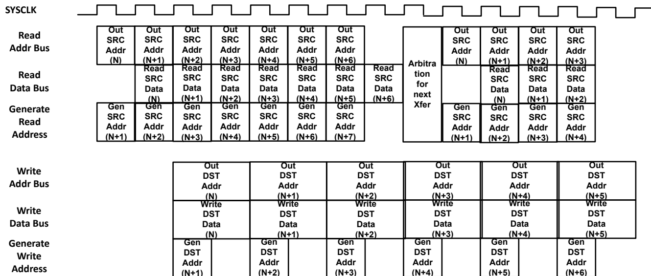
Figure 12-5. 3-stage Pipeline: With One Write Stall
