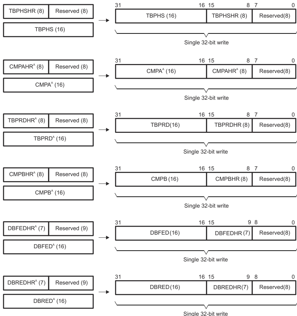
Figure 27-111. HRPWM Extension Registers and Memory Configuration
