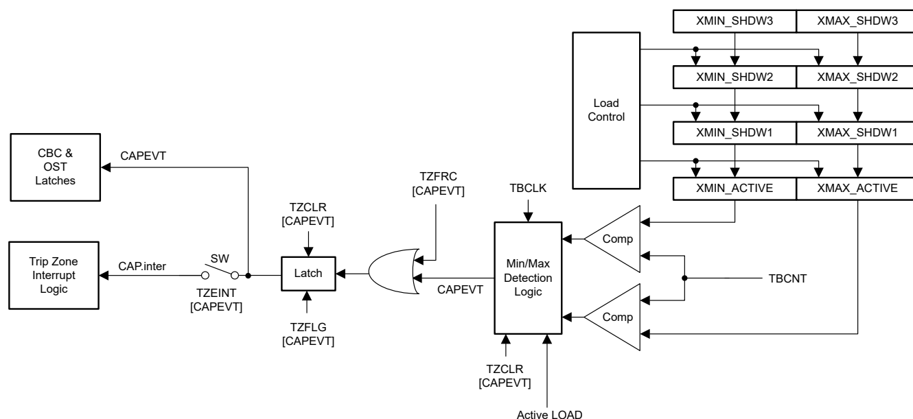
Figure 27-85. MIN and MAX Threshold Detection Logic
