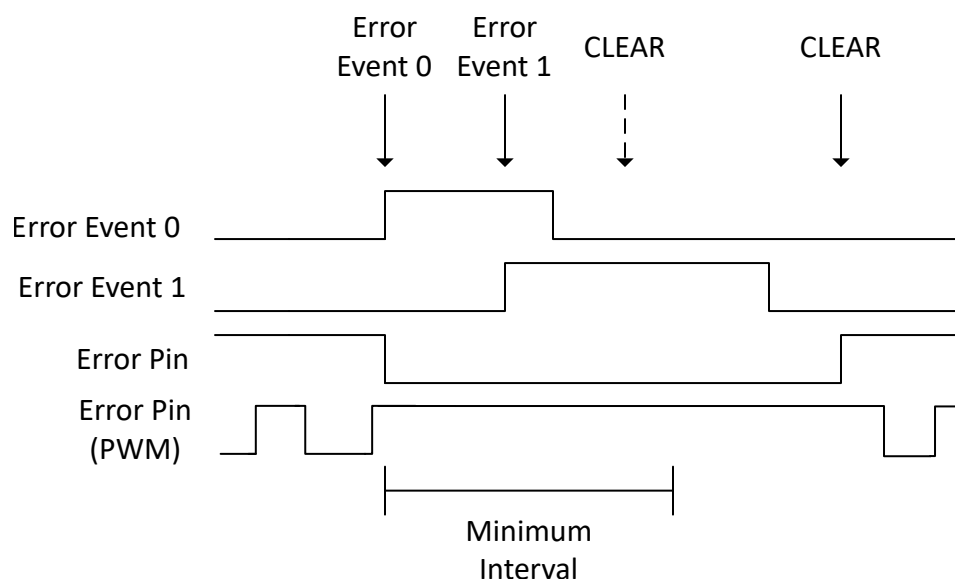
Figure 7-13. Error Pin Asserting with Single CLEAR for Multiple Events
