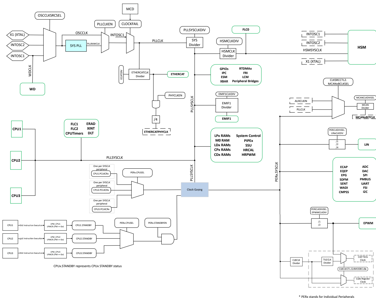
Figure 2-4. Clocking System
