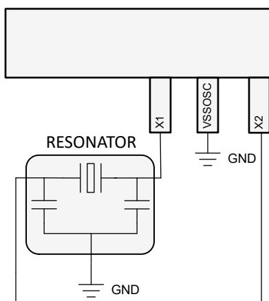
Figure 2-7. External Resonator
