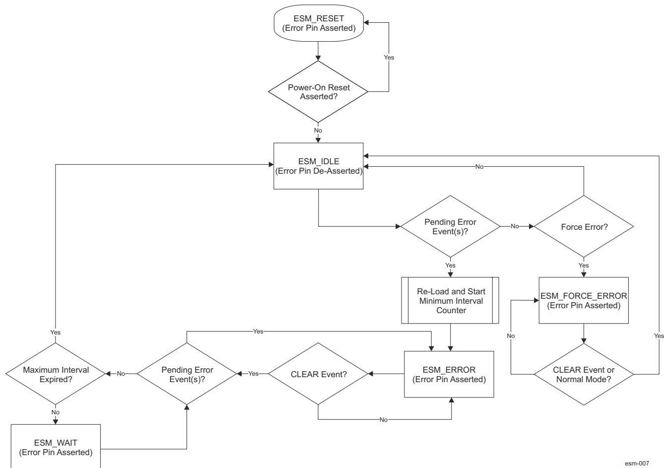
Figure 7-8. Error Pin State Flowchart
