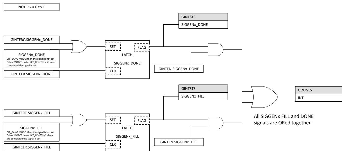
Figure 20-7. EPG Interrupt
