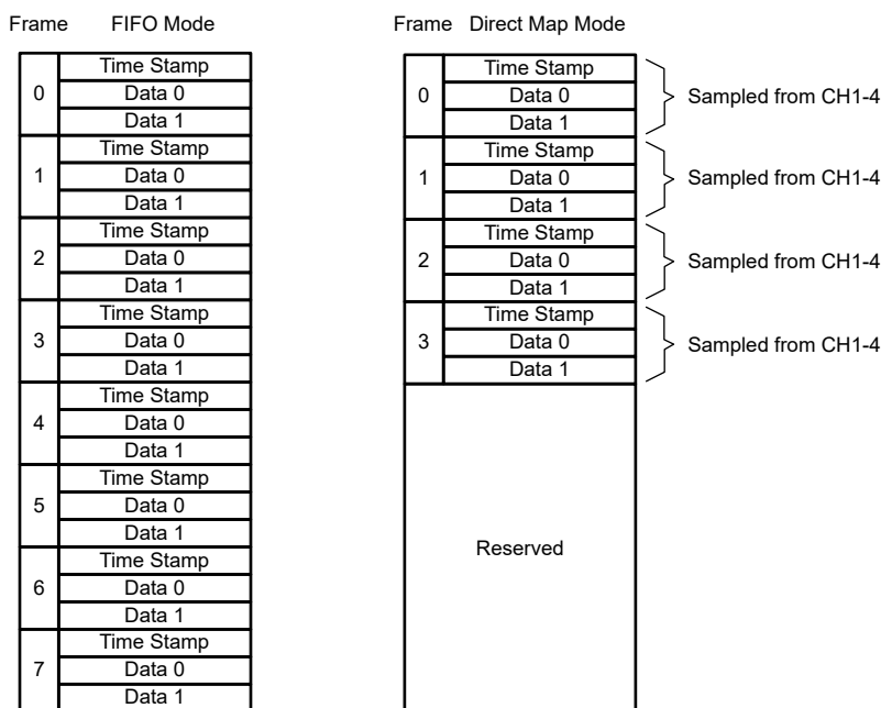
Figure 38-8. FIFO versus Direct Map Receive Modes
