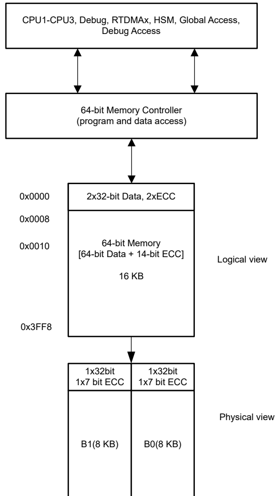
Figure 2-17. Generic view of 64-Bit Memory
