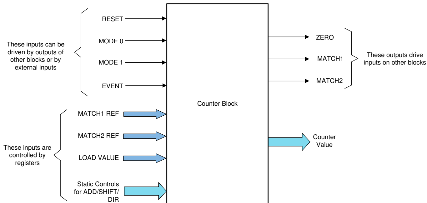
Figure 10-12. Counter Block
