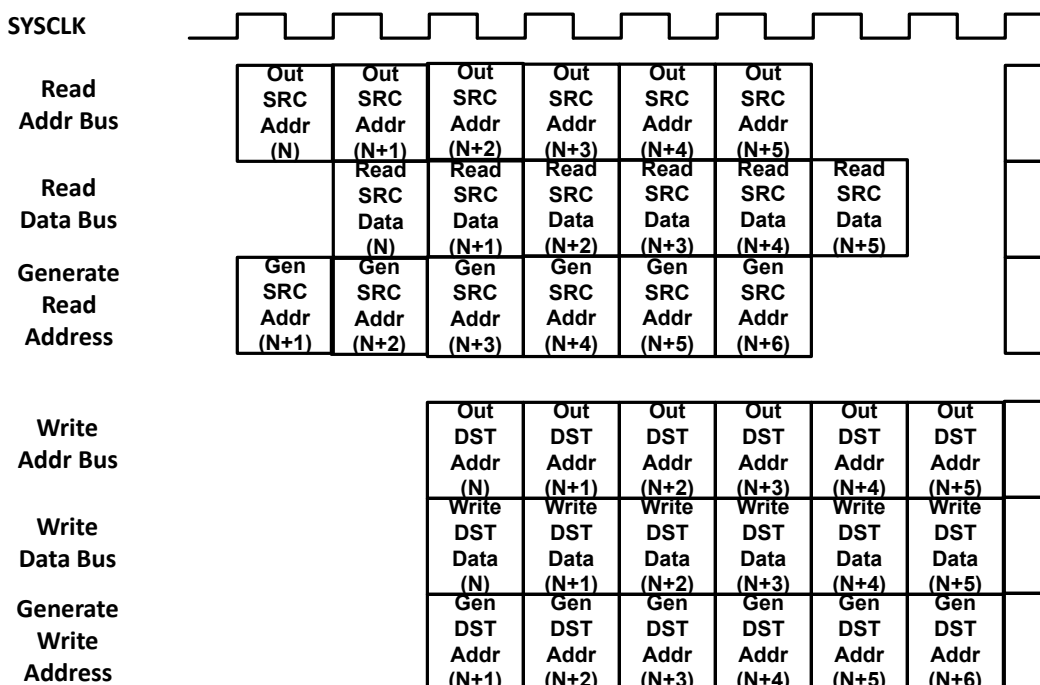
Figure 12-3. 3-stage Pipeline: With 0 Cycle Read Stall and 0 Cycle Write Stall
