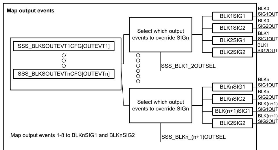
Figure 18-8. Map Output Events to BLK1SIGn
