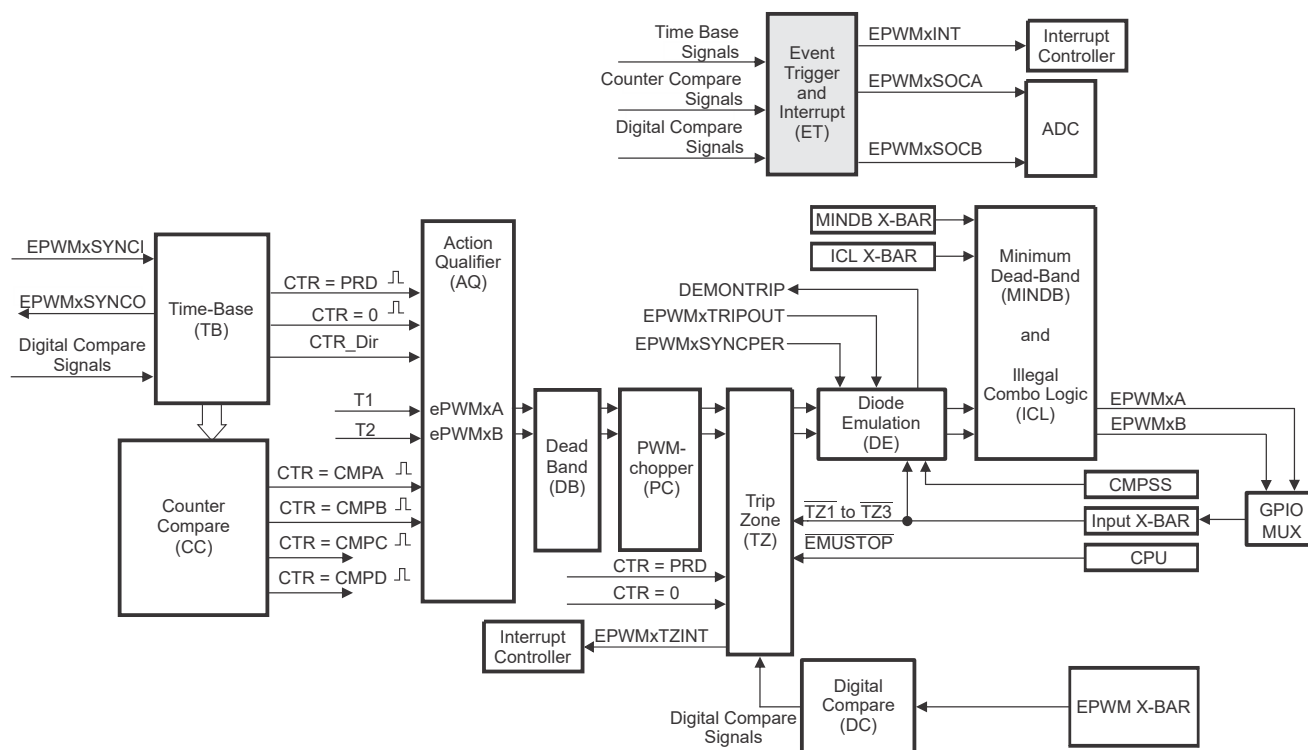
Figure 27-69. Event-Trigger Submodule
