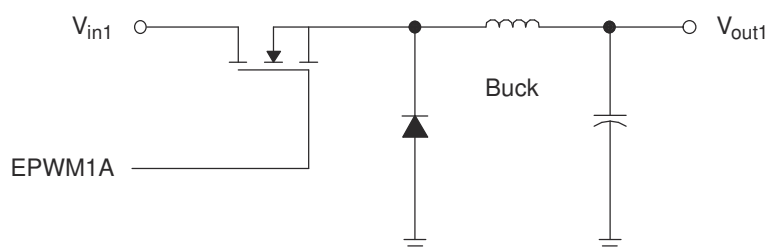
Figure 27-118. Simple Buck Controlled Converter Using a Single PWM
