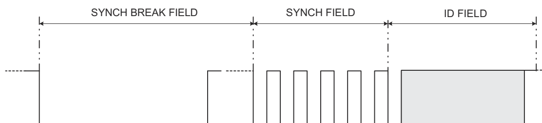
Figure 36-13. Header 3 Fields: Synch Break, Synch, and ID
