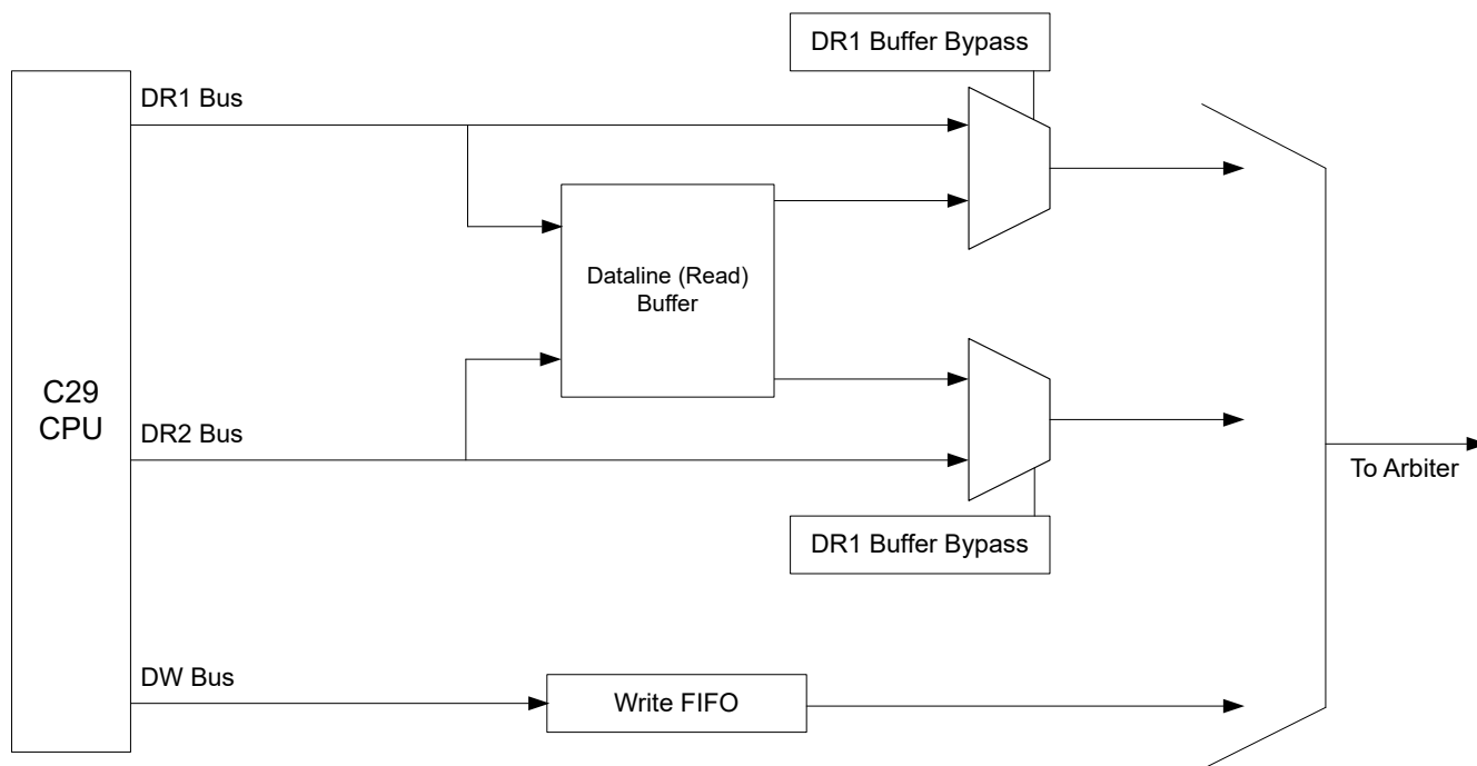
Figure 13-16. Buffer Module Block Diagram
