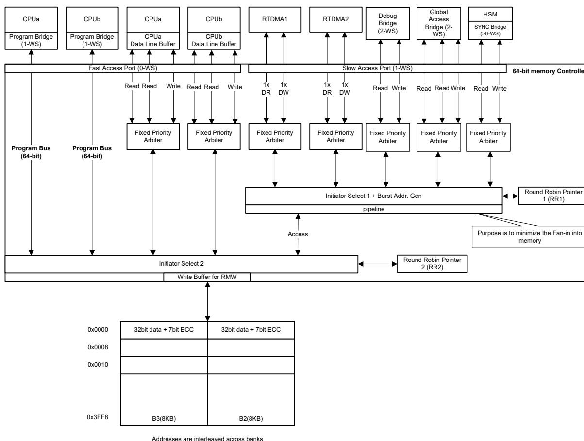
Figure 2-28. Three-Level Arbitration Scheme
