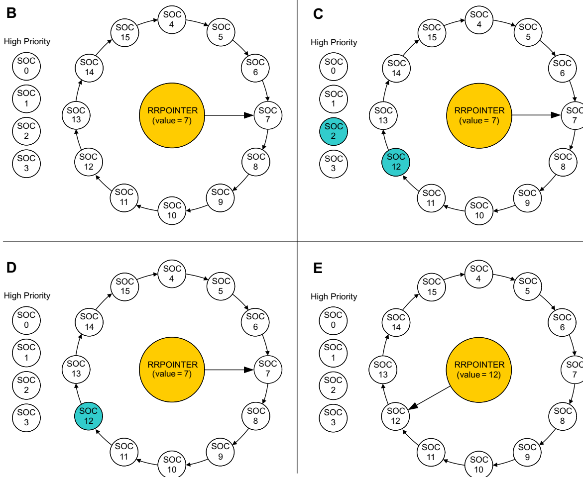
Figure 22-20. High Priority Example
