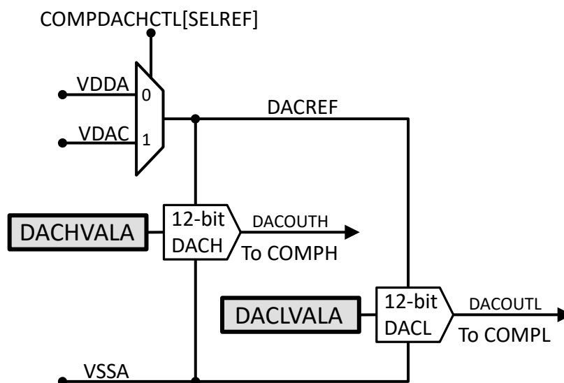
Figure 24-3. Reference DAC Block Diagram
