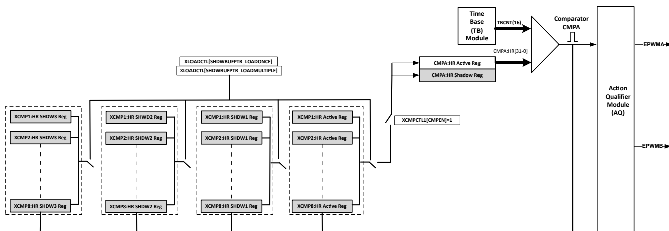
Figure 27-34. Allocate All XCMP1-8 to CMPA
