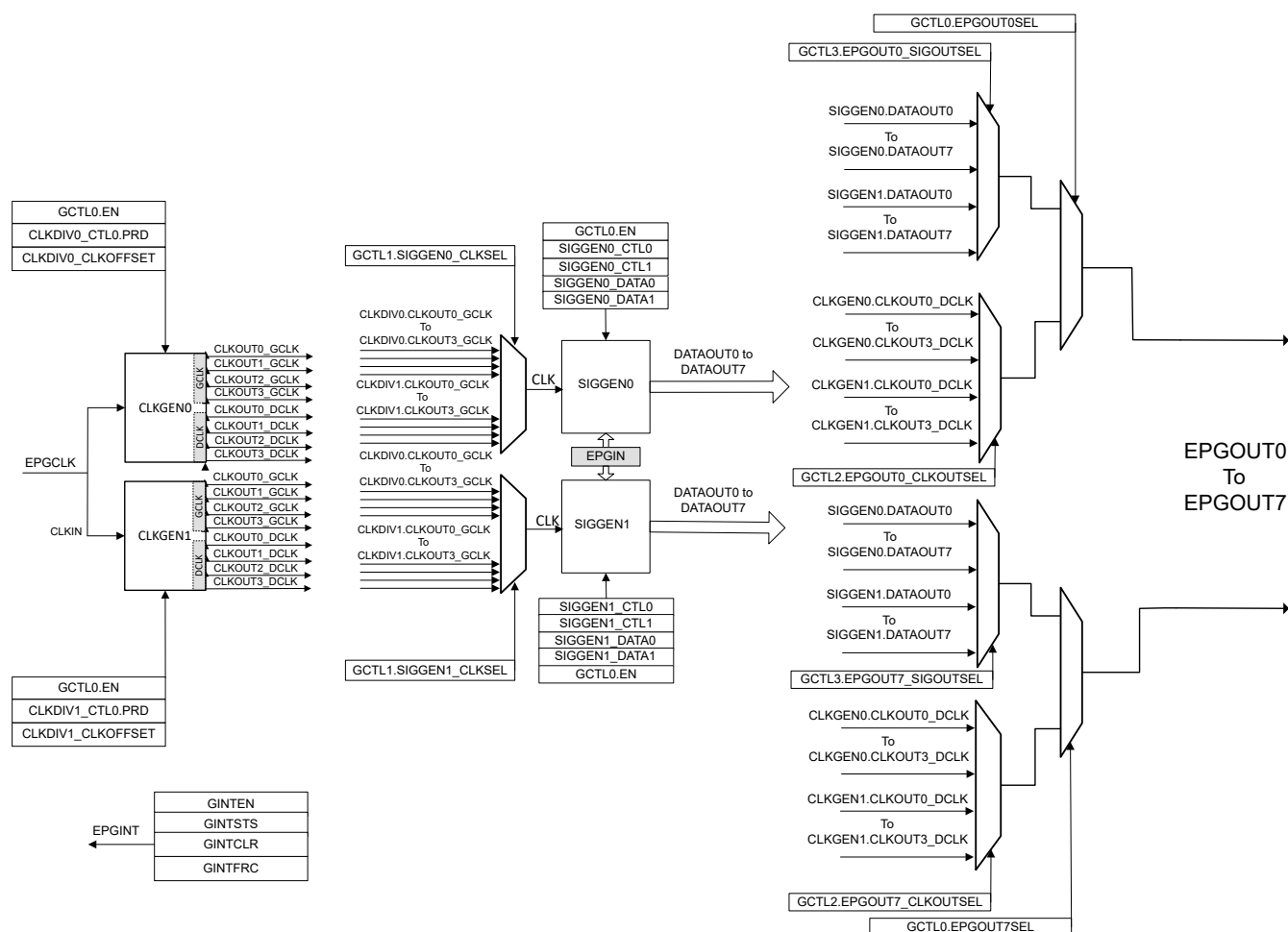
Figure 20-2. EPG Detailed Block Diagram
