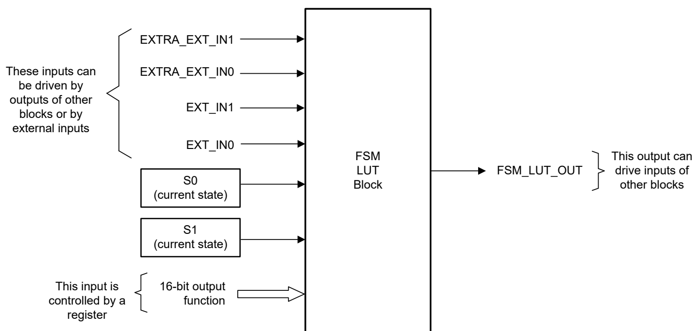
Figure 10-15. FSM LUT Block
