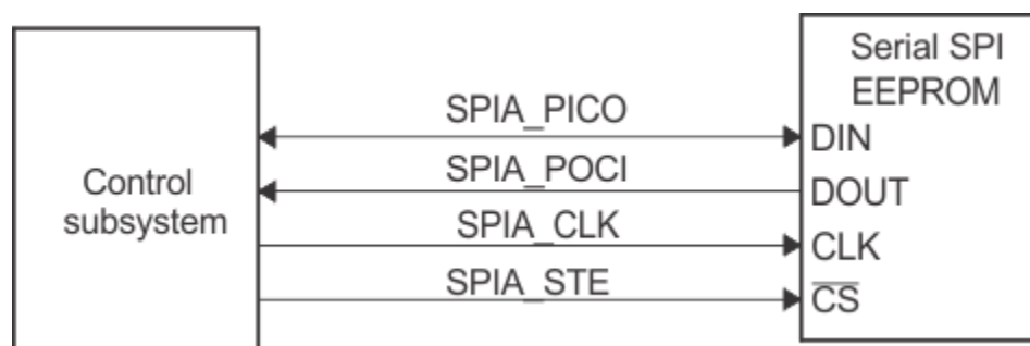
Figure 3-6. Overview of SPI Bootloader Operation
