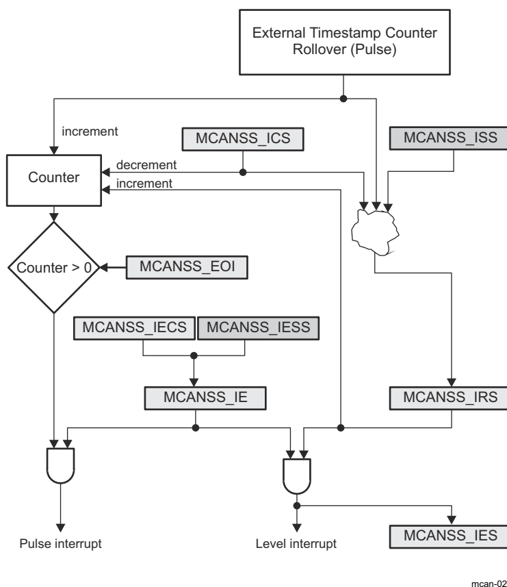
Figure 30-12. External Timestamp Counter Interrupt
