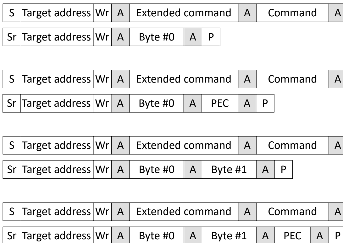
Figure 34-25. Extended Command Write Byte and Write Word Messages With and Without PEC
