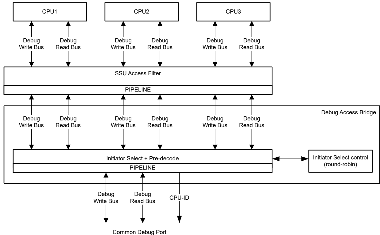
Figure 2-23. Debug Access Bridge
