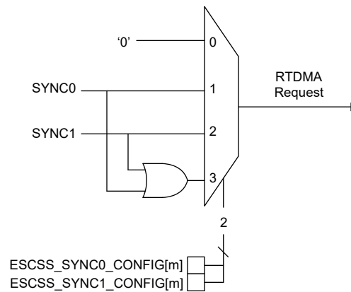
Figure 31-16. SYNC Event Muxing for Different Host RTDMA Triggers
