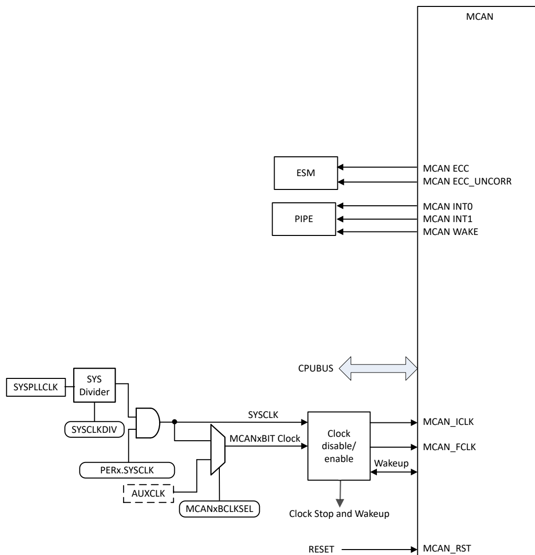
Figure 30-3. MCAN Integration
