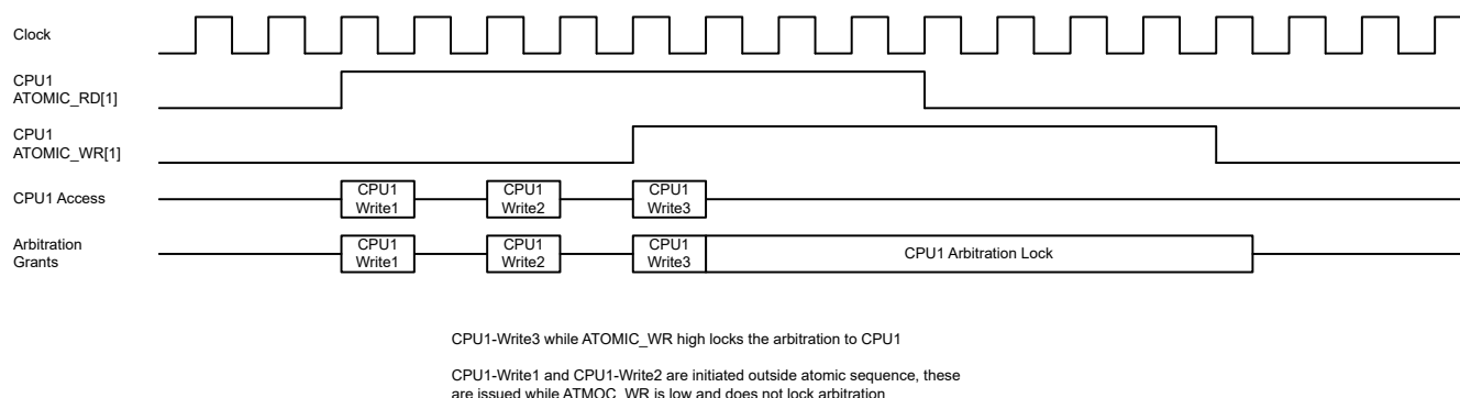
Figure 2-20. Atomic Operations in the MEMSS
