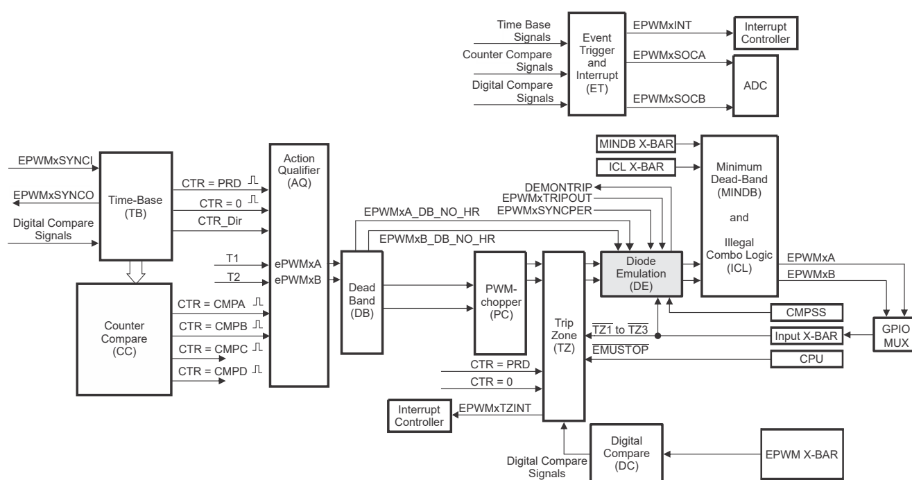
Figure 27-52. Diode Emulation Submodule
