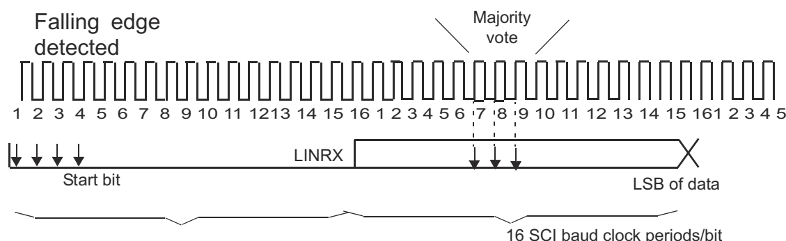
Figure 36-4. Asynchronous Communication Bit Timing
