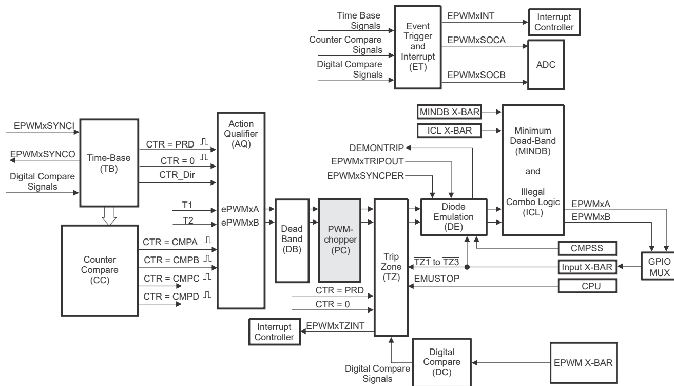
Figure 27-43. PWM Chopper Submodule
