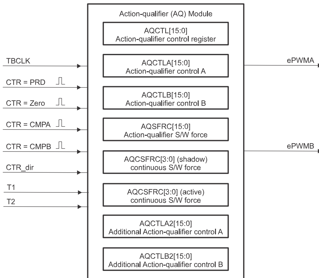
Figure 27-22. Action-Qualifier Submodule Inputs and Outputs
