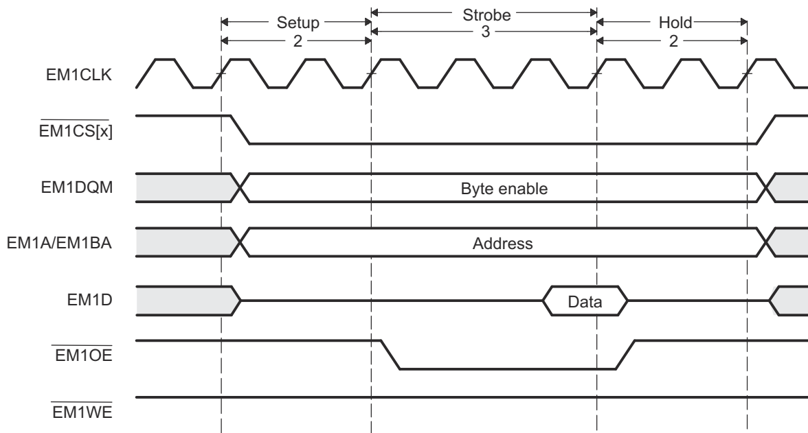
Figure 13-11. Timing Waveform of an Asynchronous Read Cycle in Normal Mode
