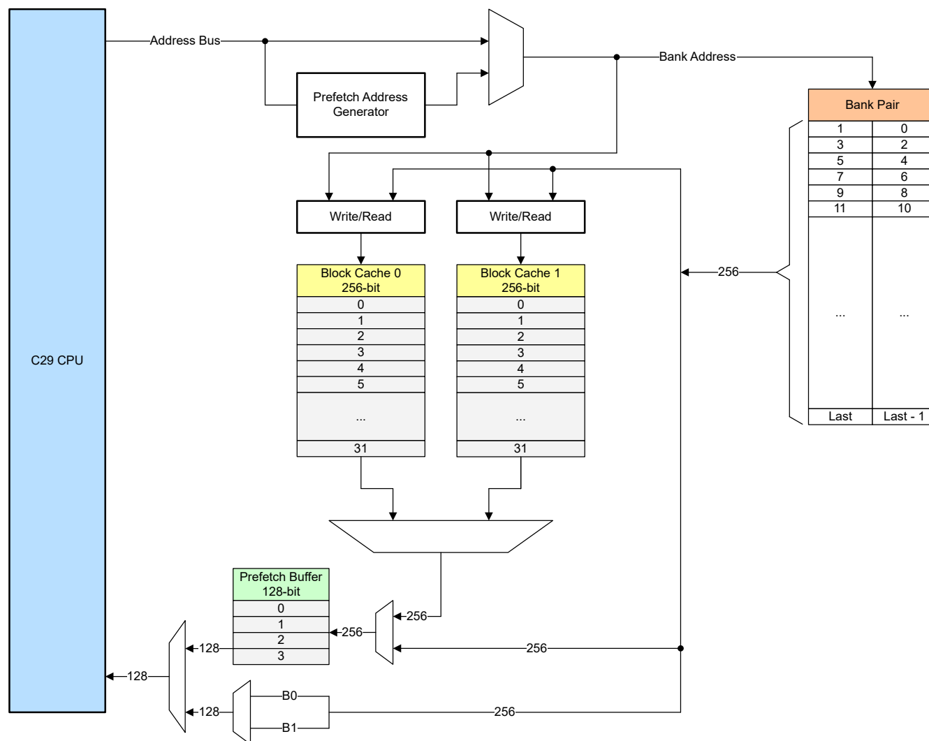
Figure 8-2. Flash Prefetch Mechanism and Block Cache
