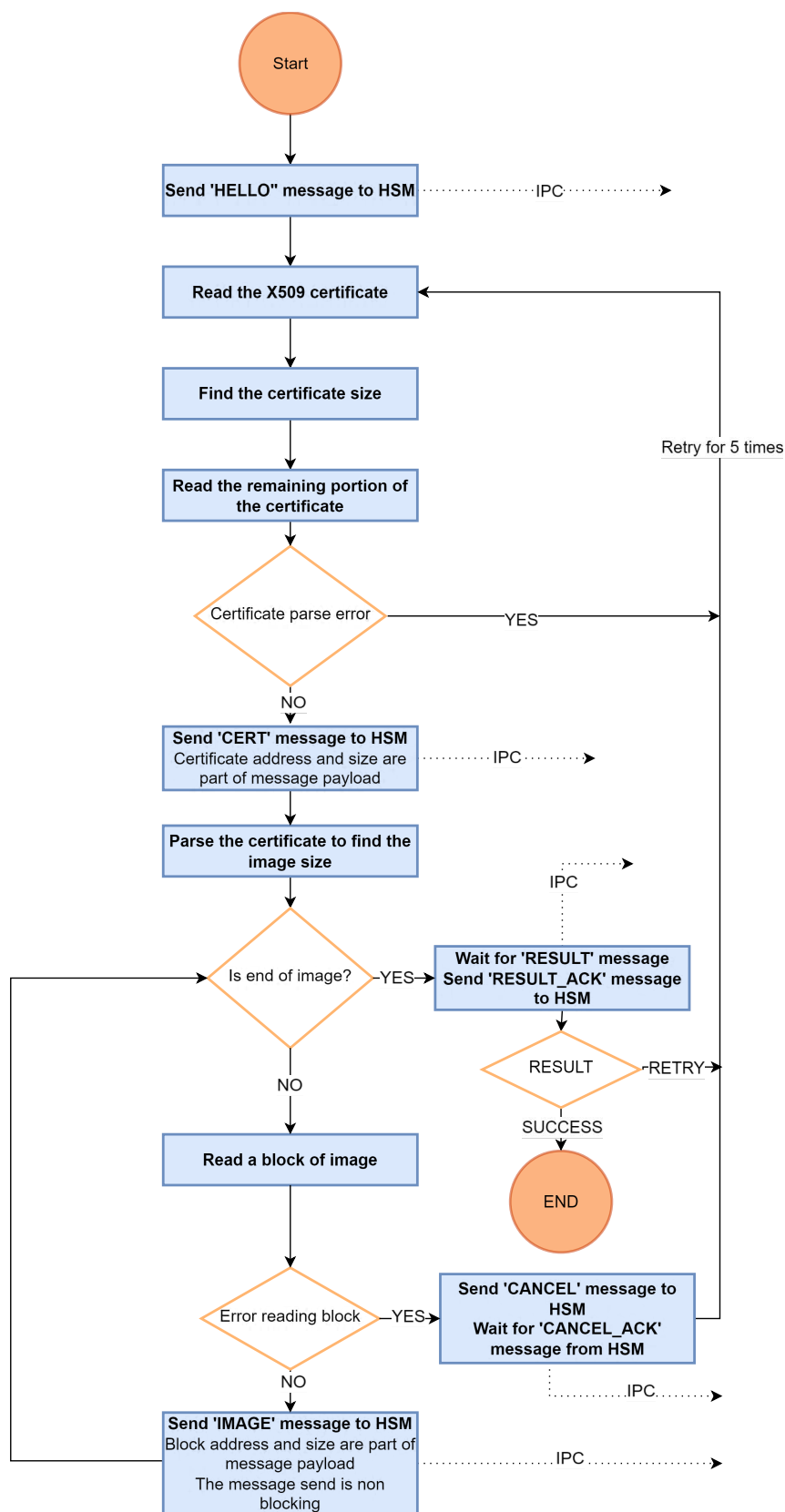
Figure 3-13. Image Authentication by HSM
