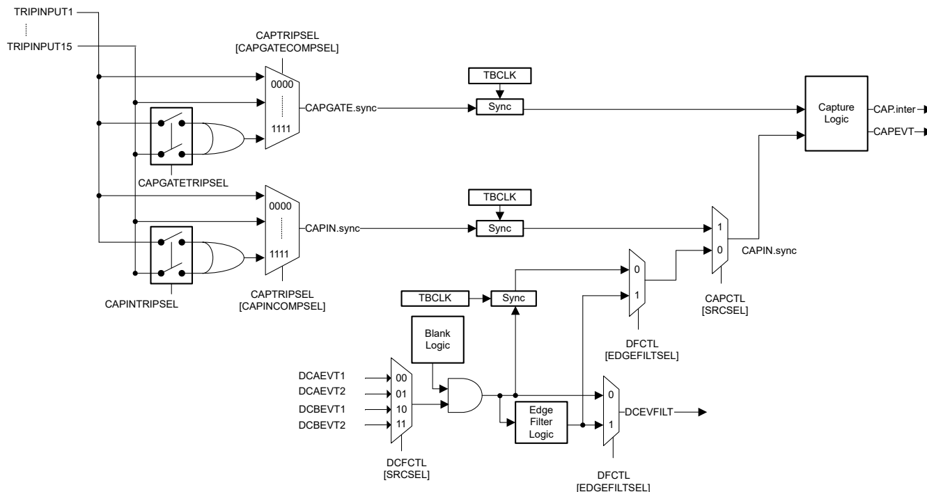
Figure 27-83. CAPIN and CAPGATE Source Selection
