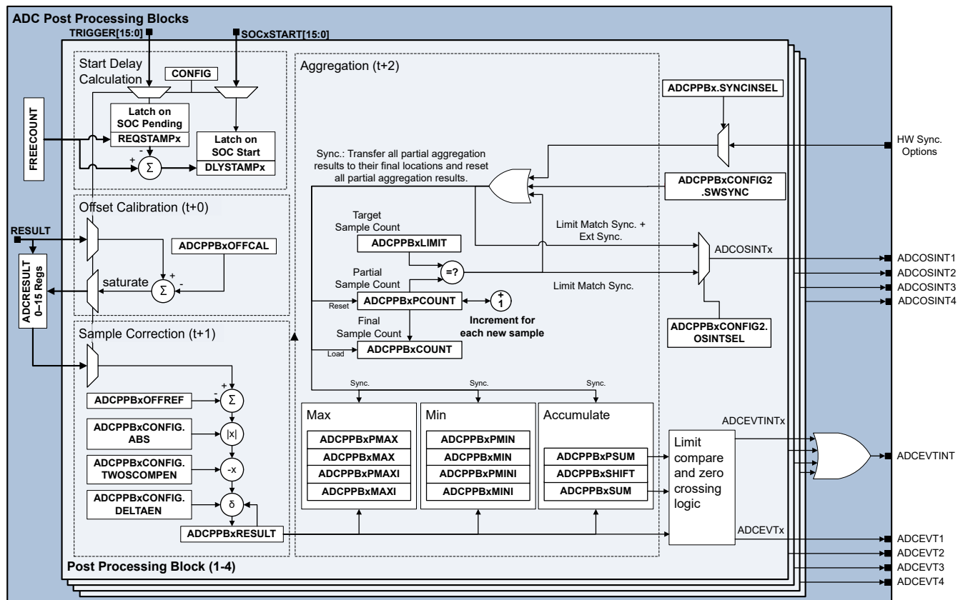
Figure 22-23. ADC Post-Processing Blocks (PPB) Block Diagram
