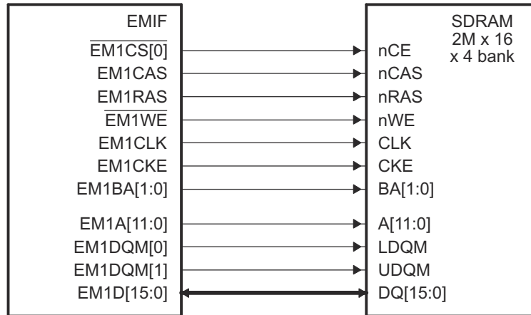
Figure 13-4. EMIF to 2M × 16 × 4 Bank SDRAM Interface
