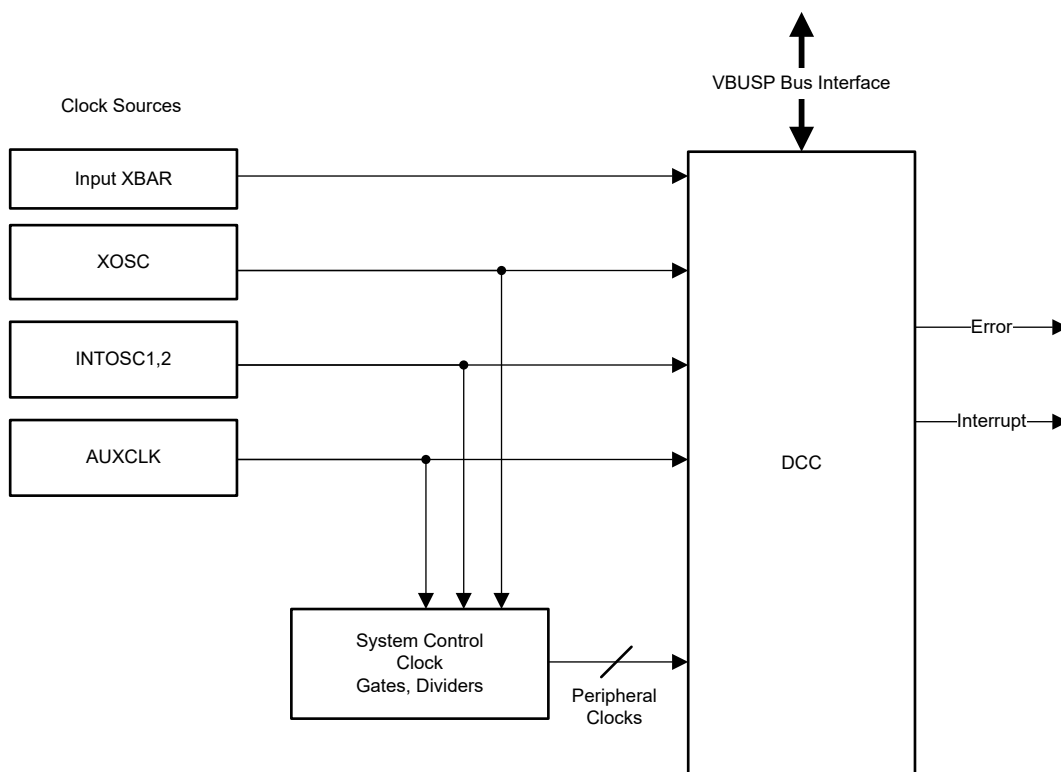
Figure 11-1. DCC Module Overview
