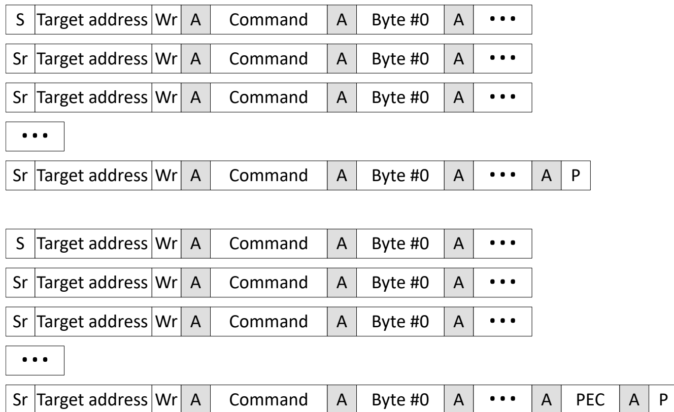
Figure 34-14. Group Command Message With and Without PEC
