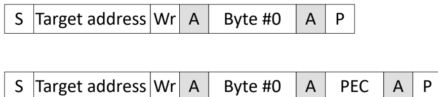
Figure 34-16. Send Byte Message With and Without PEC
