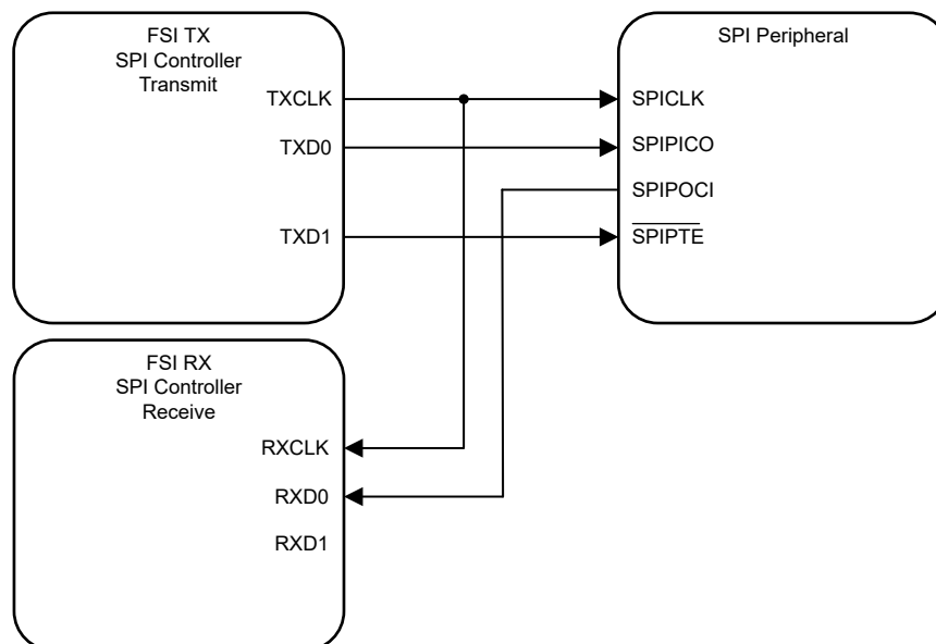
Figure 32-12. FSITX and FSIRX as SPI Controller, Full Duplex
