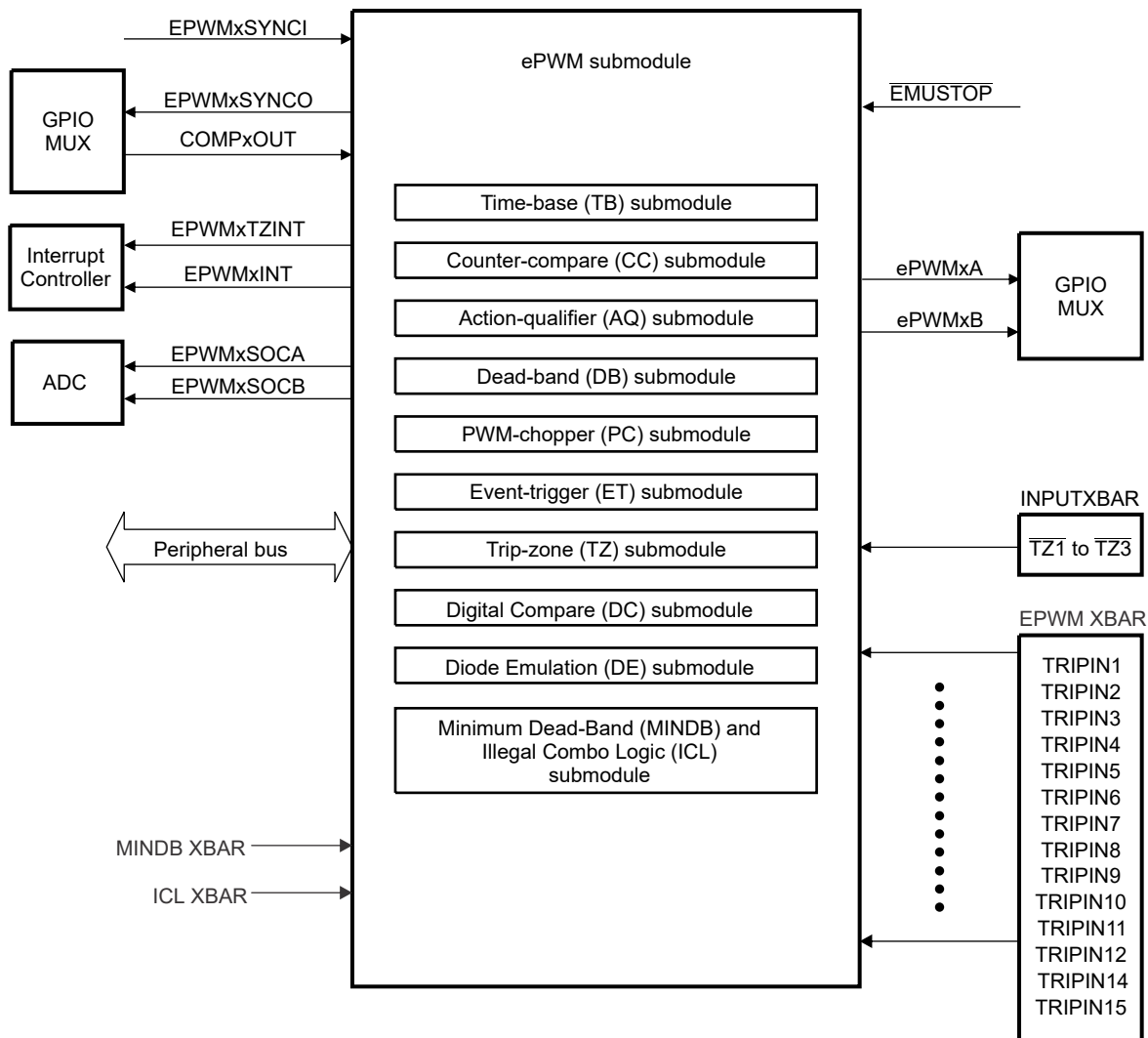
Figure 27-2. Submodules and Signal Connections for an ePWM Module
