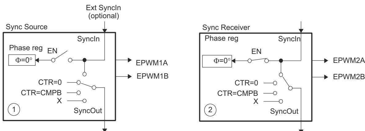
Figure 27-89. EPWM1 Configured as a Typical Sync Source, EPWM2 Configured as a Sync Receiver
