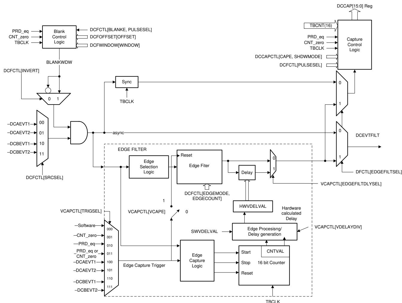
Figure 27-81. Valley Switching
