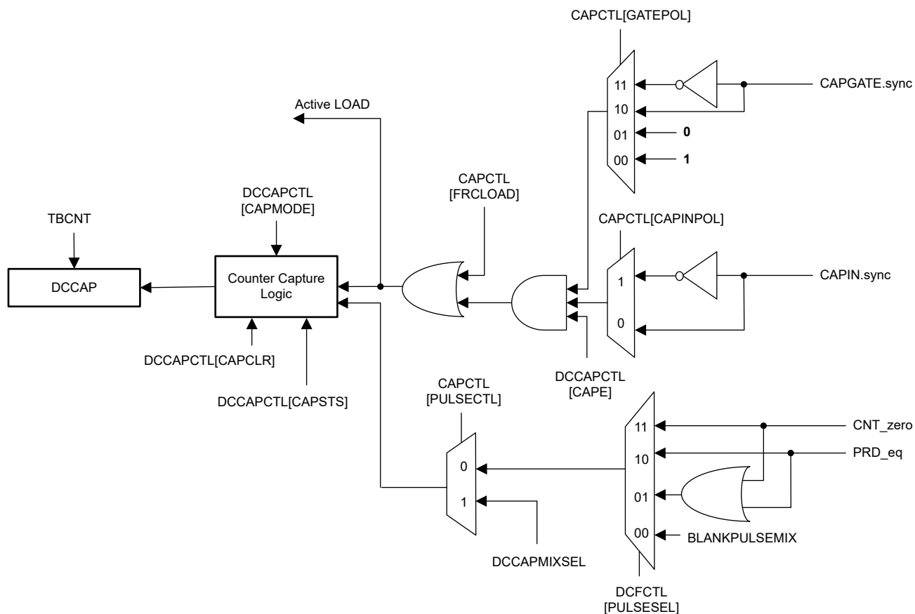
Figure 27-84. Counter Capture Logic
