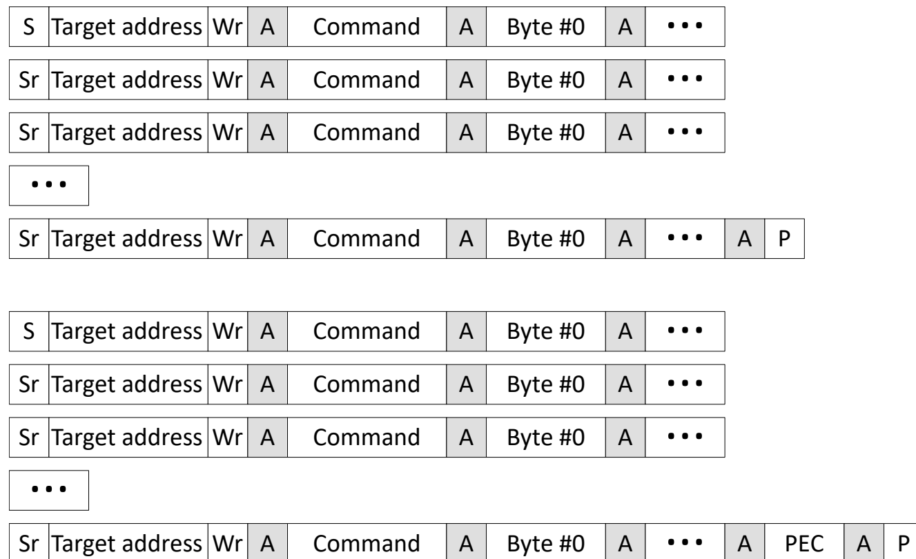
Figure 34-27. Group Command Message With and Without PEC
