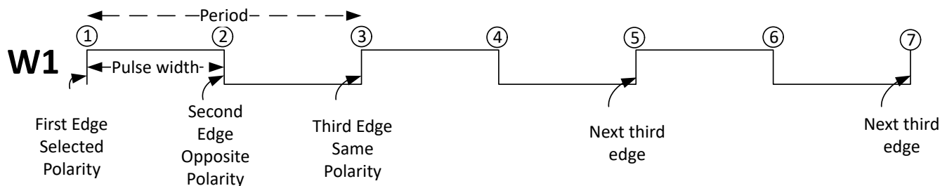
Figure 18-3. Pulse Width Diagram
