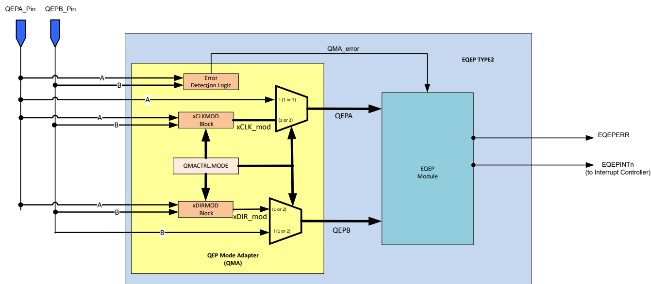
Figure 28-22. QMA Module Block Diagram
