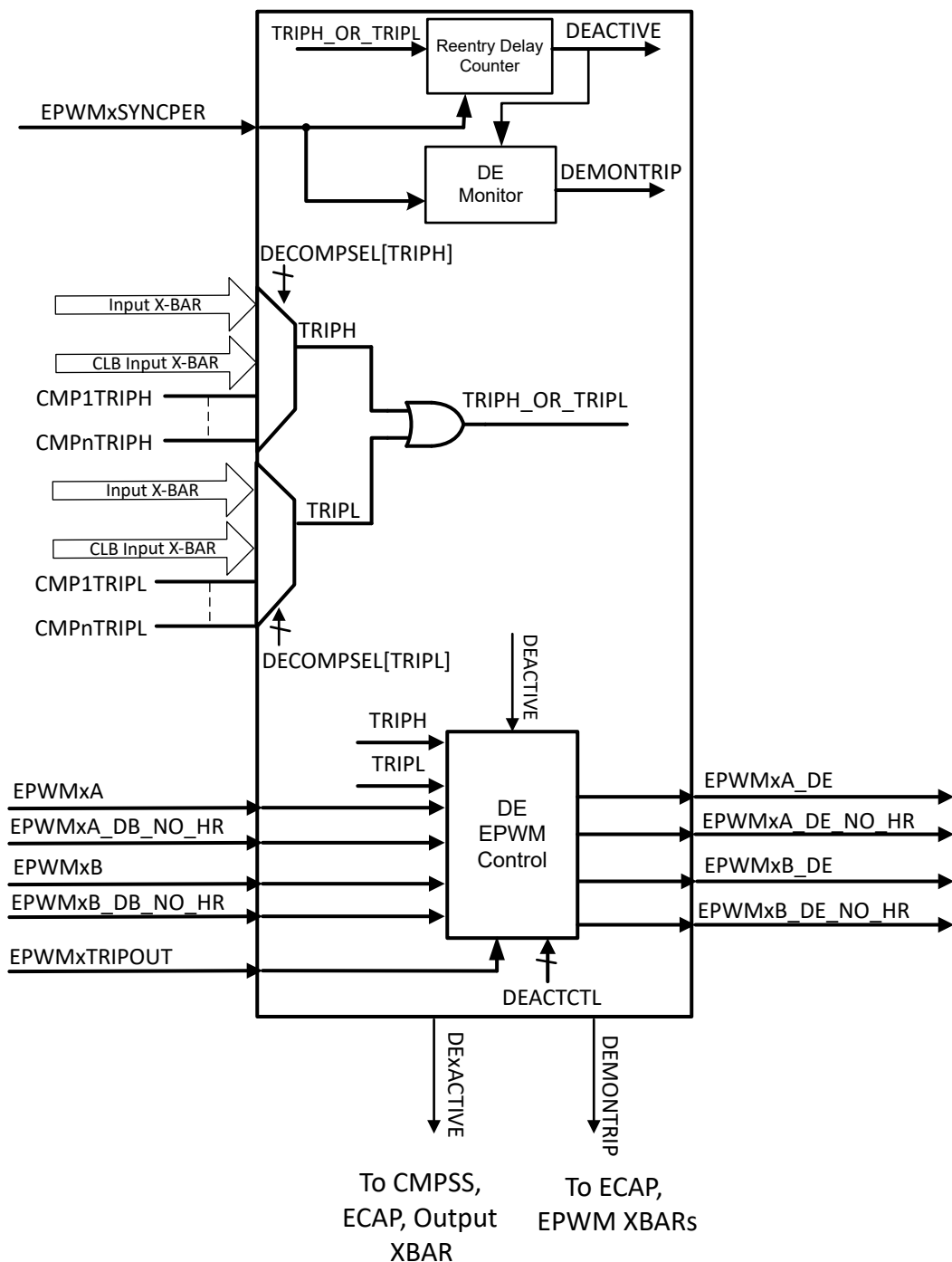
Figure 27-53. Diode Emulation Block Diagram
