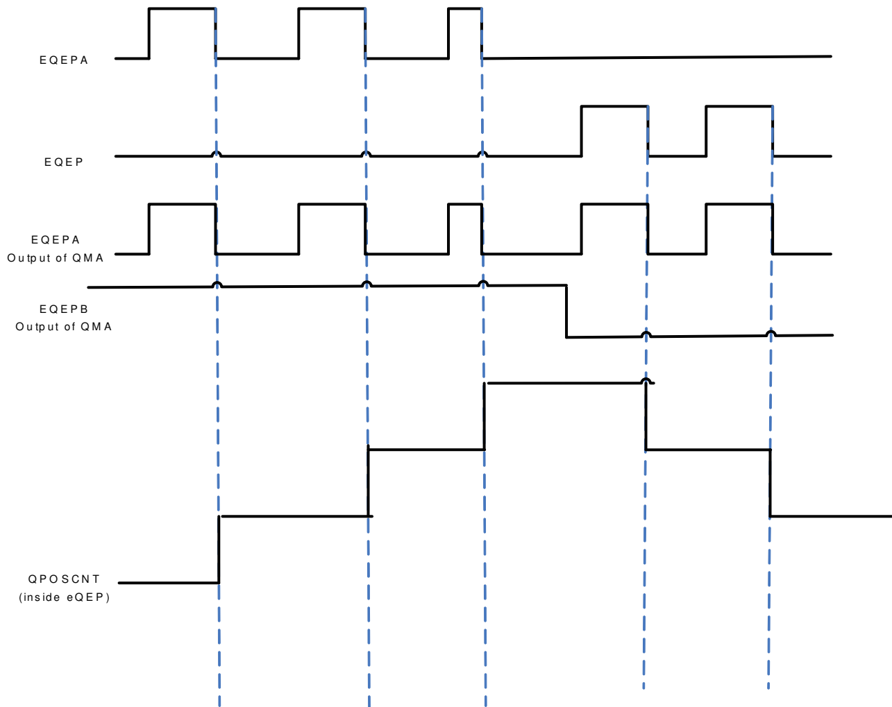
Figure 28-24. QMA Mode-2
