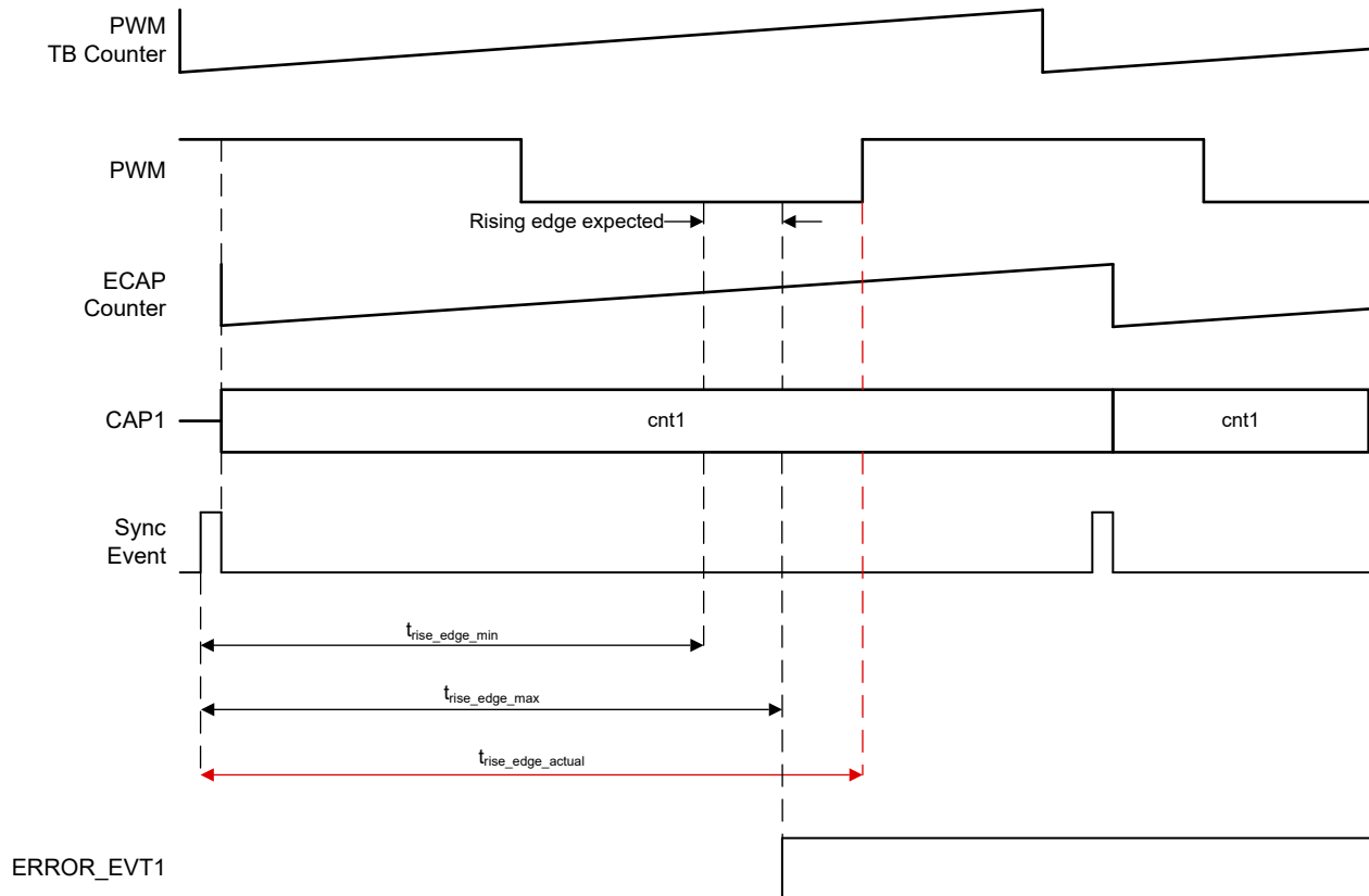
Figure 25-13. ECAP Signal Monitoring Unit Edge Error Example
