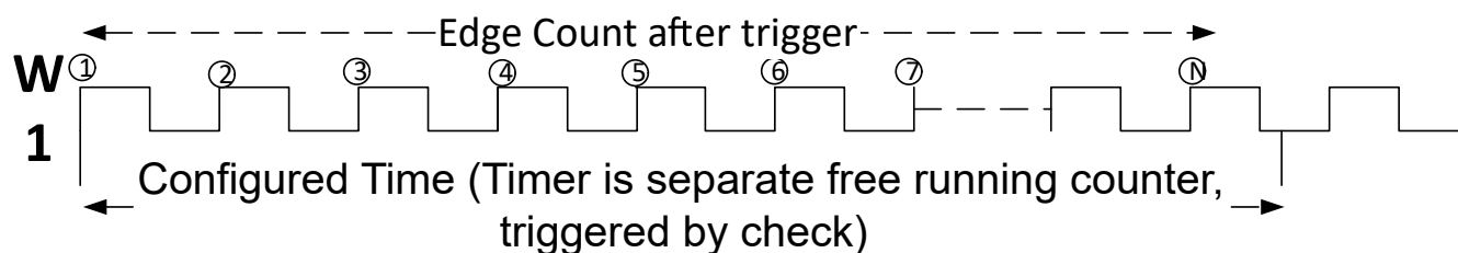
Figure 18-4. Edge Count Diagram
