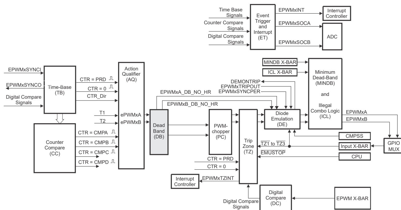
Figure 27-40. Dead_Band Submodule
