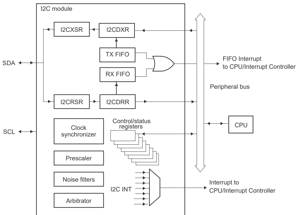
Figure 33-2. I2C Module Conceptual Block Diagram
