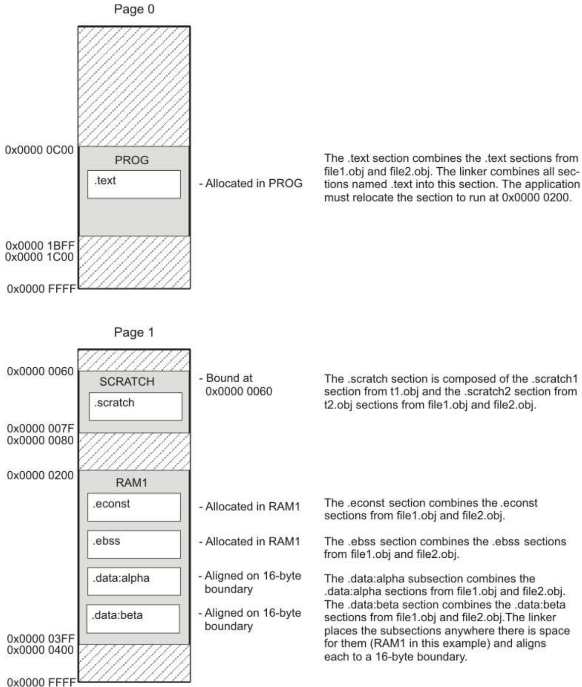
Figure 8-3. Section Placement Defined by the SECTIONS Directive Example
