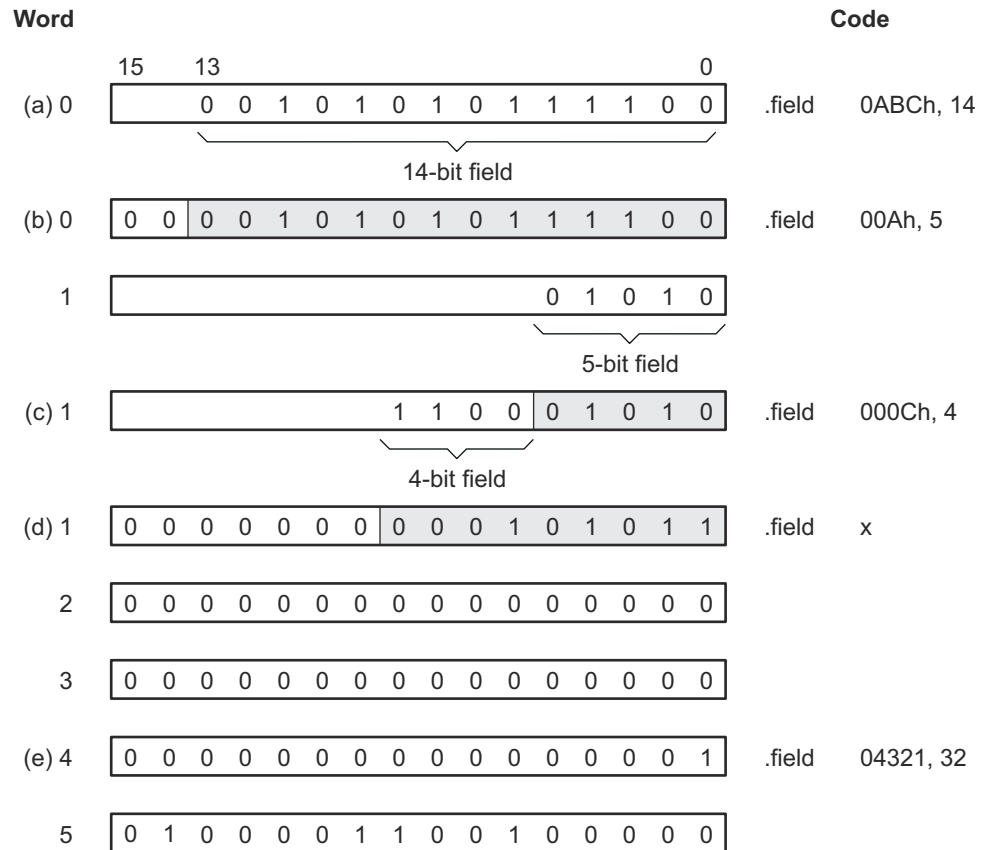
Figure 5-5. The .field Directive
