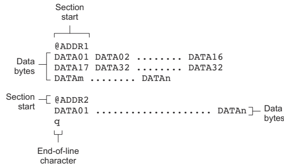
Figure 12-14. TI-TXT Object Format
