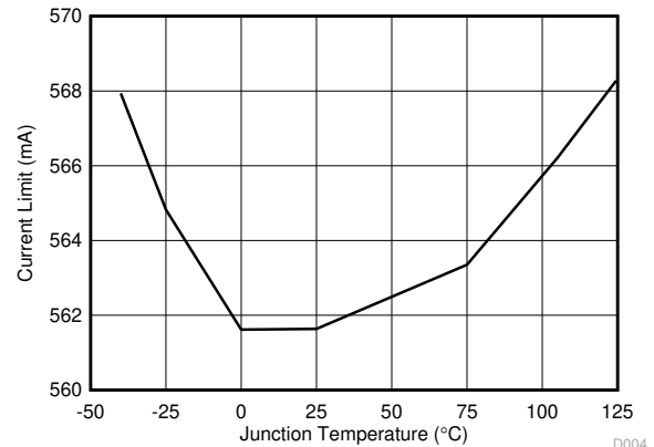
图 6-2. PoE Current Limit vs Temperature
