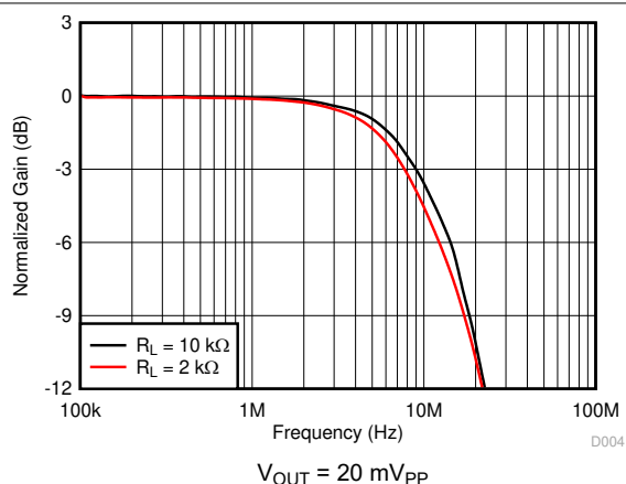
图 7-6. Small-Signal Frequency Response vs Output Load
