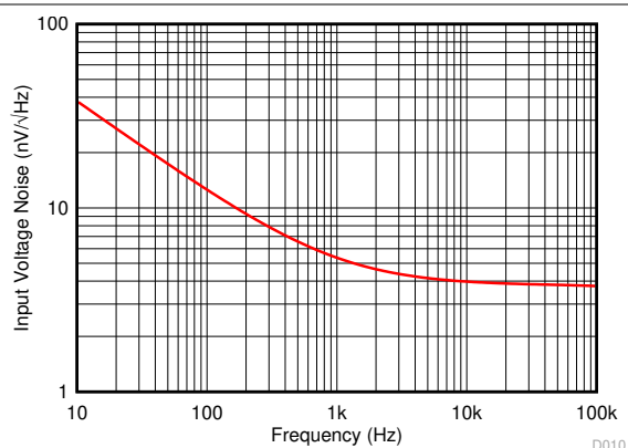
图 7-2. Input Voltage Noise Density vs Frequency
