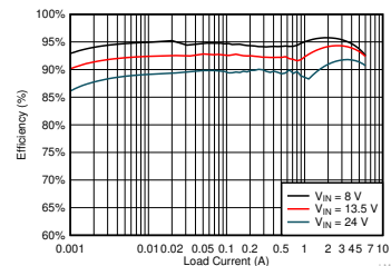
效率：，V OUT = 5V，F sw = 2.1 MHz
