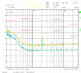
传导 EMI：V OUT = 5V，I OUT = 4A
