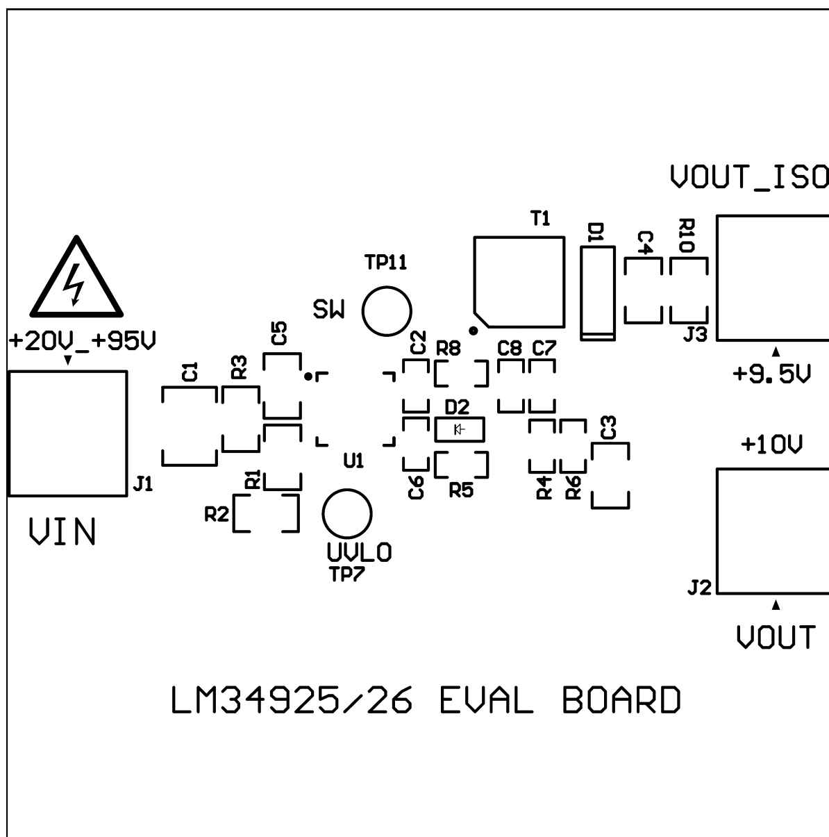
Figure 5. Board Silkscreen
