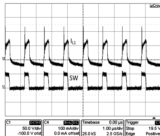
Figure 4. Steady State Waveform (VIN=48V, IOUT1=0mA, IOUT2= 100mA)
