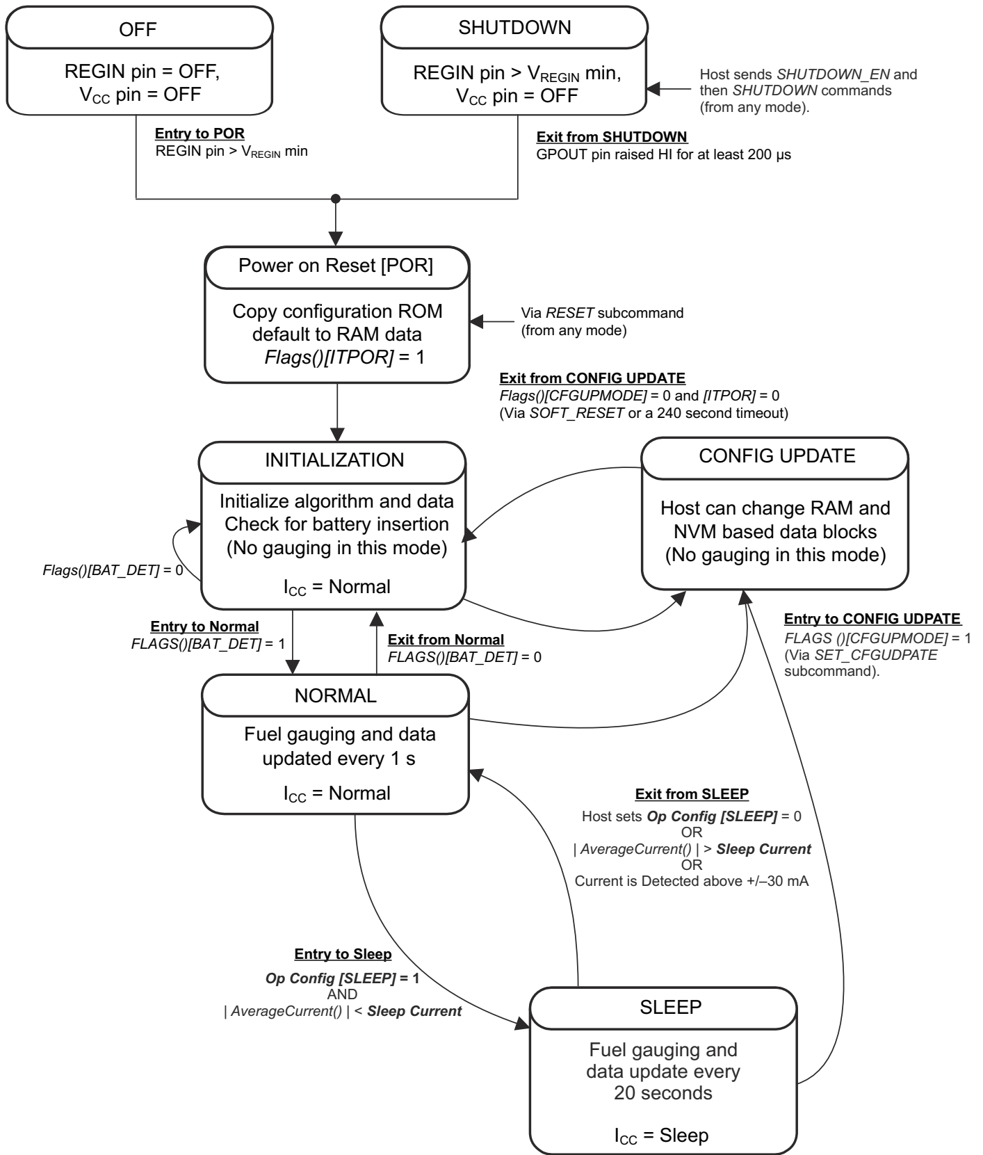
Figure 2-1. Power Mode Diagram
