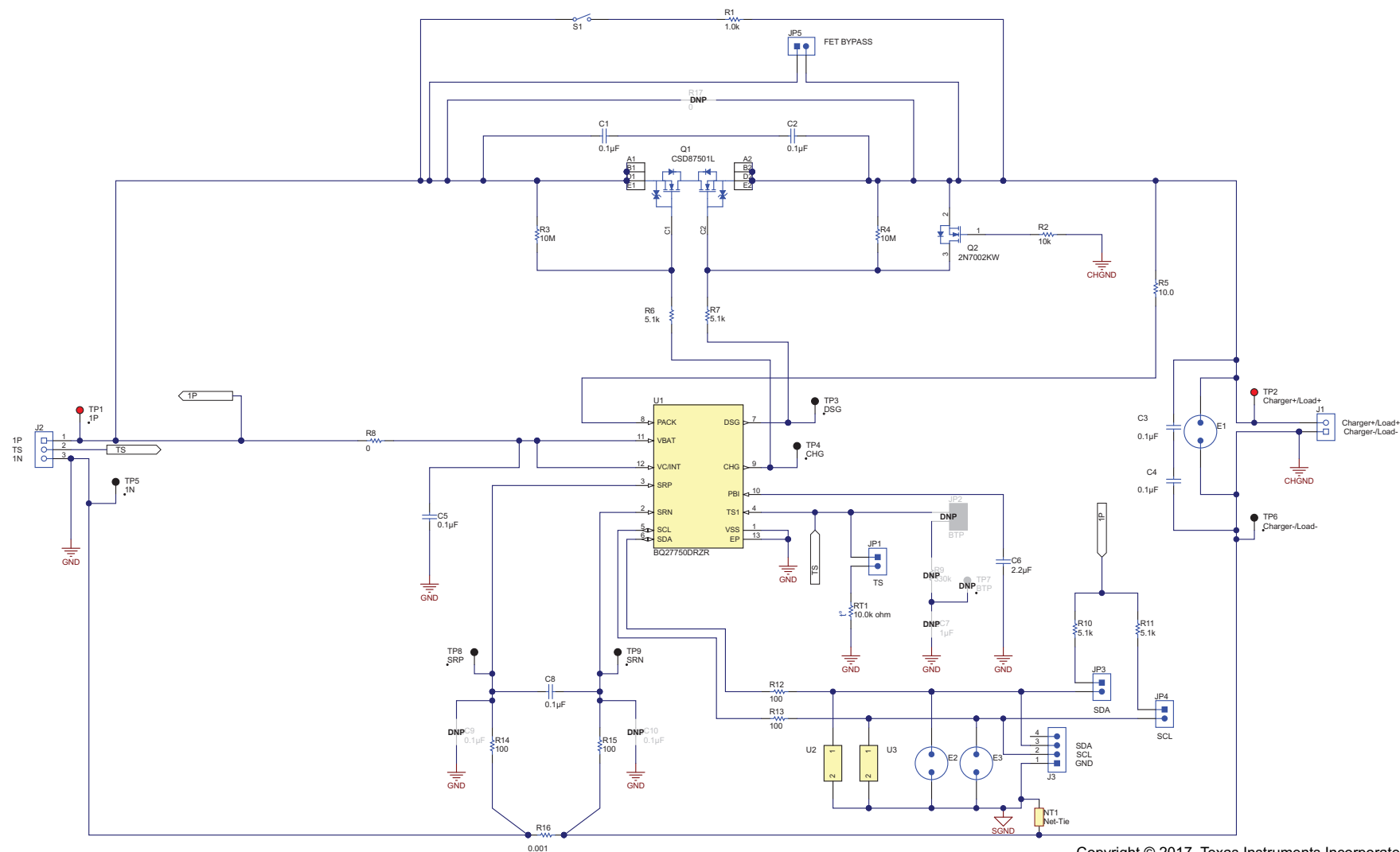
Figure 21. Schematic
