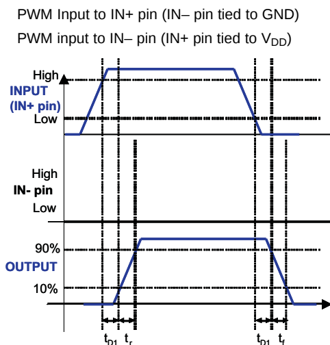
Figure 1. Non-Inverting Configuration
