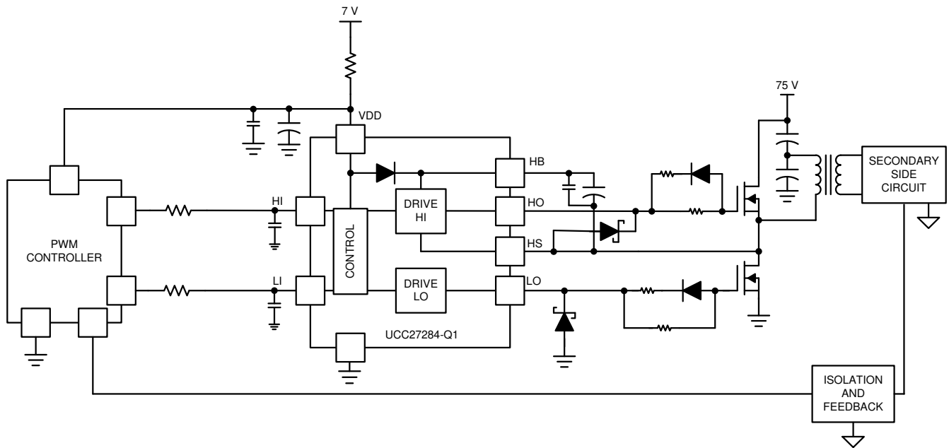
Figure 8-1. Typical Application
