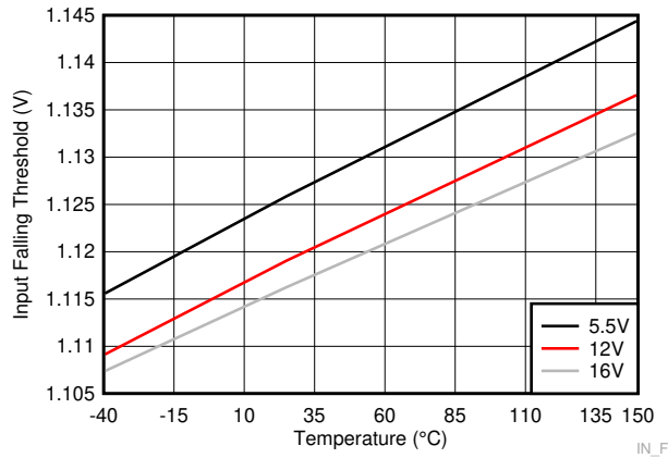
Figure 6-7. Input Falling Threshold
