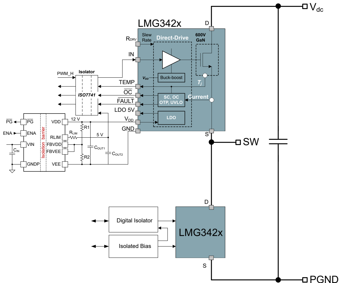
Figure 12-12. Dual-Output (Two Positive) System Configuration
