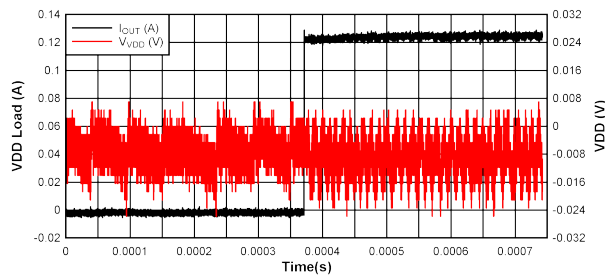
Figure 10-6. Load Transient Response: No Load to 1 W, VIN = 12 V, V VDD-VEE = 12 V, V COM-VEE = 5 V
