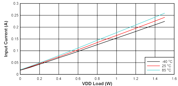
Figure 10-21. Input Current vs Load on V_{VDD-VEE} : V_{IN} = 15\text{ V} , V_{VDD-VEE} = 12\text{ V} , V_{COM-VEE} = 5\text{ V} , No Load on V_{COM-VEE}
