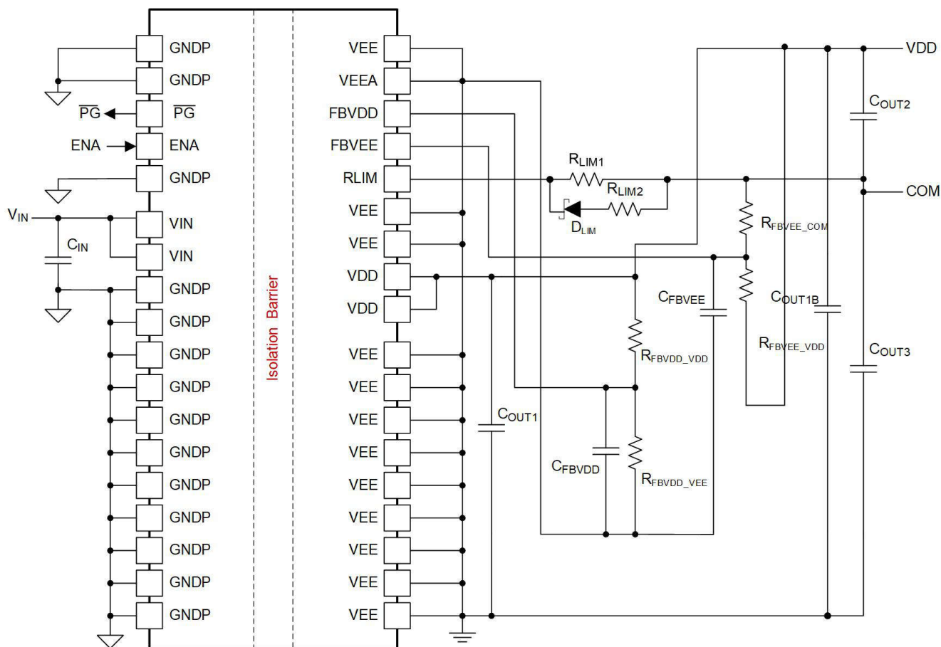
Figure 12-10. Dual output application schematic configured for V_{COM\_VEE} regulation < 2.5V
