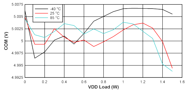
Figure 10-13. V COM-VEE Load Regulation: VIN = 15 V, V VDD-VEE = 12 V, V COM-VEE = 5 V
