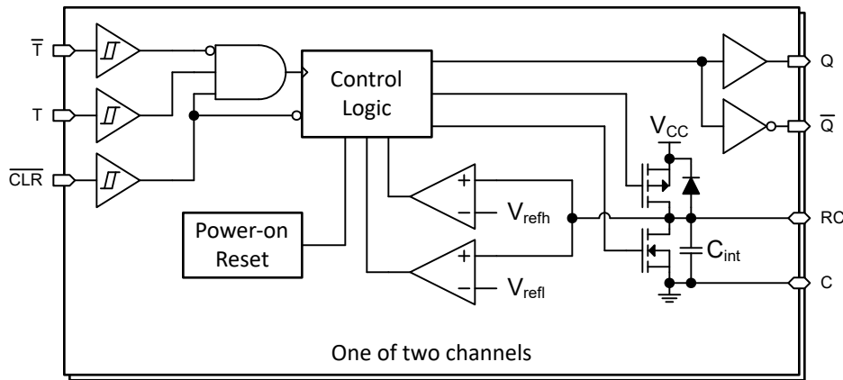
Figure 7-3. TPUL2T122-Q1
