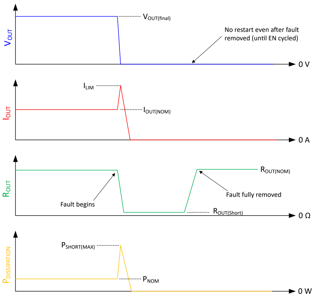
Figure 8-6. Simplified Turn-Off Current Limit Waveforms (CLM Low)
