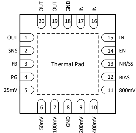
Figure 5-2. RGR Package (TPS7A8401A), 20-Pin VQFN, Top View
