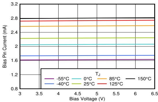
Figure 6-79. Bias Pin Current With Bias
