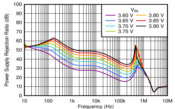
I_{OUT} = 3\text{ A} , C_{OUT} = 47\text{ }\mu\text{F} \parallel 10\text{ }\mu\text{F} \parallel 10\text{ }\mu\text{F} , C_{NR/SS} = 10\text{ nF} , C_{FF} = 10\text{ nF}
