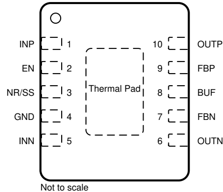
Figure 4-1. DSC Package, 10-Pin WSON (Top View)
