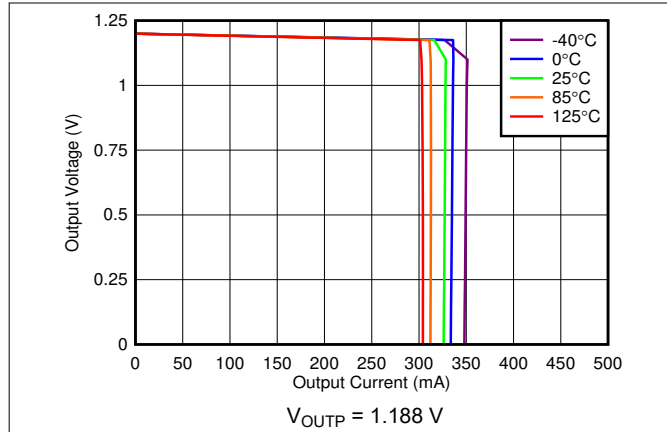
Figure 5-46. Positive Regulator Current Limit
