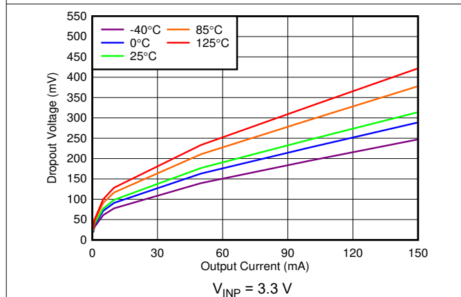
Figure 5-50. Positive Regulator Dropout Voltage vs Output Current
