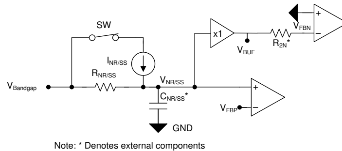
Figure 6-3. Simplified Reference Circuit
