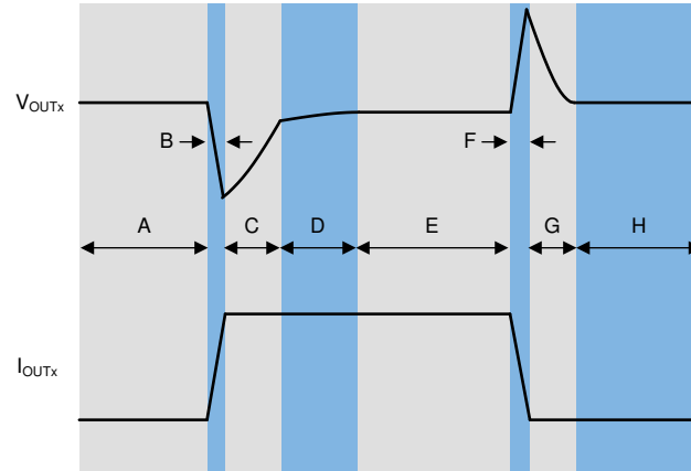
Figure 7-5. Load Transient Waveform
