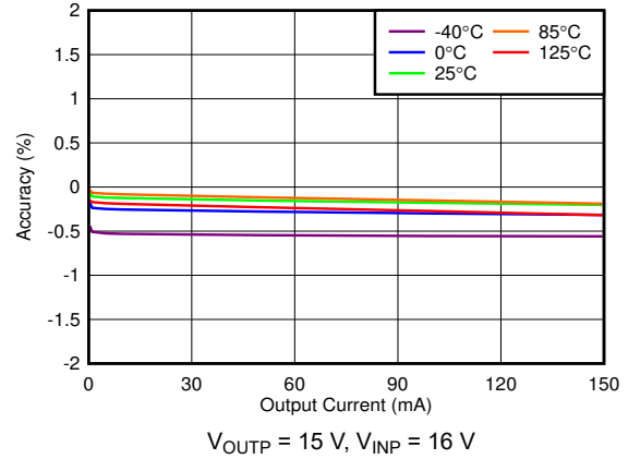
Figure 5-41. Positive Load Regulation
