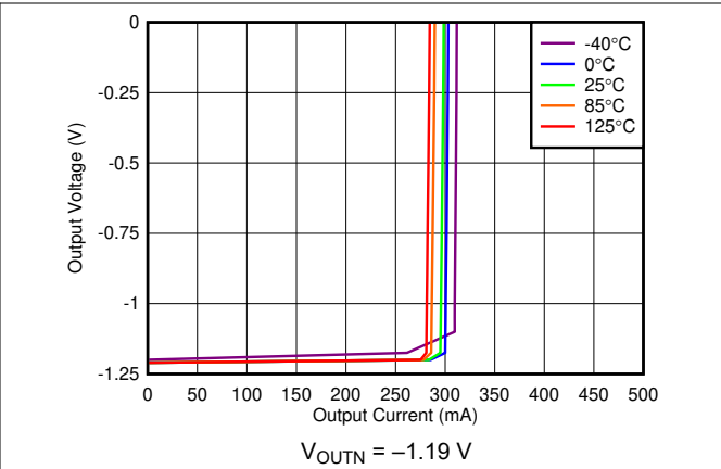
Figure 5-47. Negative Regulator Current Limit
