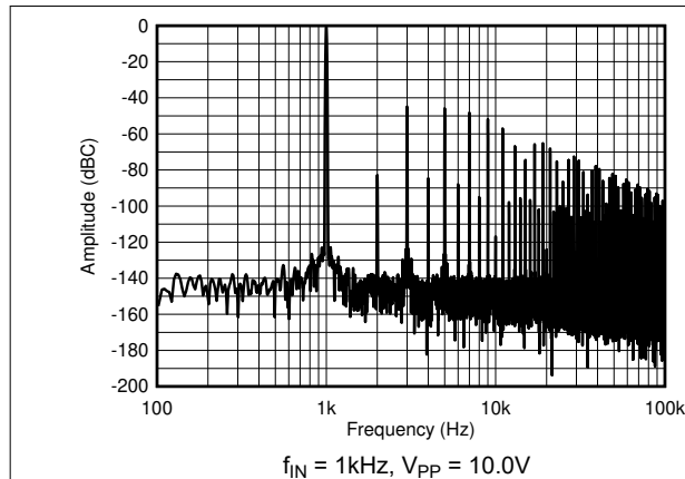
Figure 7-15. FFT Using 5V and 0V Supply Rails
