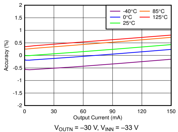
Figure 5-39. Negative Load Regulation
