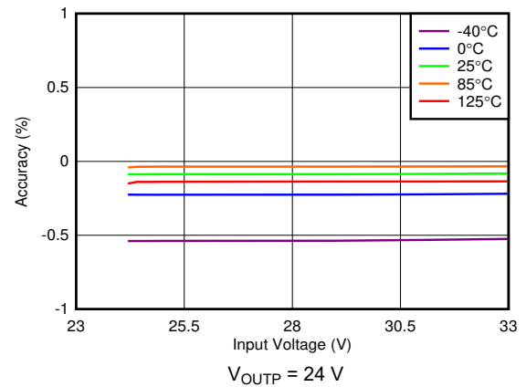
Figure 5-45. Positive Line Regulation
