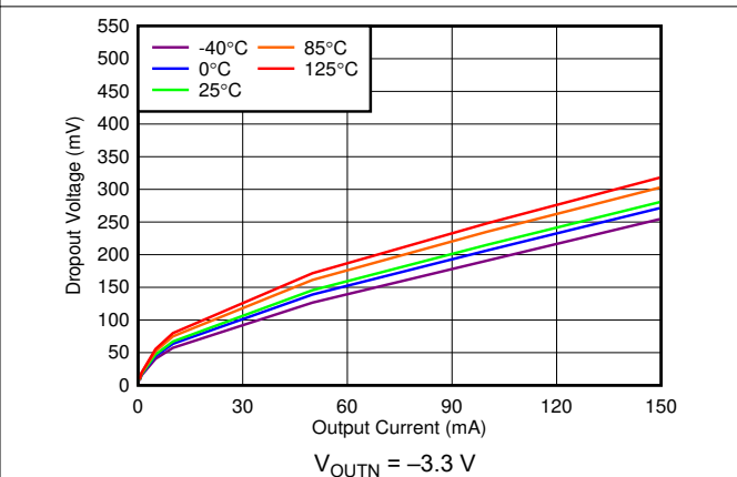
Figure 5-51. Negative Regulator Dropout Voltage vs Output Current
