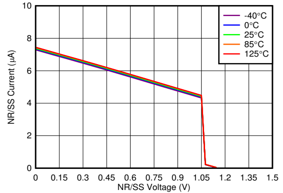
Figure 5-53. I_{NR/SS} vs V_{NR/SS}
