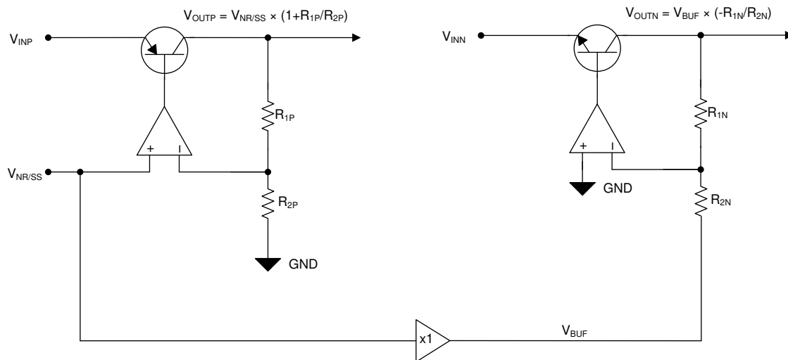
Figure 6-5. Simplified Regulation Circuit
