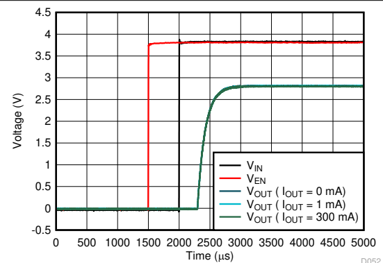
Figure 5-76. Start-Up
