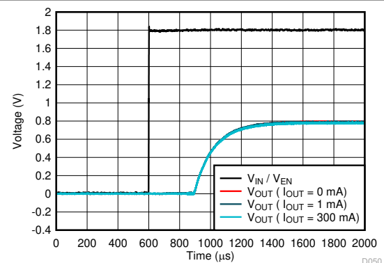
Figure 5-74. Start-Up
