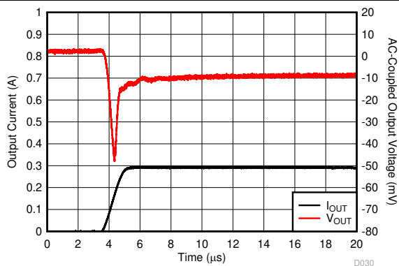
Figure 5-51. Load Transient
